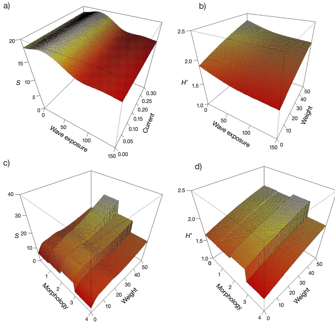
Fig. 1. Response plots of the averaged mixed generalized additive models for number of faunal species S by (a) wave exposure and current speed and by (c) epiphyte amount (weight, g) for each morphology of the epiphyte (1 = bushy, 2 = leaf, 3 = rough, 4 = smooth), and for the Shannon-Wiener diversity index H' by (b) wave exposure and epiphyte amount (weight, g) and (d) morphology and epiphyte amount (weight, g)
