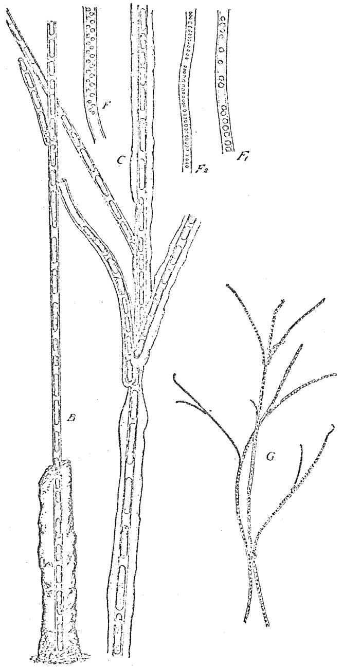
Abb. 36: Clonothrix fusca .
