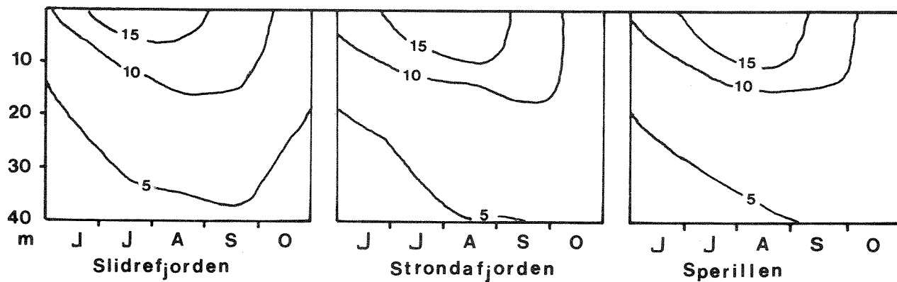
Fig.I temperaturdiagram for 1984
