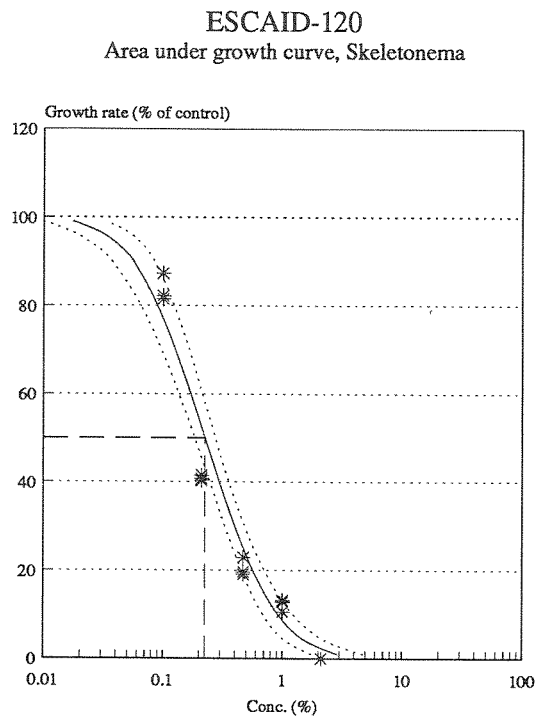
Fig. 3. Effect of ESCAID 120 on area under growth curves for Skeletonema
