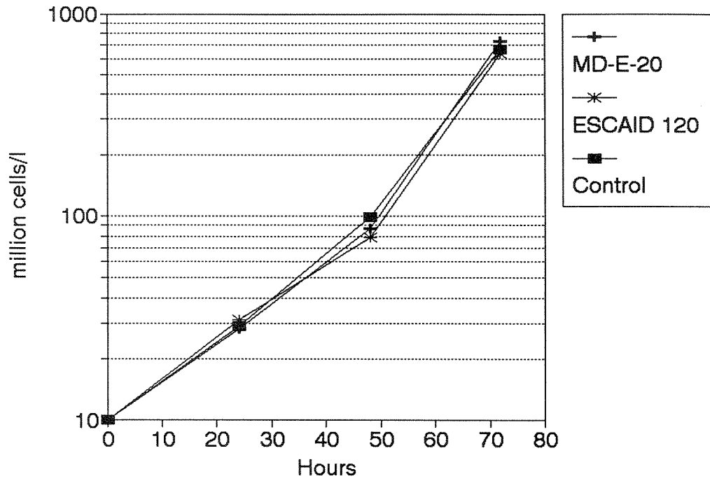
Fig. 1. Growth curves of Selenastrum capricornutum with the degraded samples of ESCAID 120 and MD-E-20 and in control cultures.
