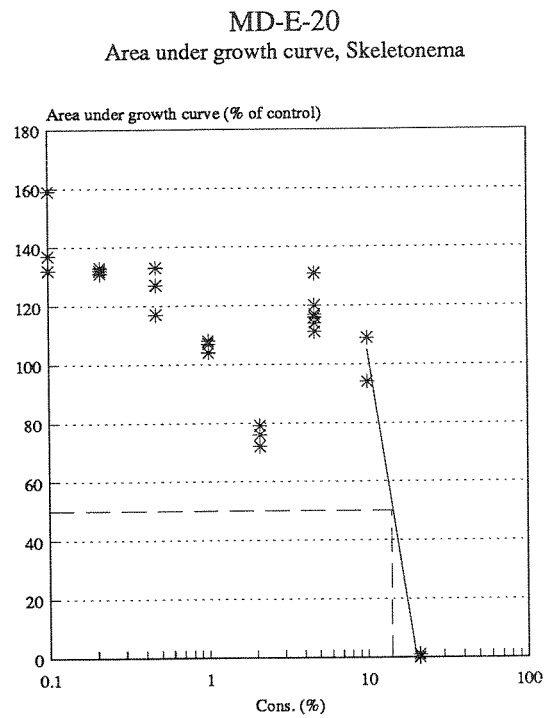
Fig. 3. Effect of MD-E-20 on area under growth curves for Skeletonema costatum . (Test 1 and 2)
