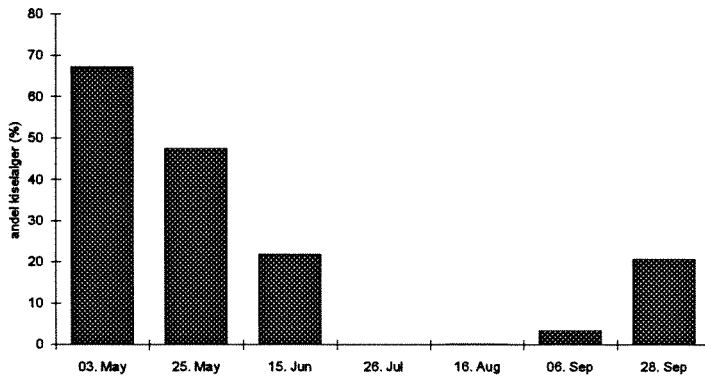
Figur 3.10 Andel kiselalger 1993
