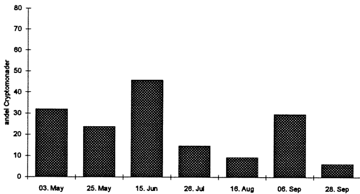
Figur 3.12 Andel cryptomonader 1993
