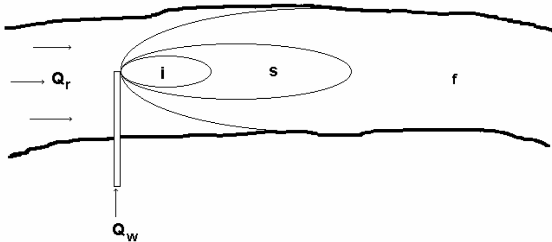
Fig. 3. Schematic view of dilution of wastewater in a river. i = initial dilution zone, s = secondary dilution zone and f = final dilution zone.
