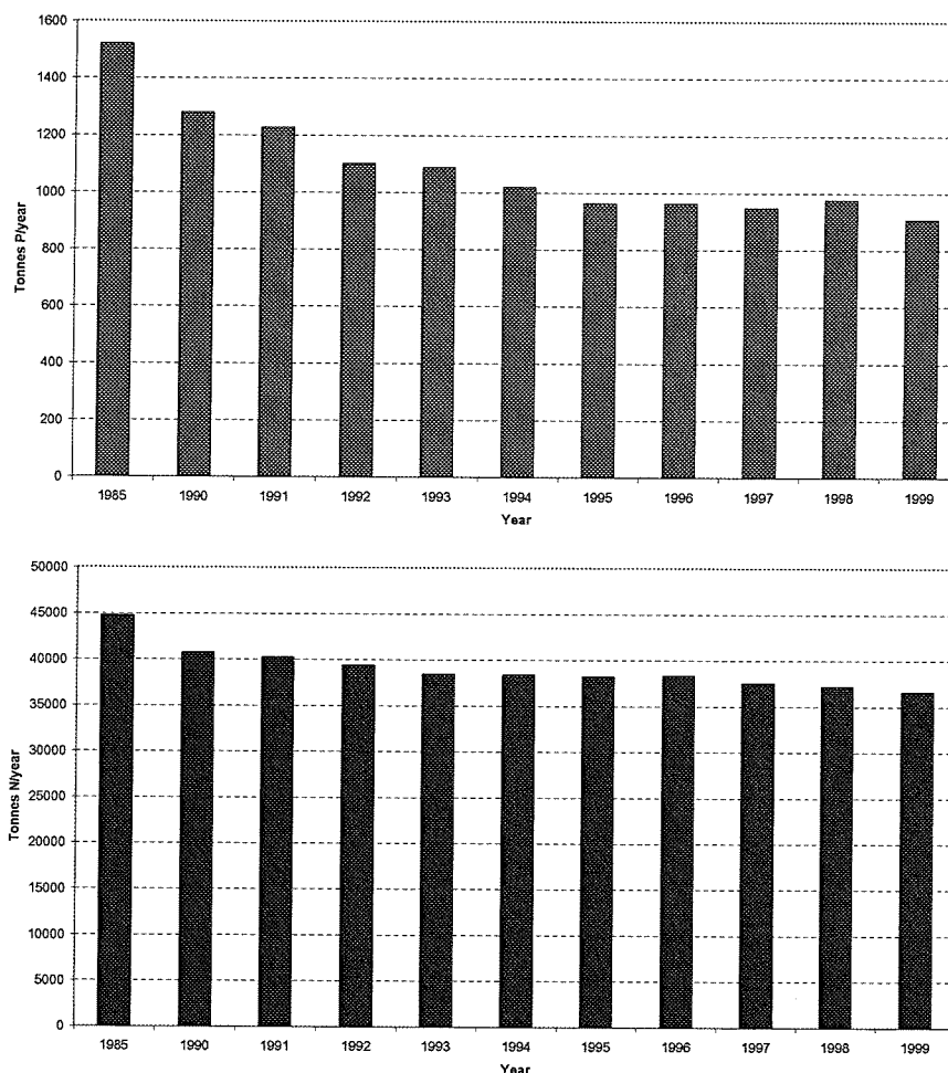
Figure 6. Total input of phosphorus (upper figure) and nitrogen (lower figure) from landbased sources between the Swedish border and Lindesnes (after Borgvang and Tjomsland 2001).
