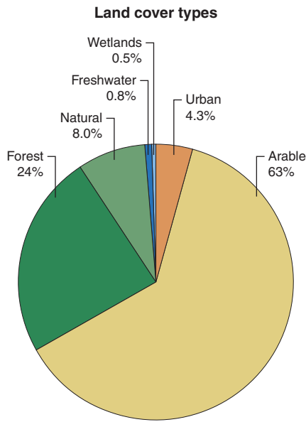
Figure 2: Main land use classes in the River Kapos catchment.
