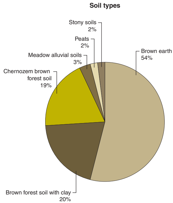
Figure 3: Main soil types in the River Kapos catchment.
