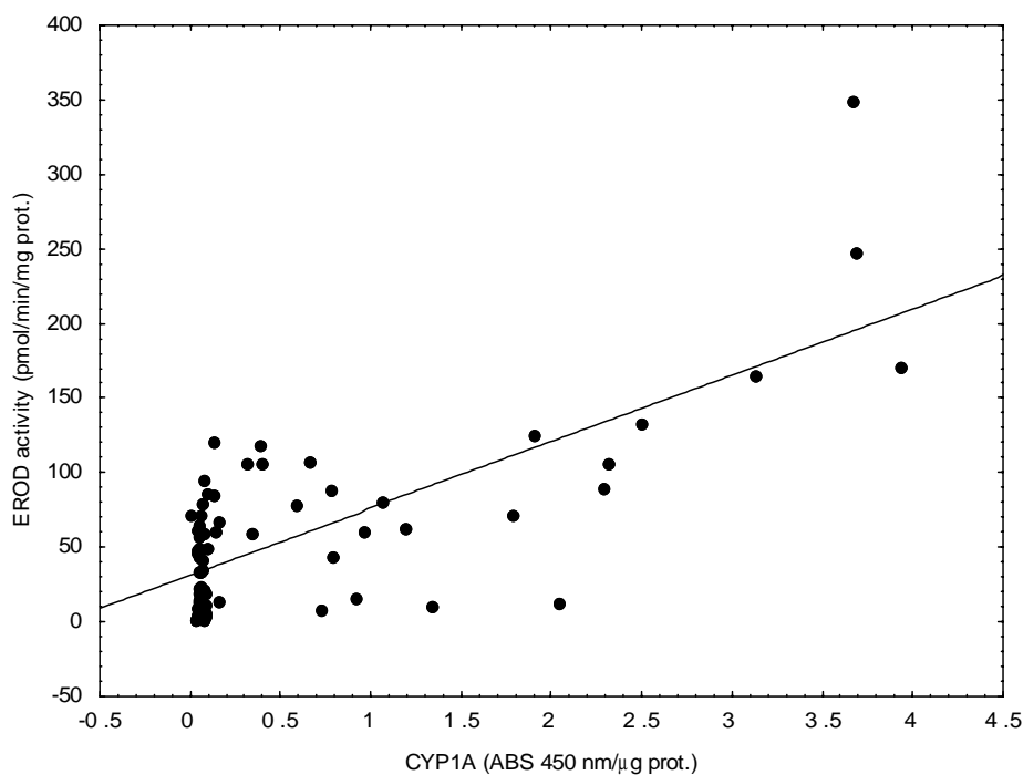
Figure 16. Concentration of cytochrome P4501A protein (CYP1A) versus EROD activity. The regression is significant ( p < 0.0001 ) with a correlation coefficient R^2 = 0.53 .
