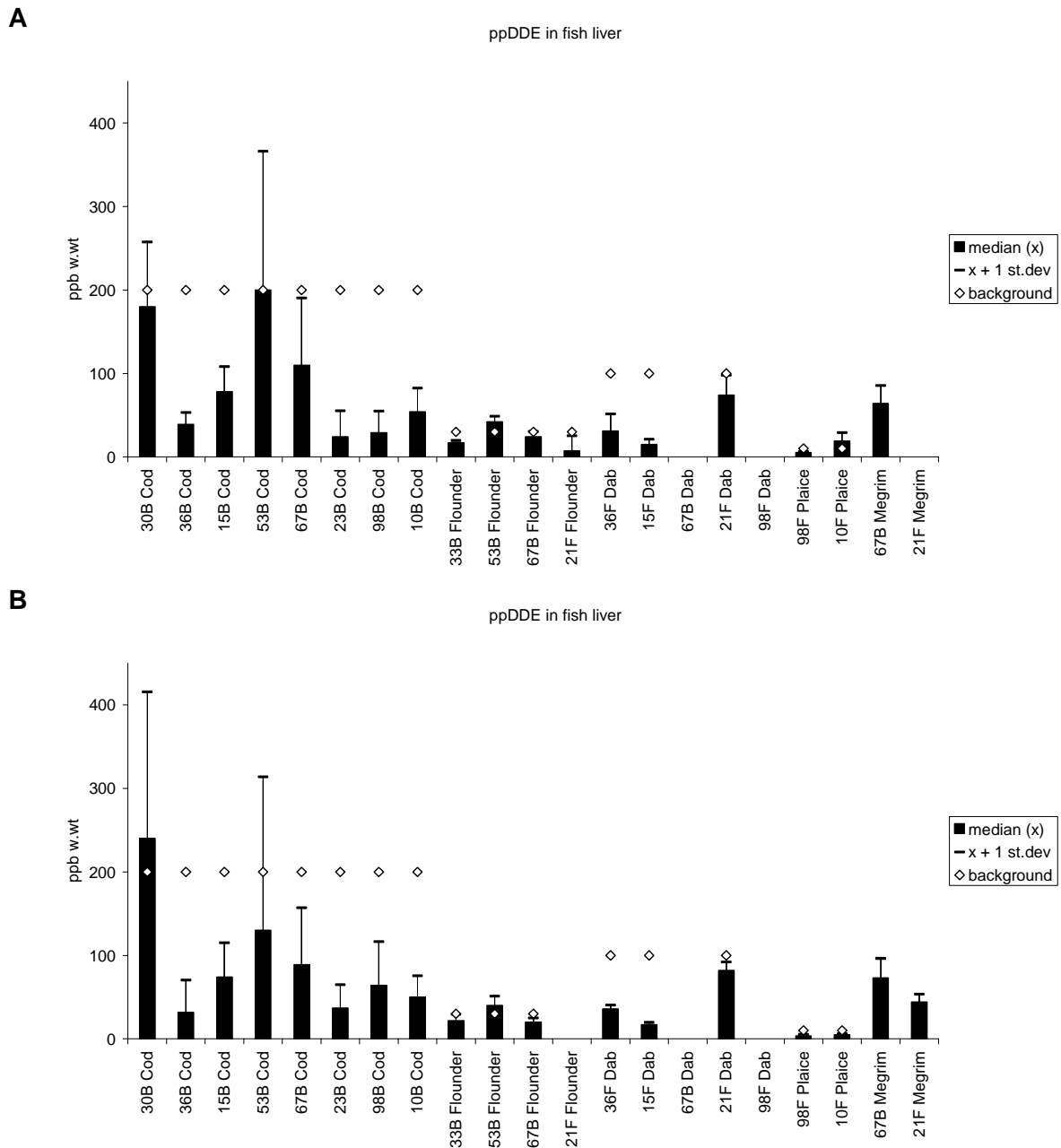
Figure 30. Median, standard deviation and provisional "high background" concentration for ppDDE (DDEPP) in fish liver 2002 ( A ) and 2003 ( B ), ppb ( \mu\text{g}/\text{kg} ) wet weight (see maps in Appendix F). (See also footnote in Table 6).
