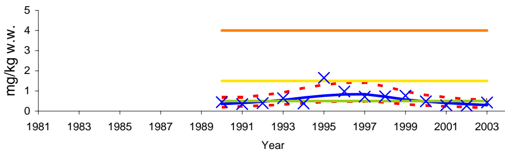
\Sigma PCB-7, Gadus morhua , liver, 36B Outer Oslofjord
