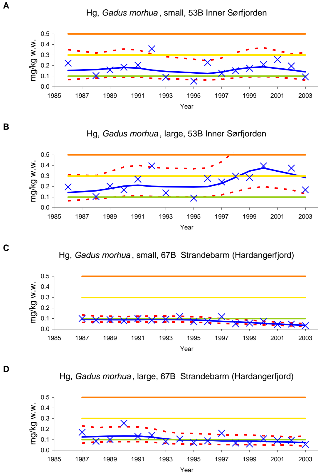
Figure 9. Median mercury (Hg) concentration in fillet of cod ( Gadus morhua ): from Sør fjorden (st.53B) for “small” (A) and “large” (B) fish and Hardangerfjord (st.67B) for “small” (C) and “large” (D) fish (cf. Appendix F and Appendix H, and key in Figure 20). Note: for some years the upper confidence interval line is off-scale in Figure B.
