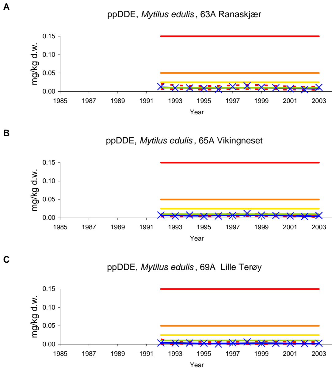
Figure 11. Median ppDDE concentrations in blue mussel ( Mytilus edulis ) from Hardangerfjord (st. 63A, 65A and 69A). (cf. Appendix F and Appendix H, and key in Figure 20). Note: horizontal line for Class I is near x-axis.
