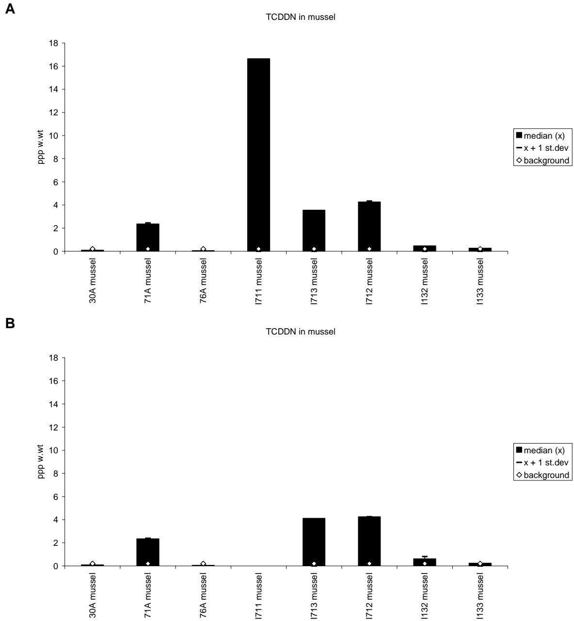
Figure 36. Median, standard deviation and provisional "high background" concentration for dioxin TCDD-toxicity equivalents after nordic model (TCDDN) in mussels 2002 ( A ) and 2003 ( B ), ppp (ng/kg) wet weight (see maps in Appendix F). NB: TCDDN is a sum of specific dioxin compounds of which may be of uncertain quantification.
