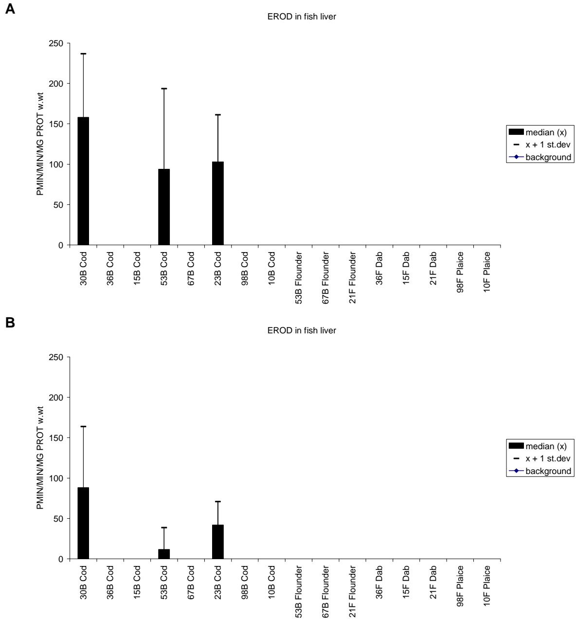
Figure 39. Median and standard deviation activity for EROD (Cytochrome P4501A-activity) in fish liver 2002 (A) and 2003 (B), pmol/min/mg protein (see maps in Appendix F).
