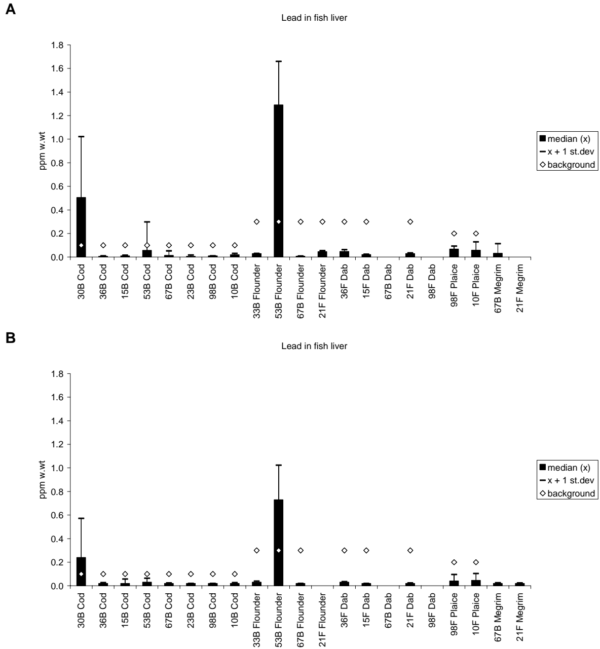
Figure 26. Median, standard deviation and provisional "high background" concentration for lead in fish liver 2002 ( A ) and 2003 ( B ), ppm (mg/kg) wet weight (see maps in Appendix F).
