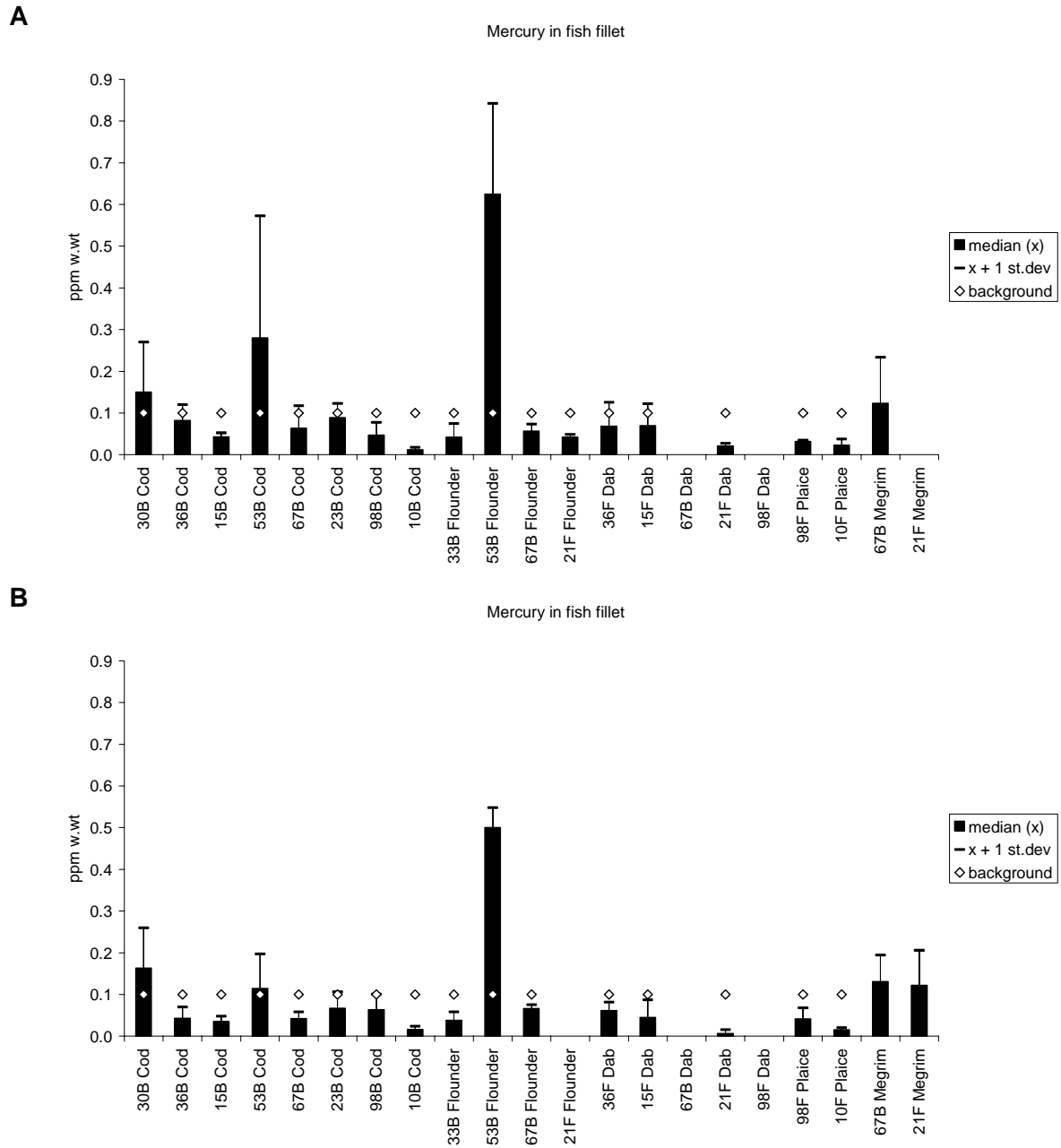
Figure 24. Median, standard deviation and provisional "high background" concentration for mercury in fish fillet 2002 ( A ) and 2003 ( B ), ppm (mg/kg) wet weight (see maps in Appendix F).
