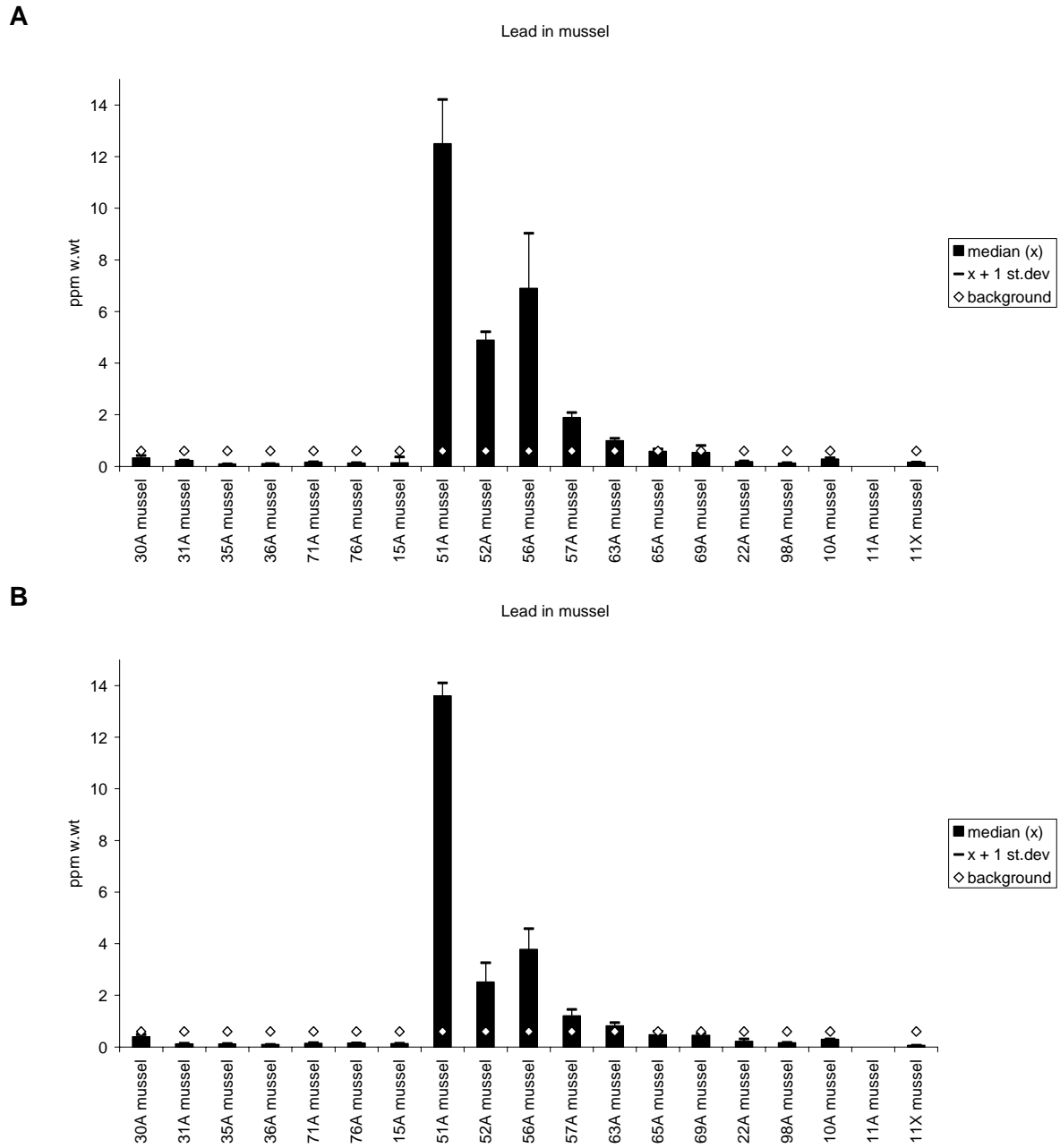
Figure 25. Median, standard deviation and provisional "high background" concentration for lead in mussels ( Mytilus edulis ) 2002 ( A ) and 2003 ( B ), ppm (mg/kg) wet weight (see maps in Appendix F).
