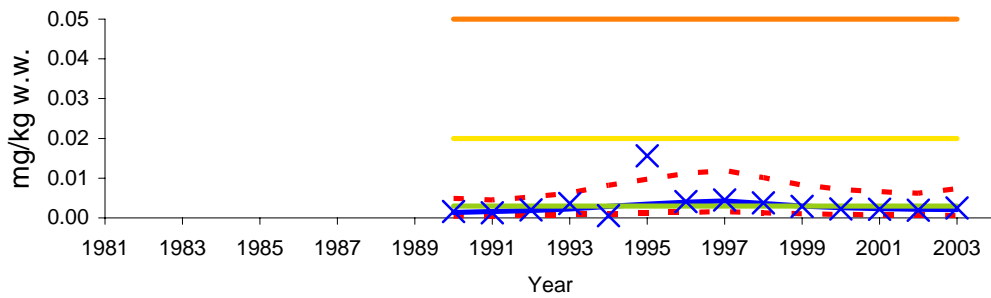
Figure 2. Median \Sigma PCB-7 (sum of PCB 28, 52, 101, 118, 138, 153 and 180) concentration in liver and fillet of cod ( Gadus morhua ) from the inner (st.30B) to outer (st.36B) Oslofjord. (cf. Appendix F and Appendix H, and key in Figure 20).
