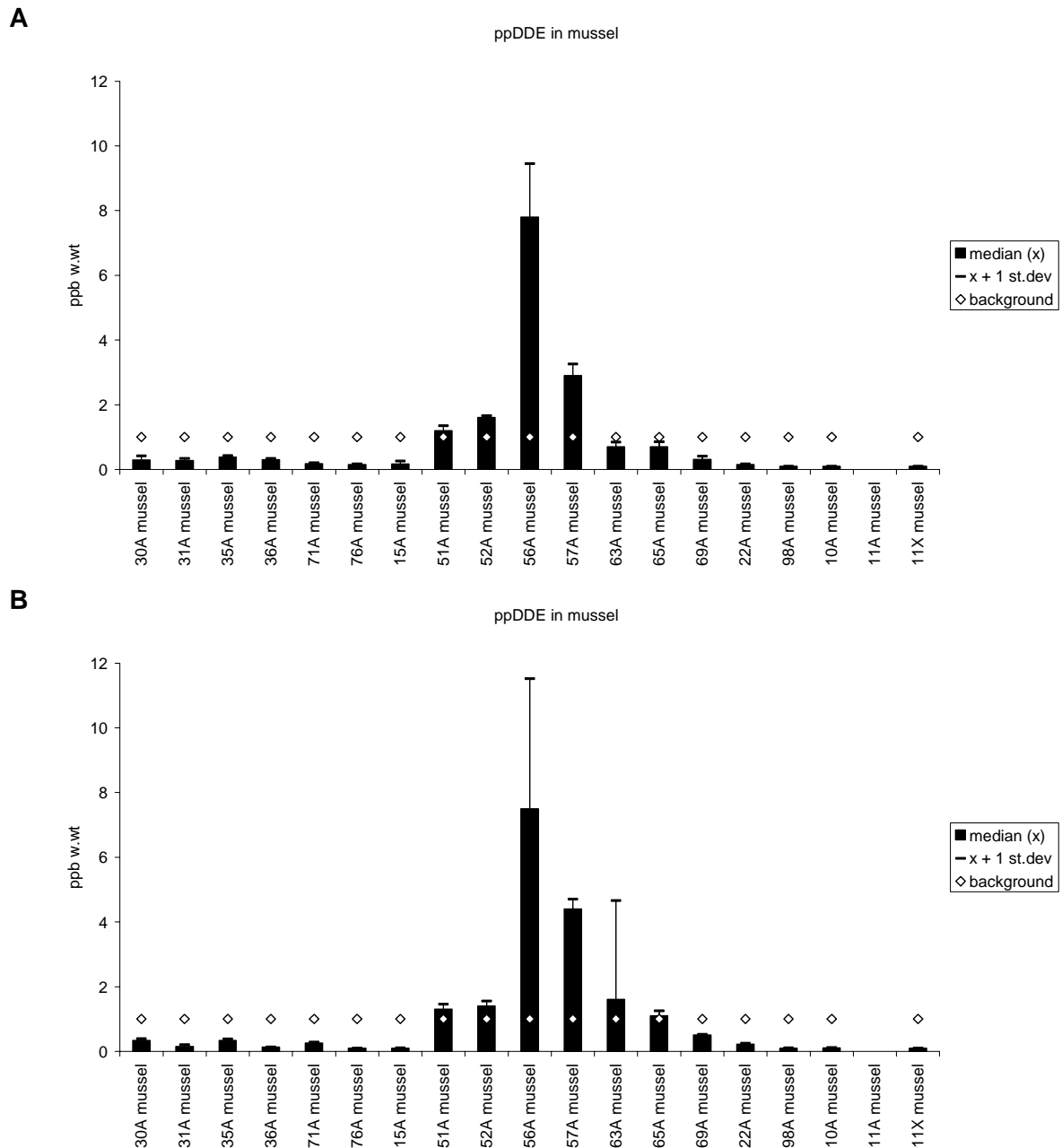
Figure 29. Median, standard deviation and provisional "high background" concentration for ppDDE (DDEPP) in mussels ( Mytilus edulis ) 2002 ( A ) and 2003 ( B ), ppb ( \mu\text{g}/\text{kg} ) wet weight (see maps in Appendix F). (See also footnote in Table 6).
