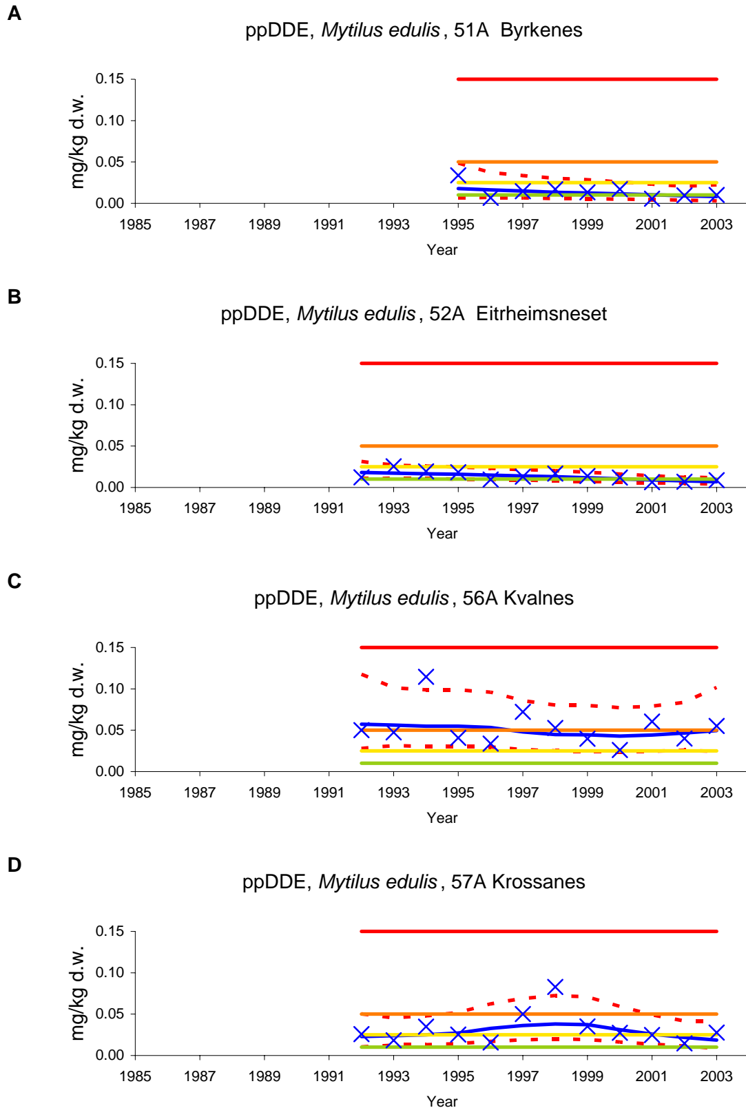
Figure 10. Median ppDDE concentration in blue mussel ( Mytilus edulis ) from inner (st.51A) to outer (st.57A) Sør fjord. (cf. Appendix F and Appendix H, and key in Figure 20). Note: horizontal line for Class I is near x-axis.
