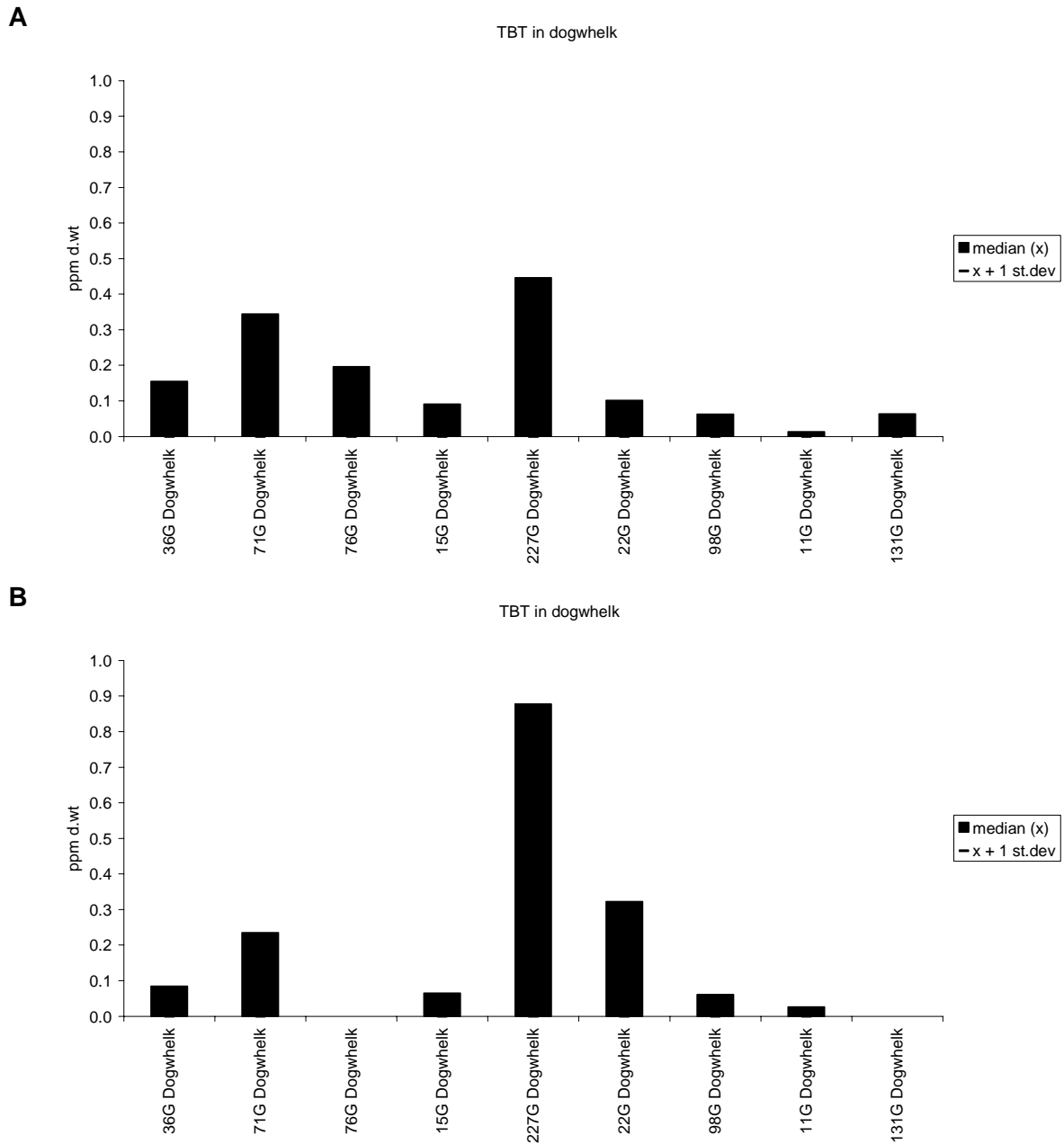
Figure 41. Median, standard deviation and provisional "high background" concentration for tributyl tin (TBT-concentration on a formulation basis) in dogwhelks 2002 ( A ) and 2003 ( B ), ppm (2.44* mg Sn/kg) dry weight (see maps in Appendix F).
