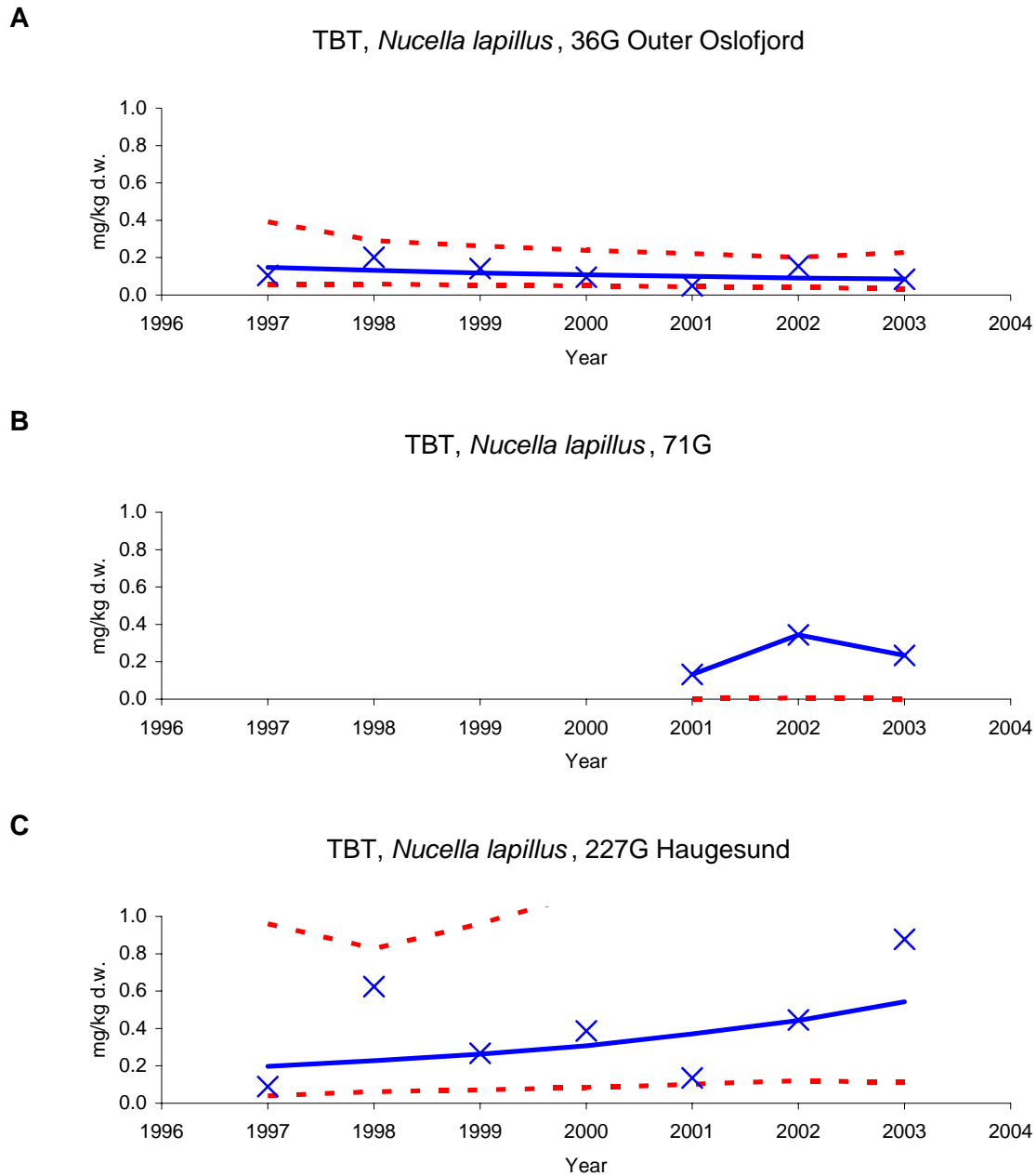
Figure 17. Median concentration of TBT (on a formulation basis) in dog whelks ( Nucella lapillus ) from outer Oslofjord (st.36G), Langesundsfjord (west of Oslofjord) (st.71G) and Haugesund (St.227G), mg/kg (mg TBT/kg) dry weight. NB: (cf. Appendix F and Appendix H, and key in Figure 20). Note: for some years the upper confidence interval line is off-scale in Figures B and C.
