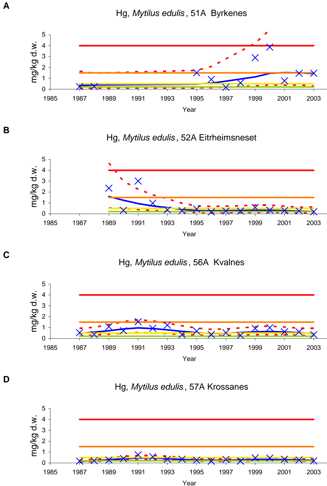
Figure 8. Median mercury (Hg) concentration in blue mussel ( Mytilus edulis ) from inner (st.51A) to outer (st.57A) Sør fjord. (cf. Appendix F and Appendix H, and key in Figure 20). Note: for some years the upper confidence interval line is off-scale in figure A. Note: horizontal lines for Classes I and II are near x-axis.
