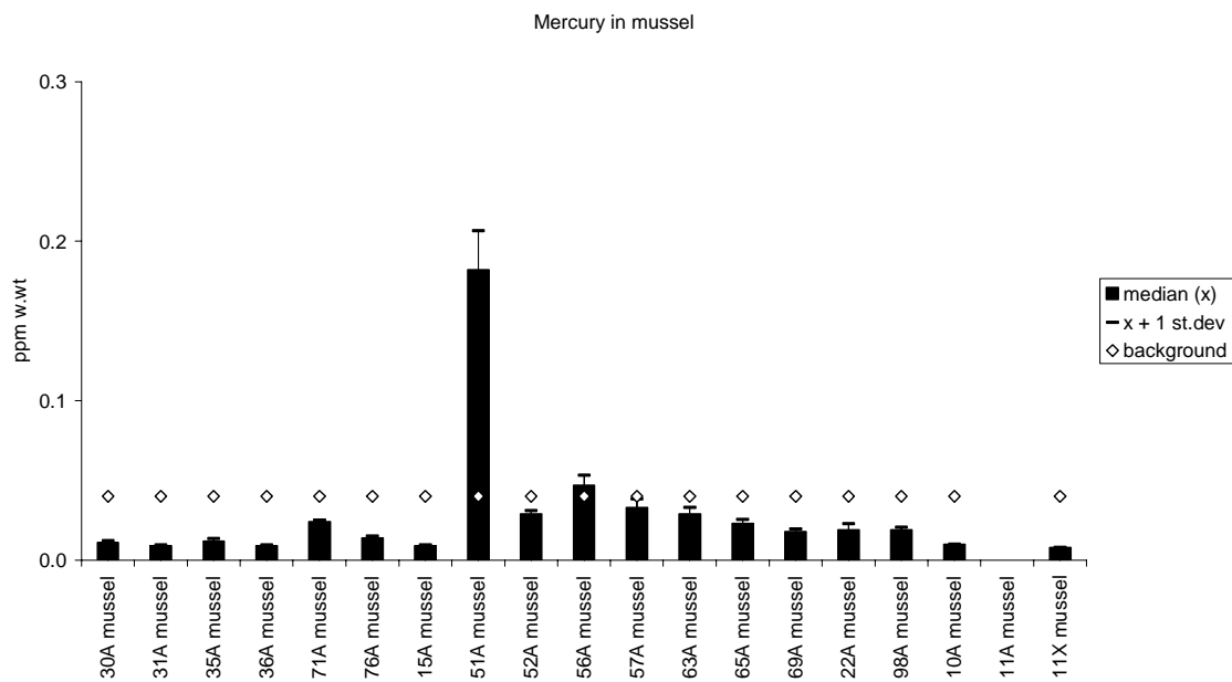
Figure 23. Median, standard deviation and provisional "high background" concentration for mercury in mussels ( Mytilus edulis ) 2002 ( A ) and 2003 ( B ), ppm (mg/kg) wet weight (see maps in Appendix F).
