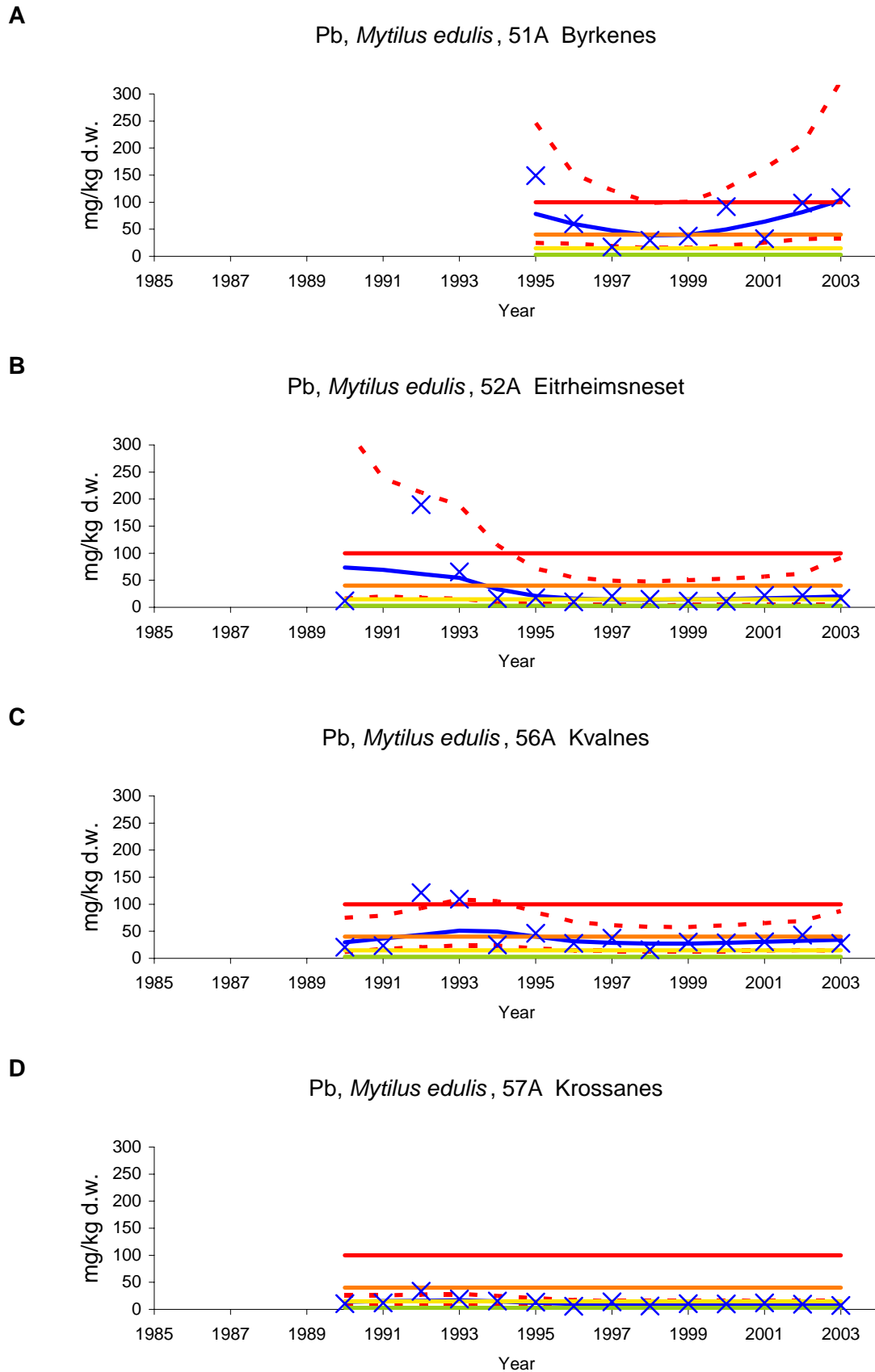
Figure 7. Median lead (Pb) concentration in blue mussel ( Mytilus edulis ) from inner (st.51A) to outer (st.57A) Sør fjord. (cf. Appendix F and Appendix H, and key in Figure 20). Note: horizontal lines for Classes I and II are near x-axis.
