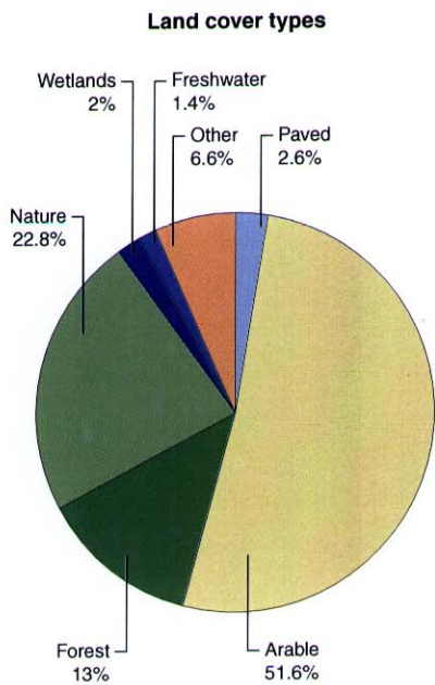
Figure 2: Main land use classes in the Guadiamar catchment.
