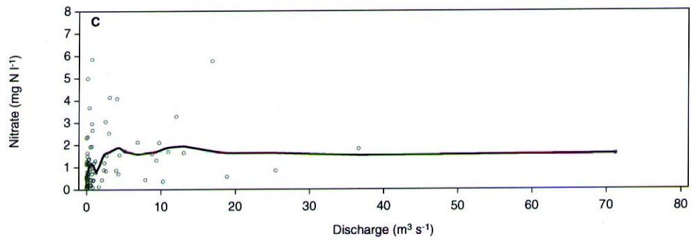
Figure 12: Relationships between discharge and concentrations of nitrate nitrogen established applying the LOWESS fitting procedure (see Annex 3).
