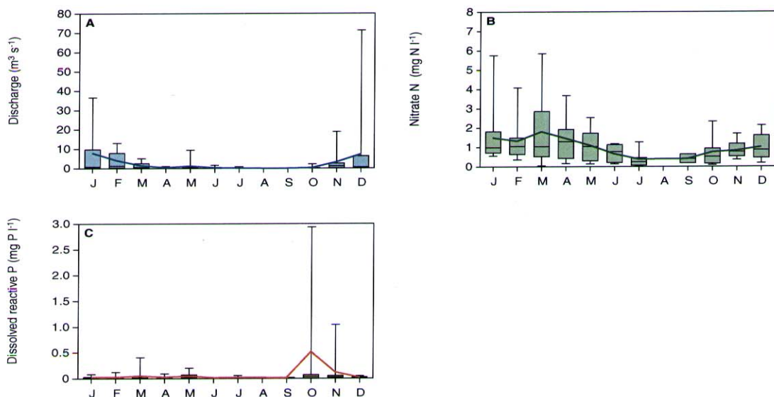
Figure 8: Box-Whisker plots showing the variation in runoff, nitrate nitrogen and dissolved reactive phosphorus concentrations in the catchment.
