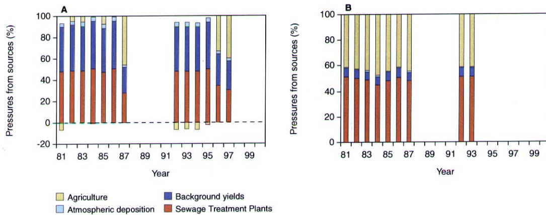
Figure 6: Source apportionment of annual nitrate nitrogen (left) and dissolved reactive phosphorus (right) exports from the catchment.
