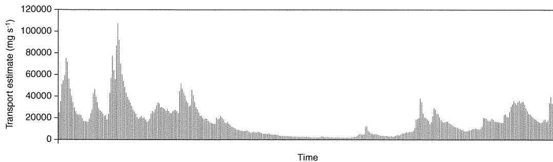
Figure 3: Daily estimated fluxes (product of runoff and estimated concentration).
