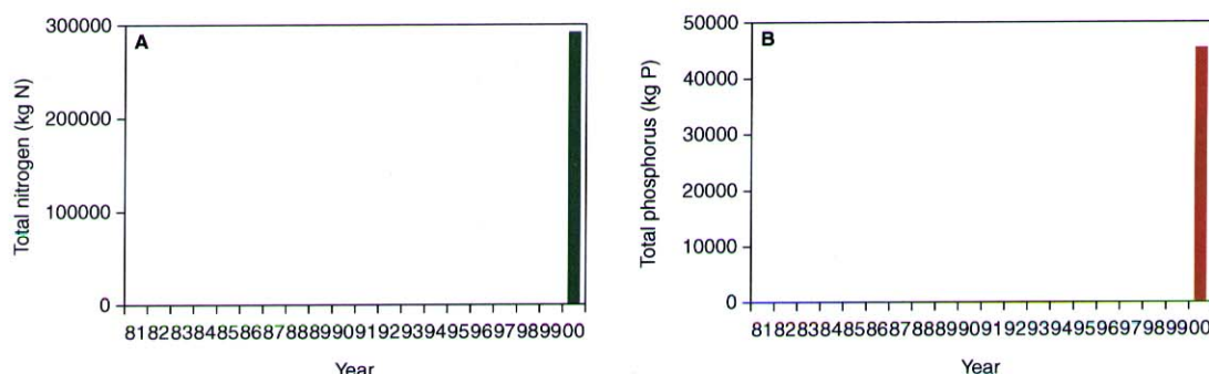
Figure 4: Annual estimated discharge of total nitrogen and total phosphorus from inhabitants living in the Guadiamar catchment.
