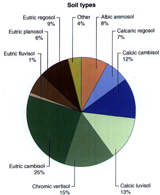
Figure 3: Main soil types in the Guadiamar catchment.
