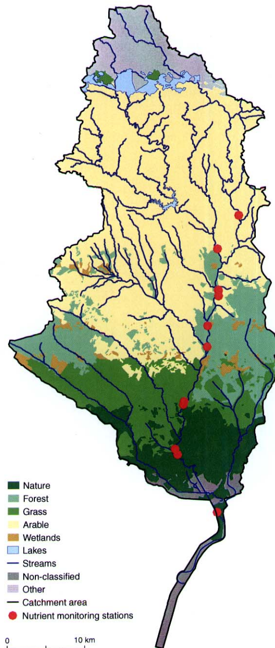
Figure 1: Map showing land use and river network characteristics for the Guadiamar catchment, Spain, and existing water quality monitoring stations in the catchment.
