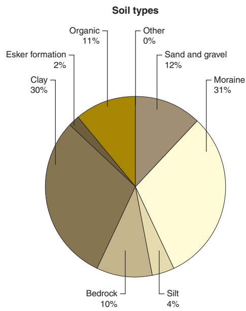
Figure 3: Main soil types in the Eurajoki catchment.
