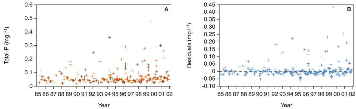
Figure 10: Time-series of flow-adjusted concentrations of total phosphorus and the flow-adjusted concentrations (residuals) during the period 1985-2002. The average concentration of total phosphorus is 0.068 mg l -1 (CV=82%).
