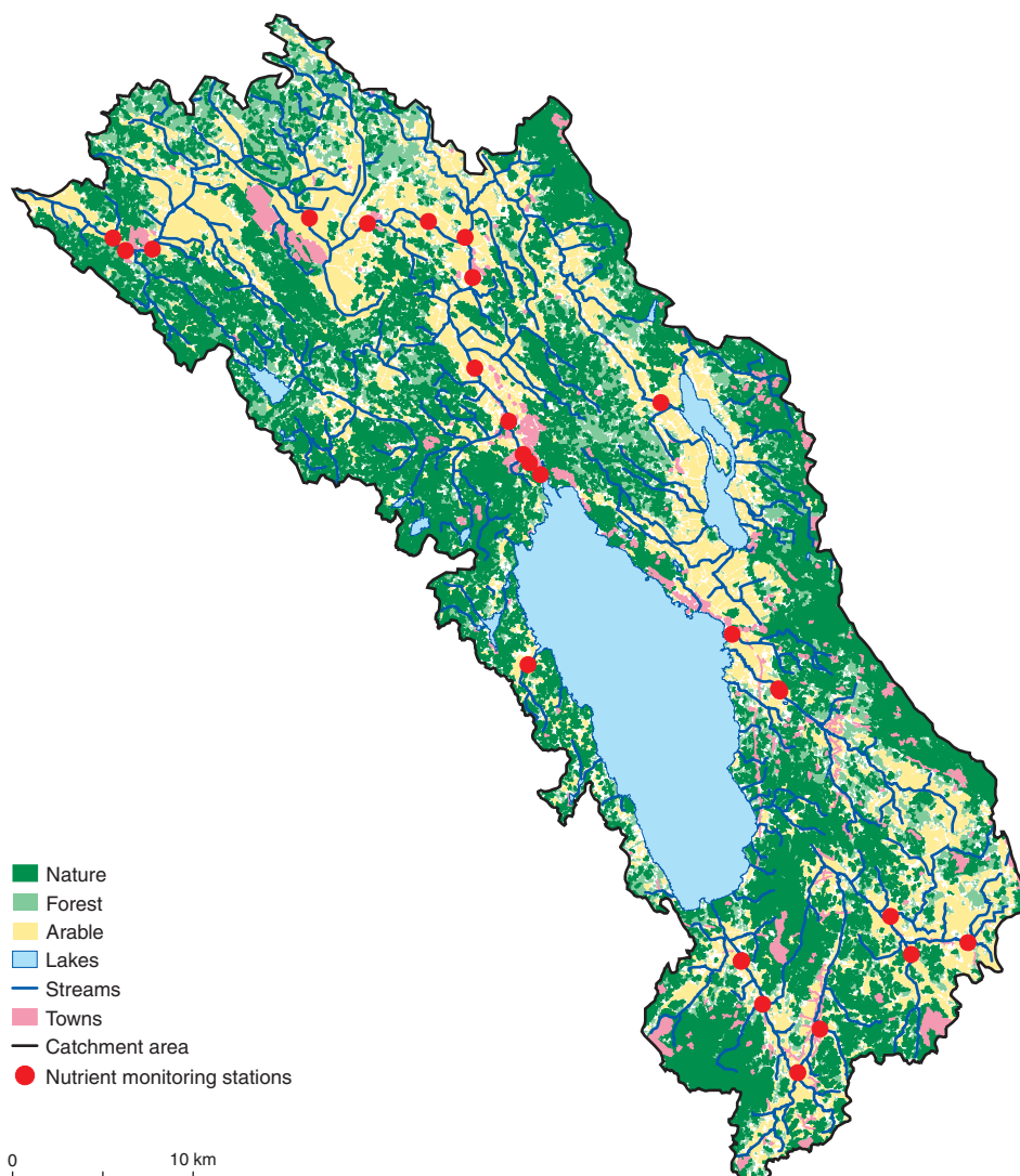
Figure 1: Map showing land use and river network characteristics for the Eurajoki catchment, Finland, and existing water quality monitoring and hydrometric stations in the catchment.
