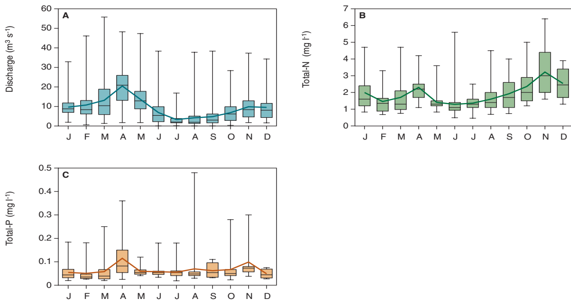
Figure 8: Box-Whisker plots showing the variation in runoff, total nitrogen and total phosphorus concentrations in the catchment.
