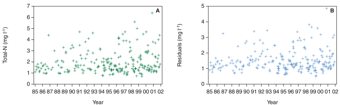
Figure 9: Time series of concentrations of total N and the flow-adjusted concentrations (residuals) during the period 1985-2001. Average concentration of total nitrogen is 1.86 \text{ mg l}^{-1} ( \text{CV}=54\% ).
