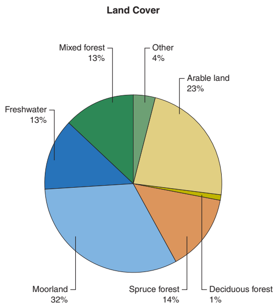
Figure 2: Main land use classes in the Eurajoki catchment.
