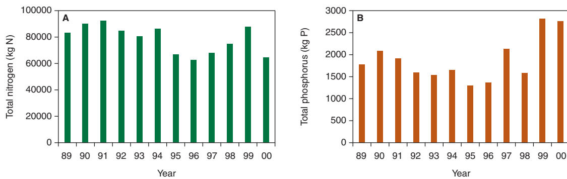
Figure 4: Annual discharge of total nitrogen and total phosphorus from WWTPs in the Eurajoki catchment.
