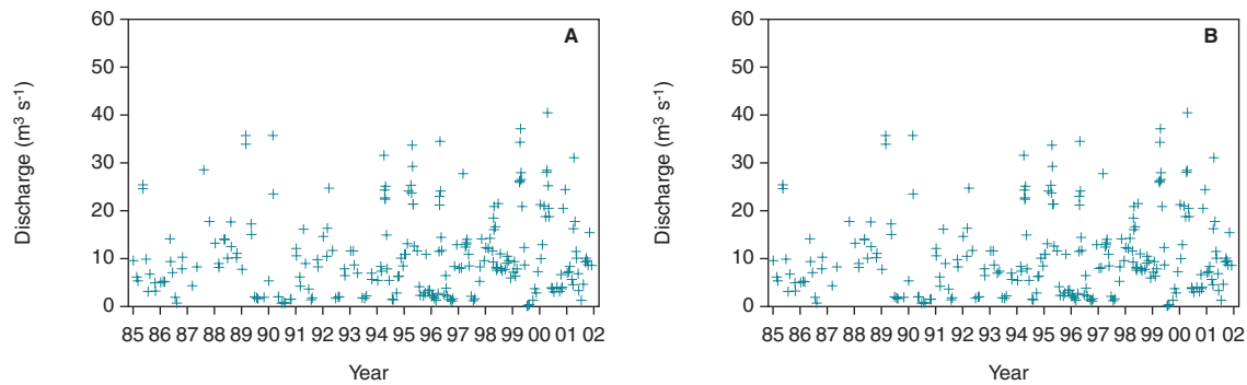
Figure 11: Mean daily discharge at the days of water sampling during the period 1985-2001. Figure 10A shows discharge at measurement days for dissolved inorganic nitrogen and Figure 10B discharge for measurement days for total phosphorus.
