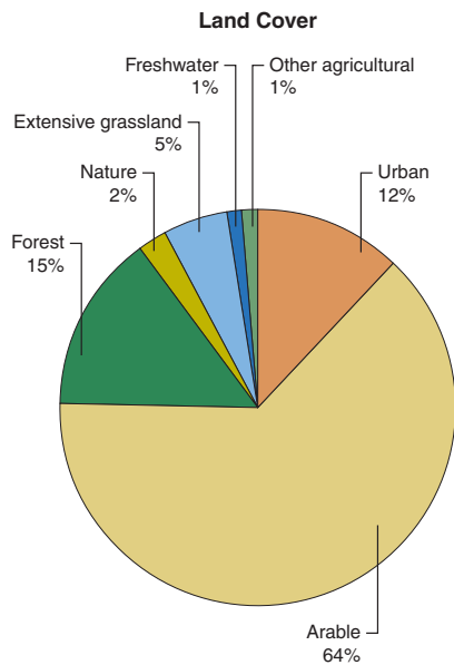
Figure 2: Main land use classes in the Vechte catchment.
