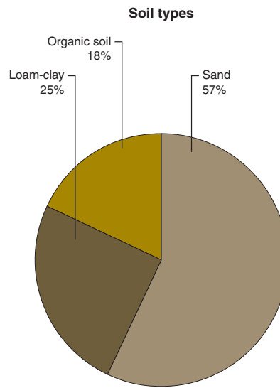
Figure 3: Main soil types in the Vechte catchment.
