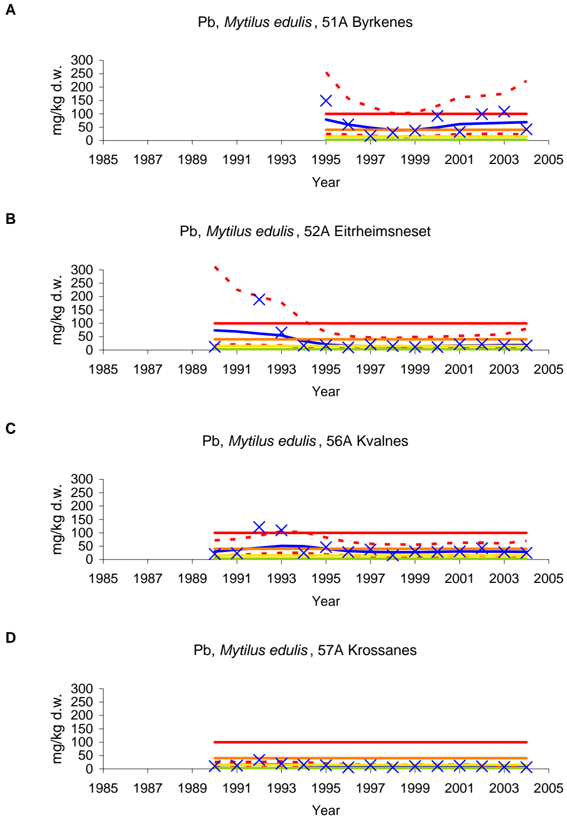
Figure 7. Median lead (Pb) concentration in blue mussel ( Mytilus edulis ) from inner (st.51A) to outer (st.57A) Sørfjord. (cf. Appendix G and Appendix I, and key in Figure 21). Note: horizontal lines for Classes I and II are near x-axis.
