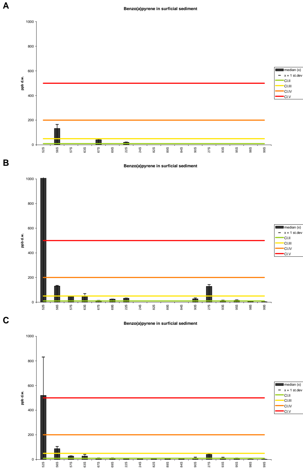
Figure 50. Median, standard deviation and provisional "high background" concentration for Benzo[a]pyrene (BAP) in surficial sediment (0-2cm) 1987-1990 ( A ), 1992-1997 ( B ) and 2004 ( C ), ppb ( \mu\text{g}/\text{kg} ) dry weight (see maps in Appendix G). Note: for some stations the standard deviation is off-scale in figure B.
