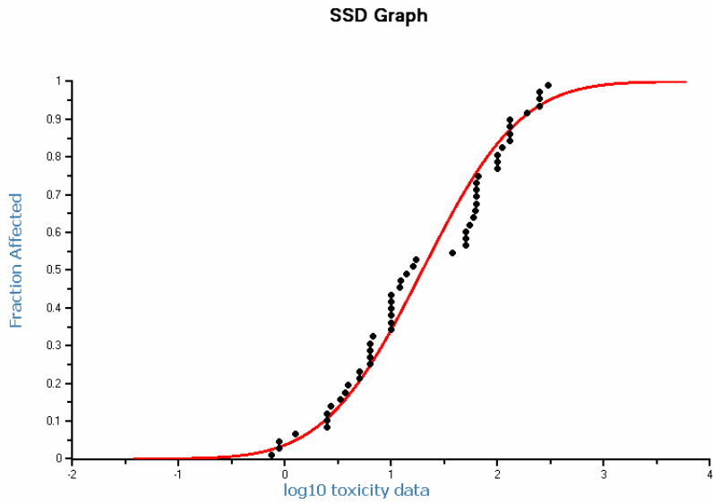
Figure 5. Distribution of NOECs for copper – salt water data
