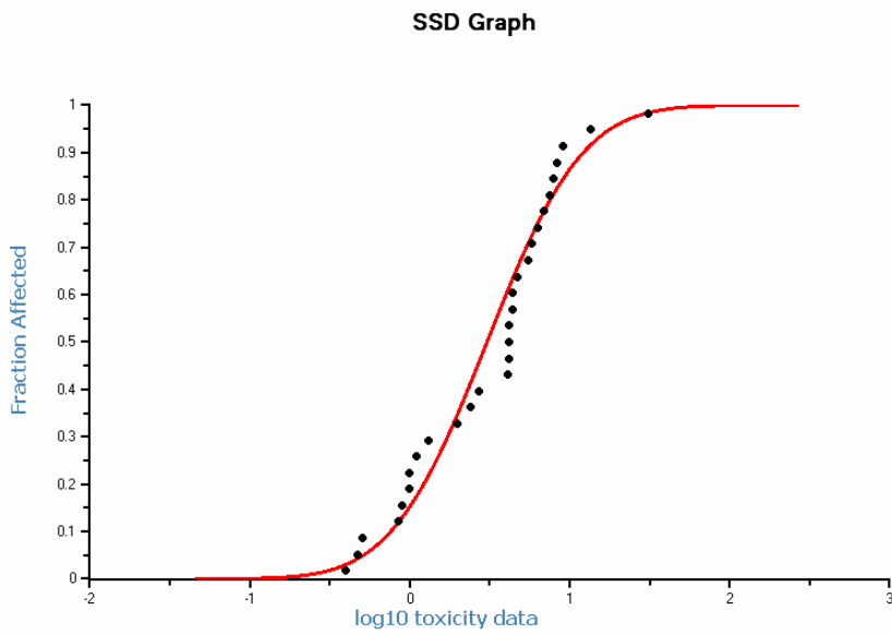
Figure 1. Distribution of NOECs for cadmium – freshwater data
