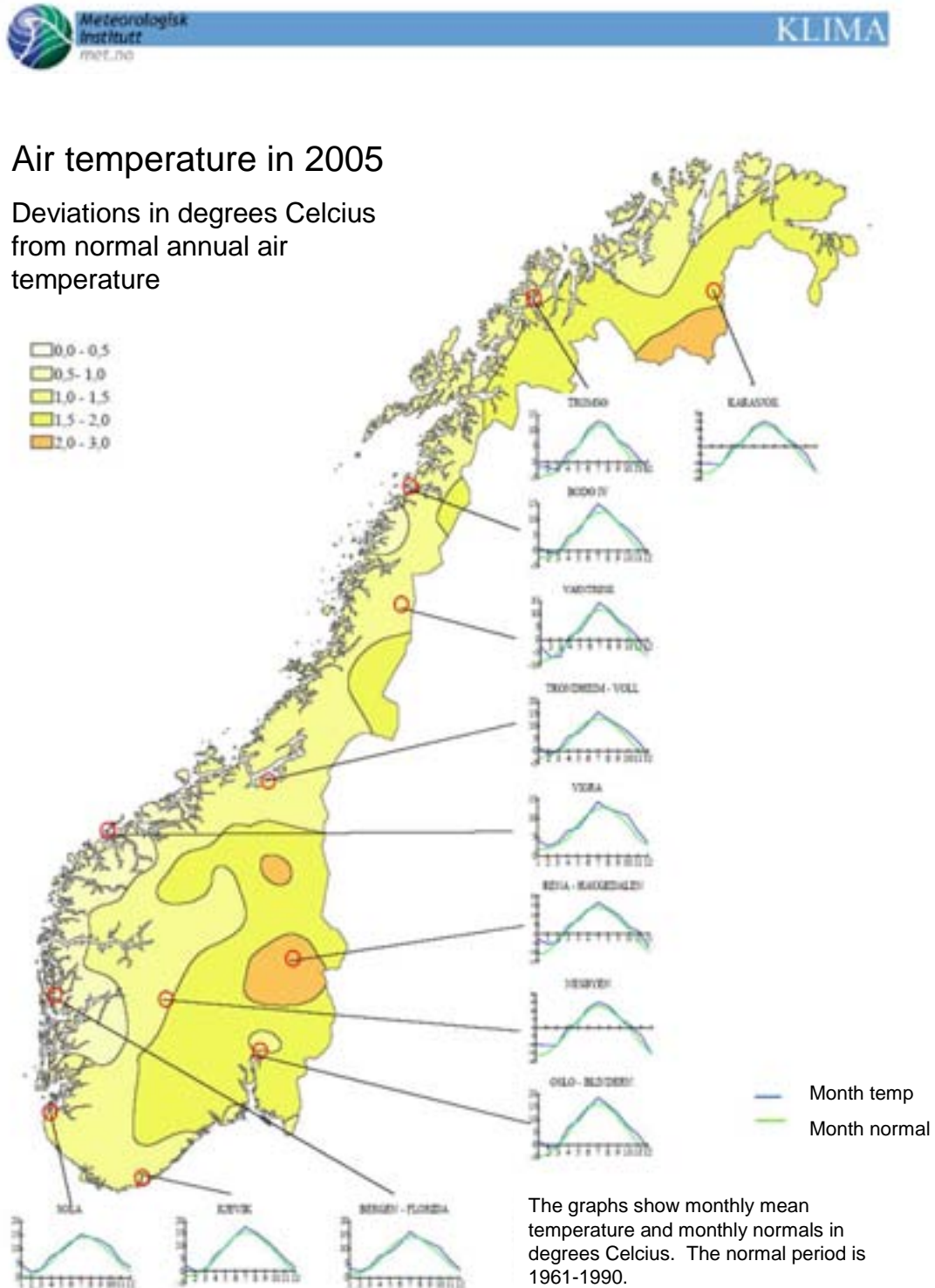
Figure 10. Air temperature in 2005 in Norway. Source: Norwegian Meteorological Institute (met.no).
