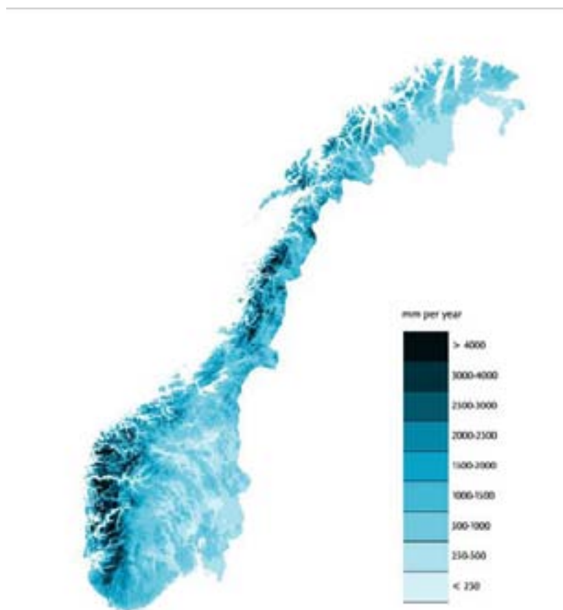
Figure 16. Annual average runoff (mm/year) for Norway for the period 1961-1990.
