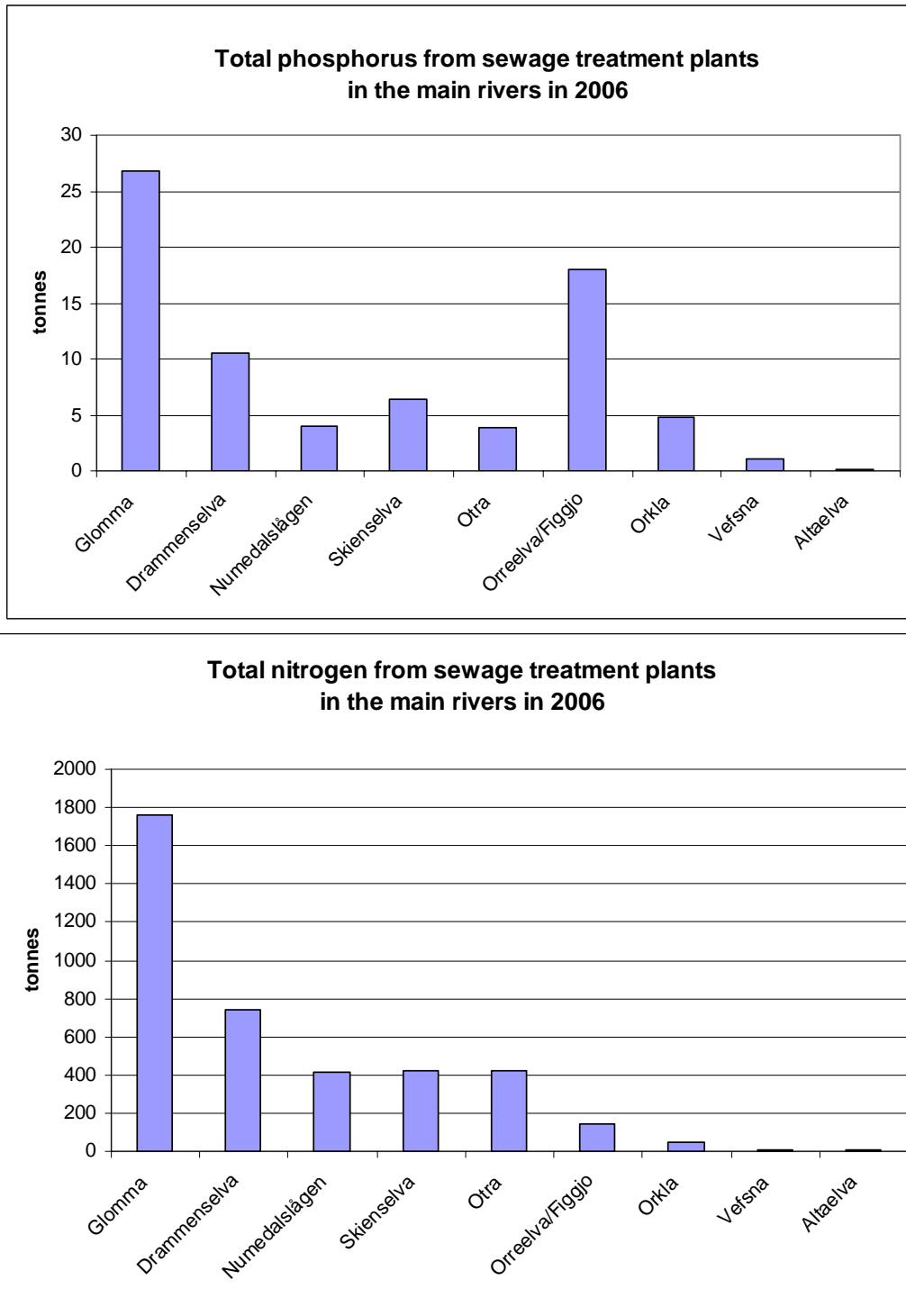
Figure 5. Discharge of phosphorus (top) and nitrogen (bottom) from sewage treatment plants in the catchment areas of rivers monitored monthly. Note that Ørreelva also includes River Figgjo.
