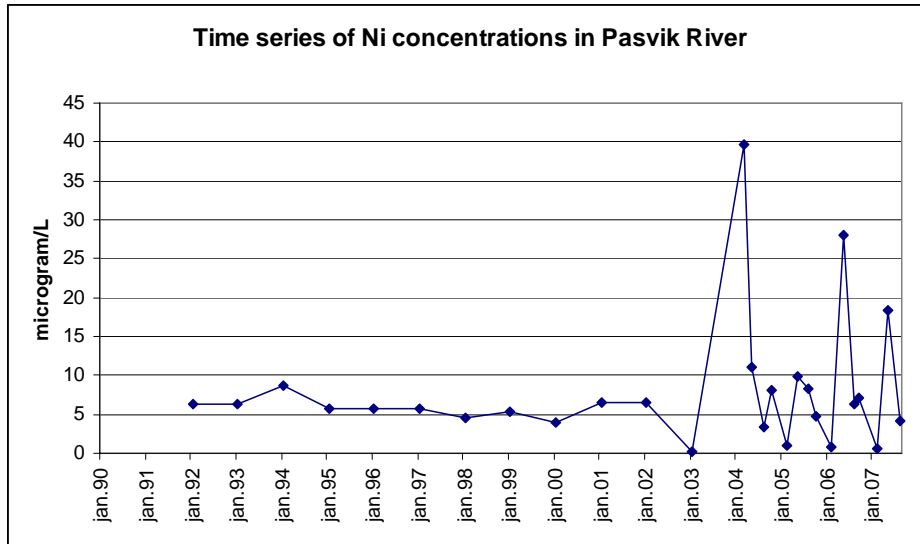
Figure 31. Time series of nickel concentrations in the Pasvik River.
