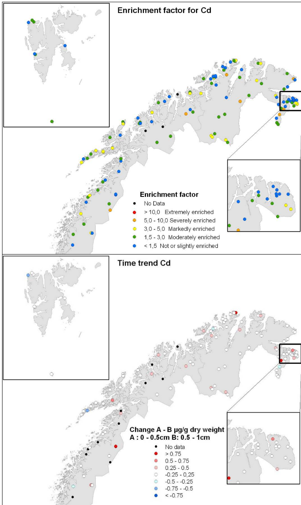
Figure 15. Enrichment factor for cadmium (Cd) in surface sediments (upper figure) and differences in concentrations ( \mu\text{g/g} dw) of Cd between surface layer (0 - 0.5 cm) and subsurface layer (0.5 - 1.0 cm) (lower figure).
