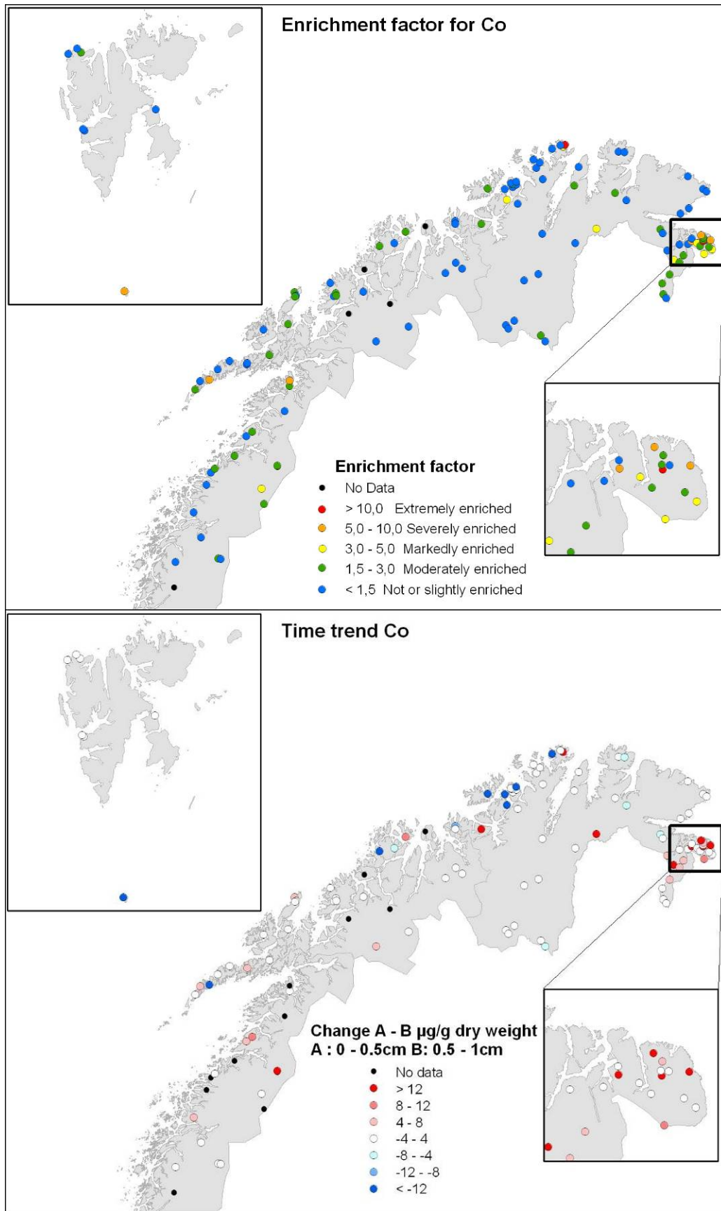
Figure 33. Enrichment factor for cobalt (Co) in surface sediments (upper figure) and differences in concentrations ( \mu\text{g/g dw} ) of Co between surface layer (0 - 0.5 cm) and subsurface layer (0.5 - 1.0 cm) (lower figure).
