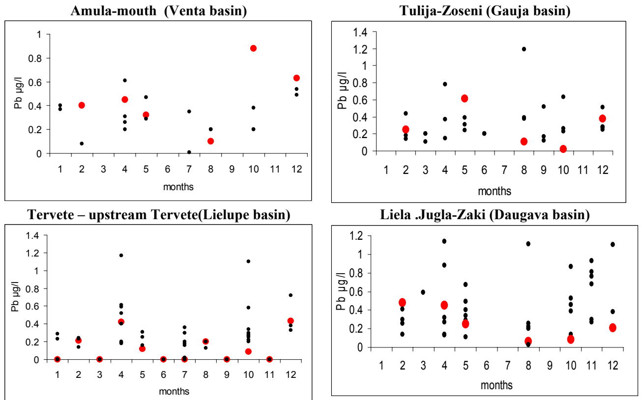
Figure 6. Pb concentrations in ICP Waters sites (red) against other river basins (black), 2007
