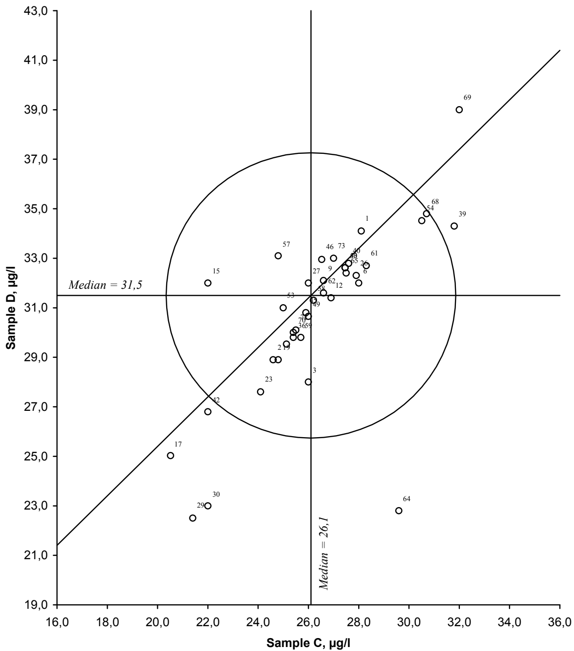
Figure 19. Youden diagramme for zinc, sample pair CD Acceptance limit, given by the circle, is 20 %
