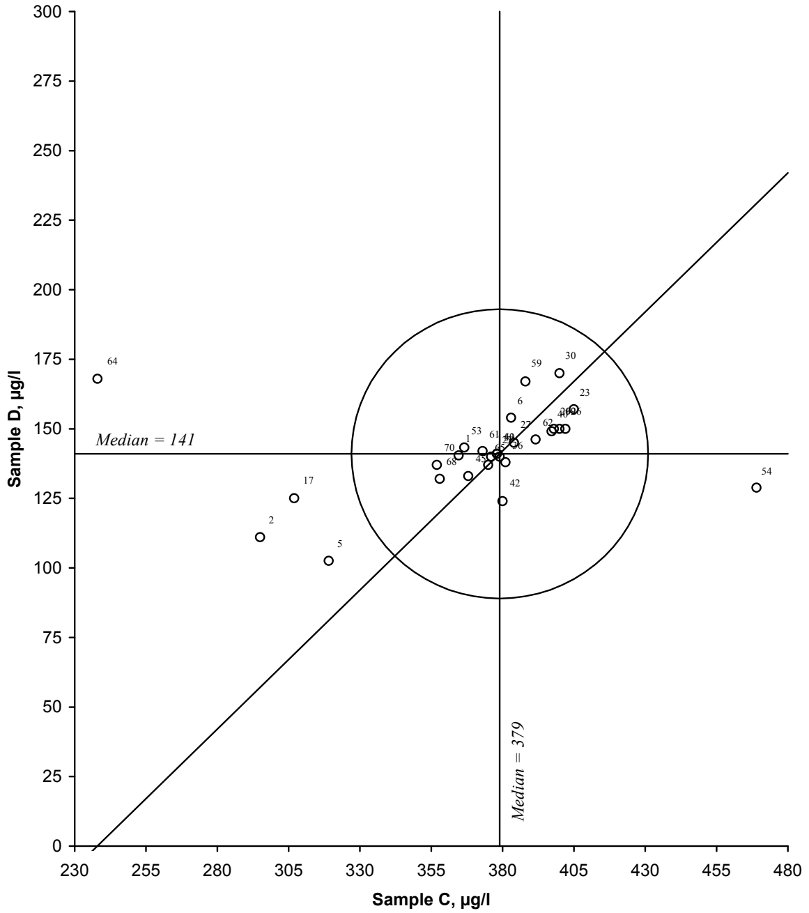
Figure 12. Youden diagramme for aluminium, sample pair CD Acceptance limit, given by the circle, is 20 %
