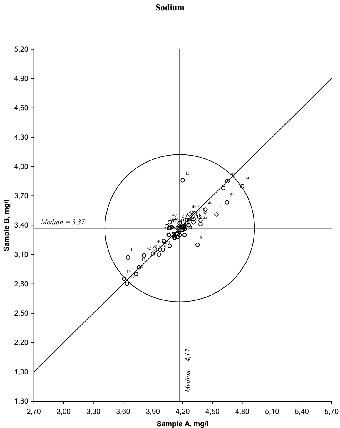
Figure 9. Youden diagramme for sodium, sample pair AB Acceptance limit, given by the circle, is 20 %
