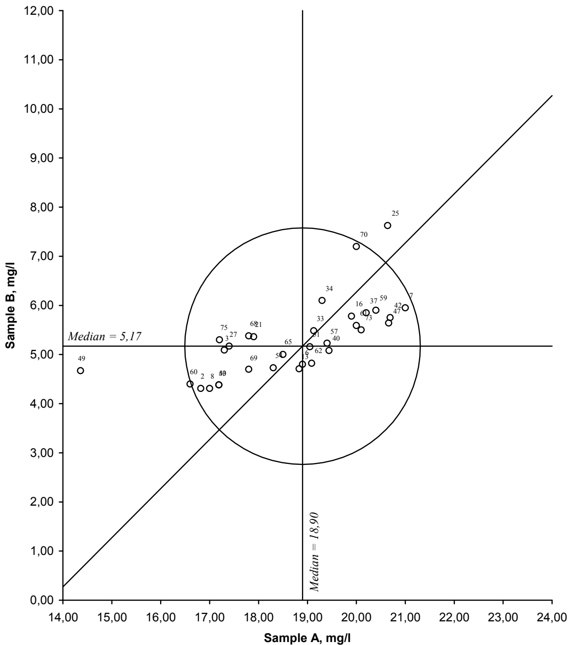
Figure 11. Youden diagramme for total organic carbon, sample pair AB Acceptance limit, given by the circle, is 20 %
