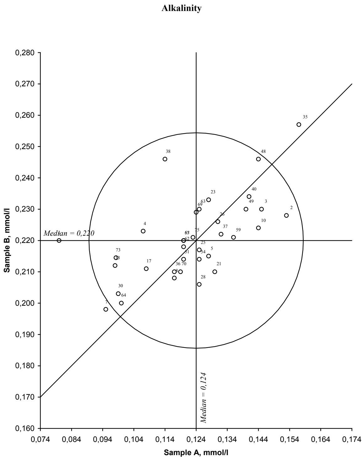
Figure 3. Youden diagramme for alkalinity, sample pair AB Acceptance limit, given by the circle, is 20 %
