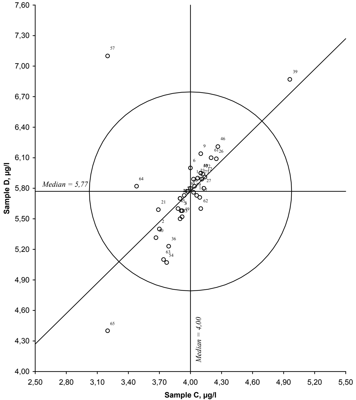
Figure 15. Youden diagramme for cadmium, sample pair CD Acceptance limit, given by the circle, is 20 %
