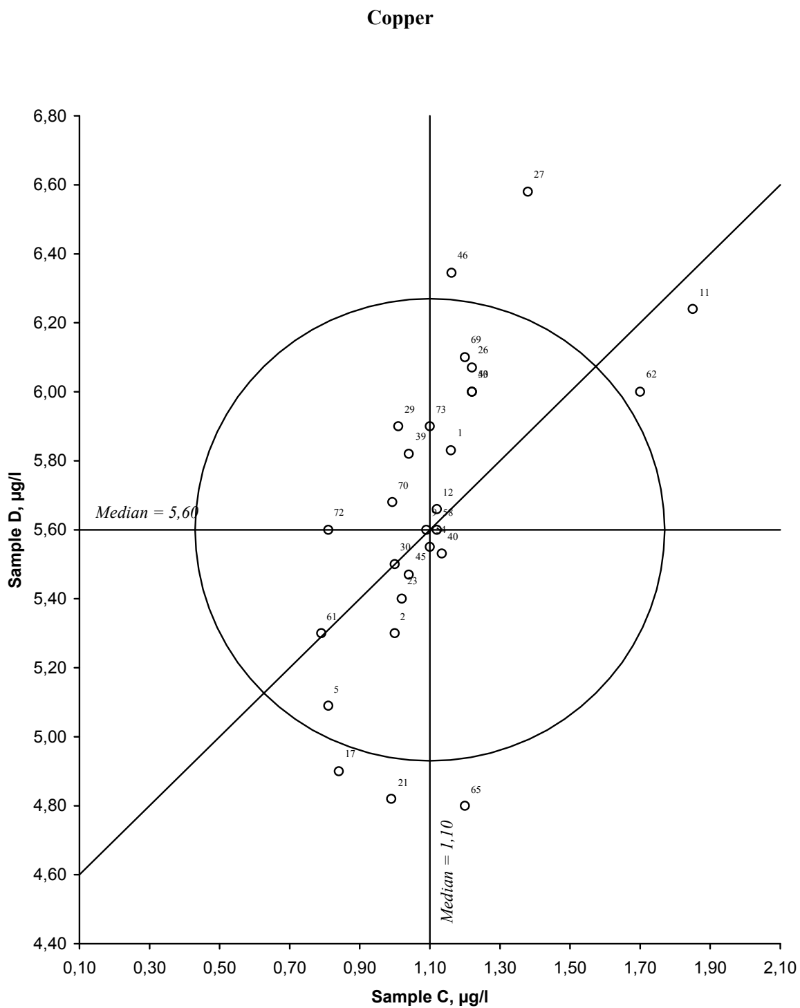
Figure 17. Youden diagramme for copper, sample pair CD Acceptance limit, given by the circle, is 20 %
