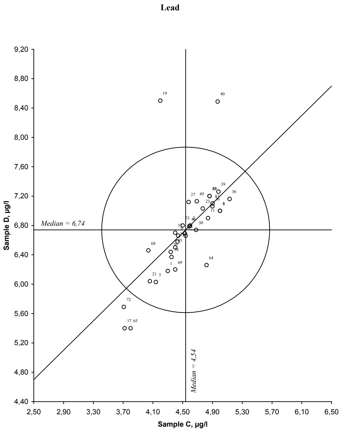
Figure 16. Youden diagramme for lead, sample pair CD Acceptance limit, given by circle, is 20 %
