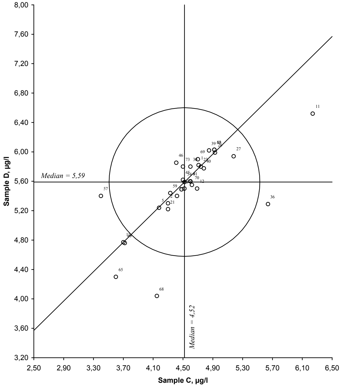
Figure 18. Youden diagramme for nickel, sample pair CD Acceptance limit, given by the circle, is 20 %
