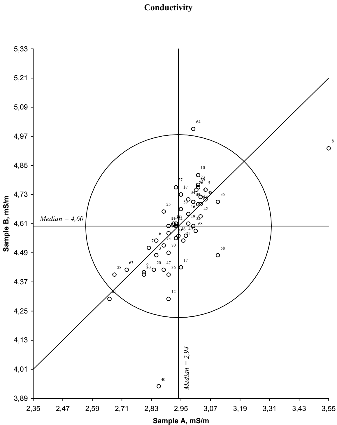
Figure 2. Youden diagramme for conductivity, sample pair AB Acceptance limit, given by the circle, is 10 %
