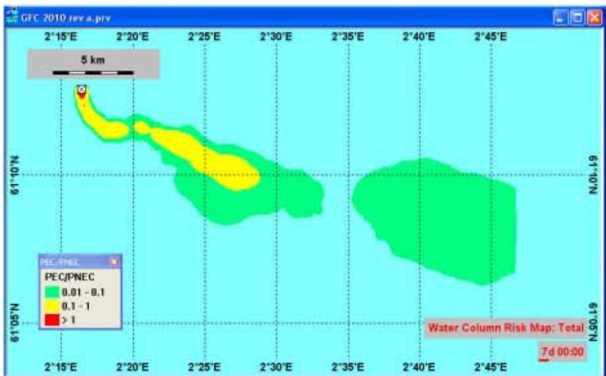
Figure A.2 Modelling of produced water discharges from Gullfaks C. DREAM/ Environmental Impact Factor (EIF) model.
