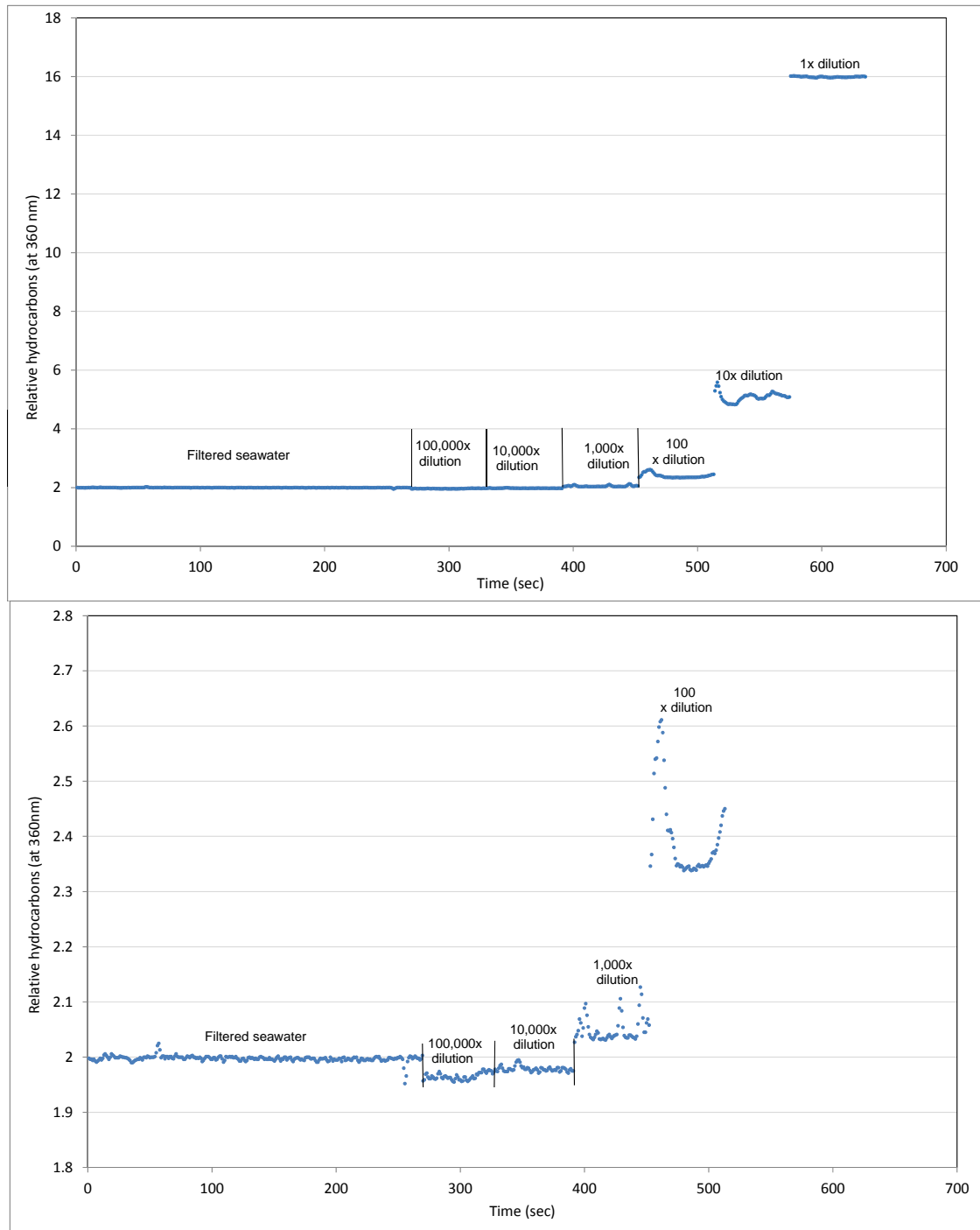
Figure 29. The relative hydrocarbon measurement of the Aquatracka following exposure to varying concentrations of an artificial PW mixture. Graphs present the same data but with different y-axis scaling. 1x dilution refers to the mean concentration of PW chemicals typically found in the Norwegian sector of the North Sea prior to dilution with the receiving water (based on Holth et al., 2008), with subsequent 10-fold dilutions of this with filtered seawater.
