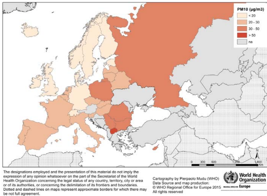
Figure 43: Population weighted annual mean PM10, for 2012 or the last year available.
