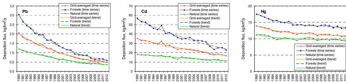
Figure 49: Deposition fluxes of lead (left), cadmium (middle) and mercury (right) for 1990-2012.
