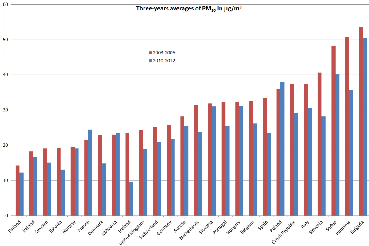
Figure 45: Population weighted annual mean PM 10 , three-year averages, for 2003-2005, and 2010-2012.
