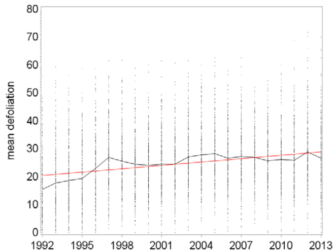
Figure 15: Plot mean defoliation (points) and the defoliation trend (regional Sen's slope, red line) for pedunculate and sessile oak 1992-2013. Black line connects annual means.
