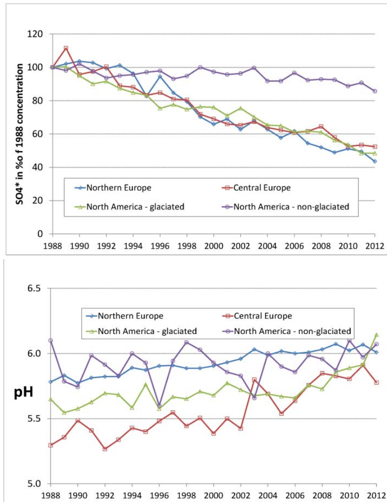
Figure 18: Trends in surface water chemistry at ICP Waters sites 1988-2012. Shown are the mean concentrations of non-marine sulphate ( \text{SO}_4^* ) (top) and pH (bottom) at 22 sites in northern Europe, 21 sites in central Europe, 37 sites in glaciated areas of eastern North America, and 7 sites in non-glaciated areas of eastern North America (Source: Garmo et al. 2015).
