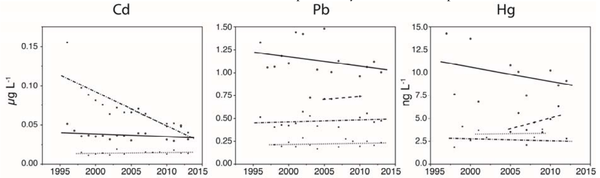
Figure 55: Stream water Cd and Pb ( \mu\text{g L}^{-1} ) and Hg ( \text{ng L}^{-1} ) concentrations at the four ICP IM sites in Sweden (Aneboda (solid line), Gammtratten (dotted line), Gårdsjön (dashed line), Kindla (dotdashed line)).
