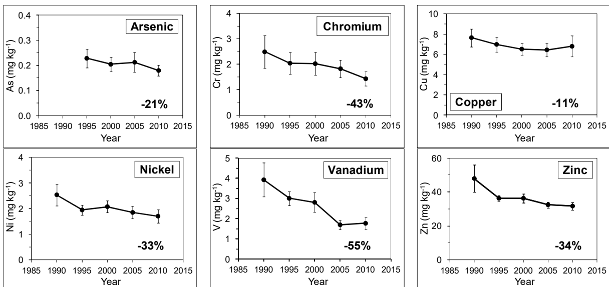
Figure 53: Average median metal concentration in mosses ( \pm one standard error) for countries that reported metal data for at least four survey years since 1990 (1995 for arsenic; Harmens et al. 2015). The values in the graphs represent the percentage change (i.e. a decline) between 1990 (1995 for arsenic) and 2010.
