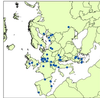
Figure 1: Impacts on white clover between 1996 and 2006 (Hayes et al., 2007).
