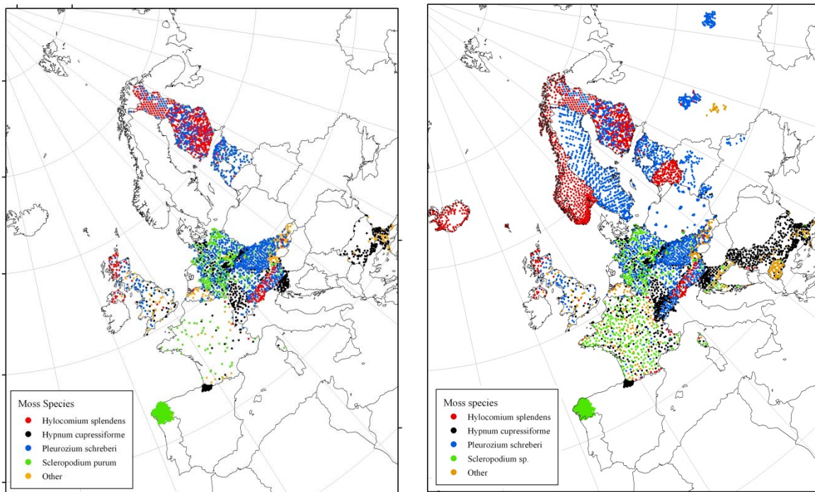
Figure 7: Sampling sites for determination of heavy metal (right) and nitrogen (left) concentrations in mosses in 2005 (Harmens et al. 2010; 2011).
