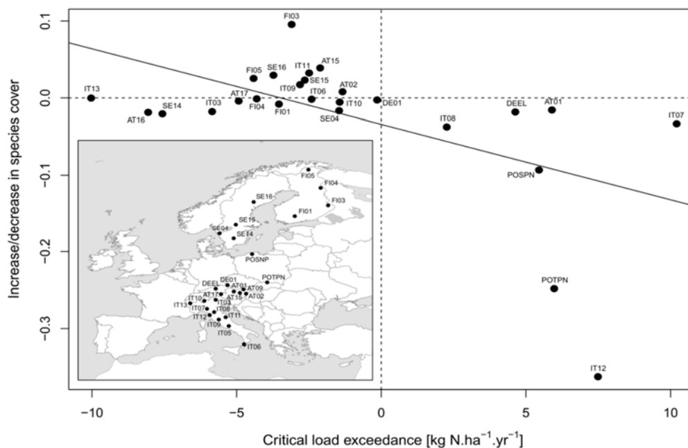
Figure 27: Forest plant species that prefer low soil nutrient levels have decreased during the last 10-50 years in 28 ICP IM and ICP Forests sites across Europe owing to the exceedance of the nitrogen critical loads. The y-axis indicates the strength of the cover change of all oligotrophic species in a study site (negative: decrease, positive: increase). The critical load exceedances are shown as the difference between the N deposition and the empirical critical load (negative values: no exceedance, positive values: exceedance) (based on Dirnböck et al. 2014).
