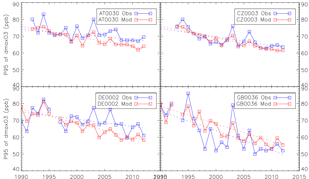
Figure 33: Observed and modelled trends in the annual 95-percentile of daily maximum ozone concentrations 1990-2012 for four EMEP sites. The dotted lines show the significant Sen's slope ( p < 0.05 ) for the observed and modelled values, respectively. AT0030: Austria, Pillersdorf bei Retz; CZ0003: Czech Republic, Kosetice; DE0002: Germany, Waldhof; GB0036: United Kingdom, Harwell.
