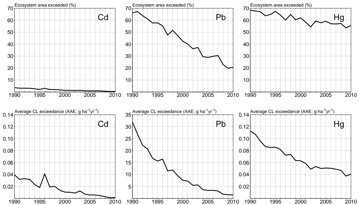
Figure 60: Temporal development of the area (top; % of ecosystem area) where critical loads of cadmium (left), lead (centre) and mercury (right) are exceeded and the magnitudes of the average accumulated exceedance (AAE) (bottom; g ha -1 yr -1 ) of the critical loads of these metals, respectively (Deposition data from EMEP-MSCE; critical loads data from the CCE).
