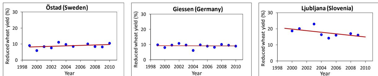
Figure 38: Reduction (%) in wheat yield due to ozone fluxes in recent years compared to pre-industrial ozone fluxes of a POD 3 IAM of zero (corresponding to ozone concentrations in the range of 10 – 15 ppb), assuming no soil water limitation. No significant trends were found.
