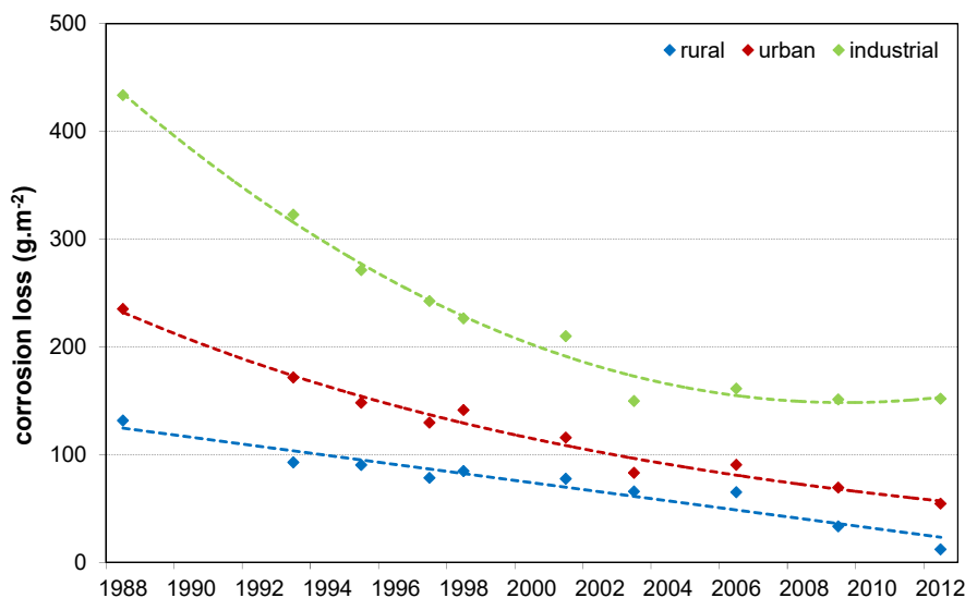
Figure 22: Trends in carbon steel yearly corrosion loss based on results from 20 test sites.
