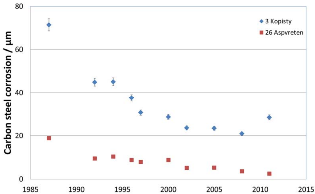
Figure 21: Trends in corrosion of carbon steel at two selected test sites.
