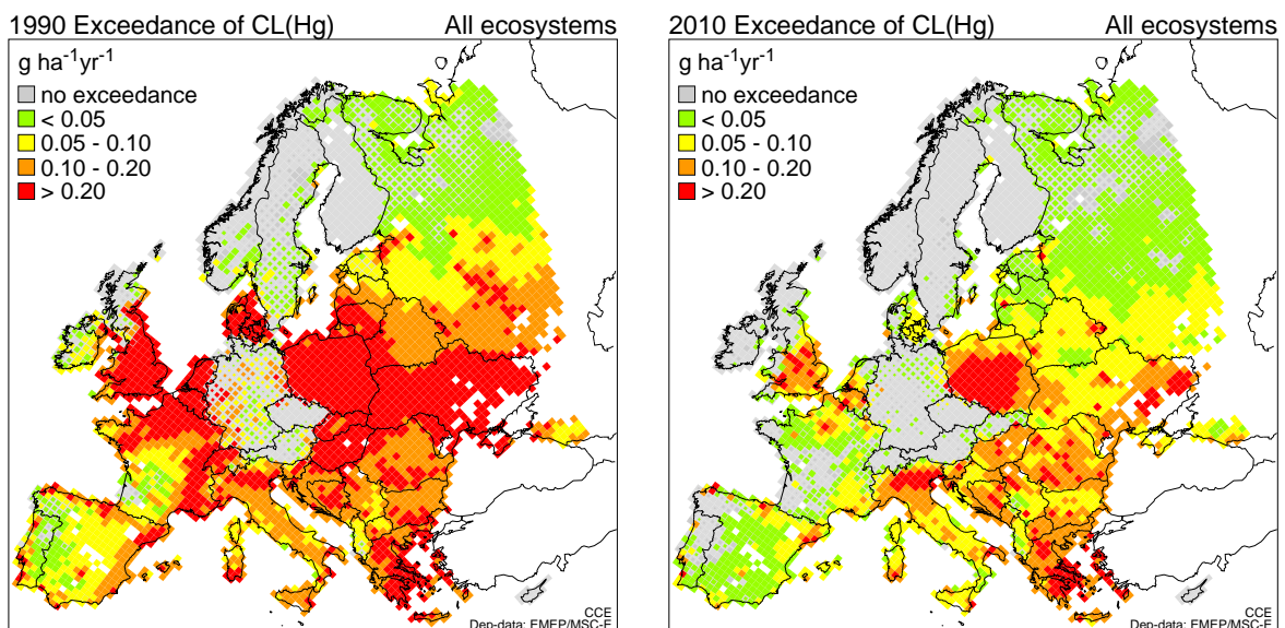
Figure 59: Exceedances (AAE) of the critical loads of mercury in 1990 (left) and 2010 (right) in Europe Note that the size of the colour shading in a grid cell indicates the % of the ecosystem area at risk. The ecosystem area can vary widely among grid cells. (Deposition data from EMEP-MSCE; critical loads data from the CCE).
