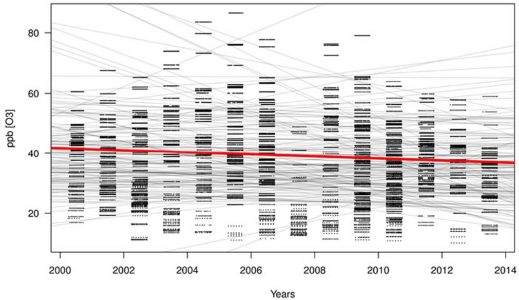
Figure 36: Mean ozone concentrations (April – September) from passive sampling from 203 plots nearby forests in 20 countries from 2000-2013, showing a significant decline of 0.35 ppb y -1 (n = 29,356; p = 0.000).
