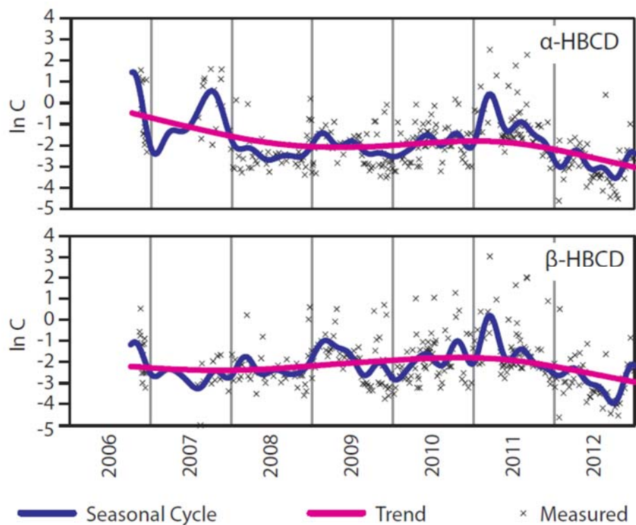
Figure 65: Air concentrations of \alpha - and \beta -HBCD at Zeppelin (Source: AMAP, 2014)
