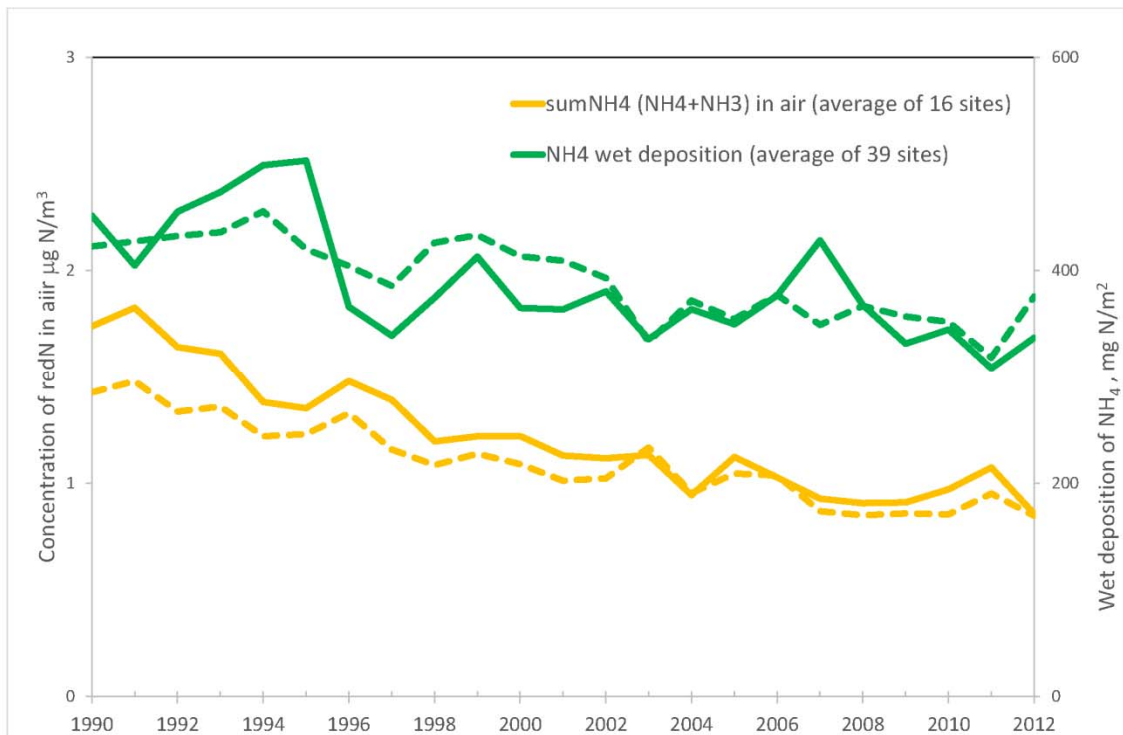
Figure 12: The observed and modelled annual average concentrations in reduced nitrogen components in air and wet deposition at EMEP sites with measurements for at least 75% of the time period, 1990-2012. Solid lines are observations while the dotted lines are EMEP model results for the same sites.
