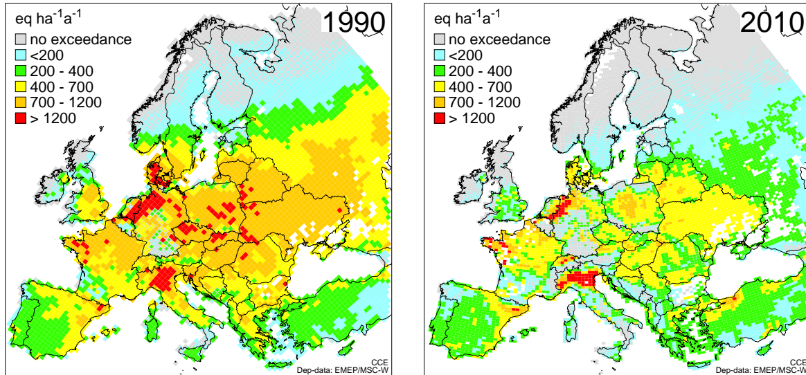
Figure 31: Exceedances (AAE) of the critical loads of nutrient N in 1990 (left) and 2010 (right) in Europe. Note that the size of the colour shading in a grid cell indicates the % of the ecosystem area at risk. The ecosystem area can vary widely among grid cells. (Deposition data from MSC-W; European critical loads data from the CCE).
