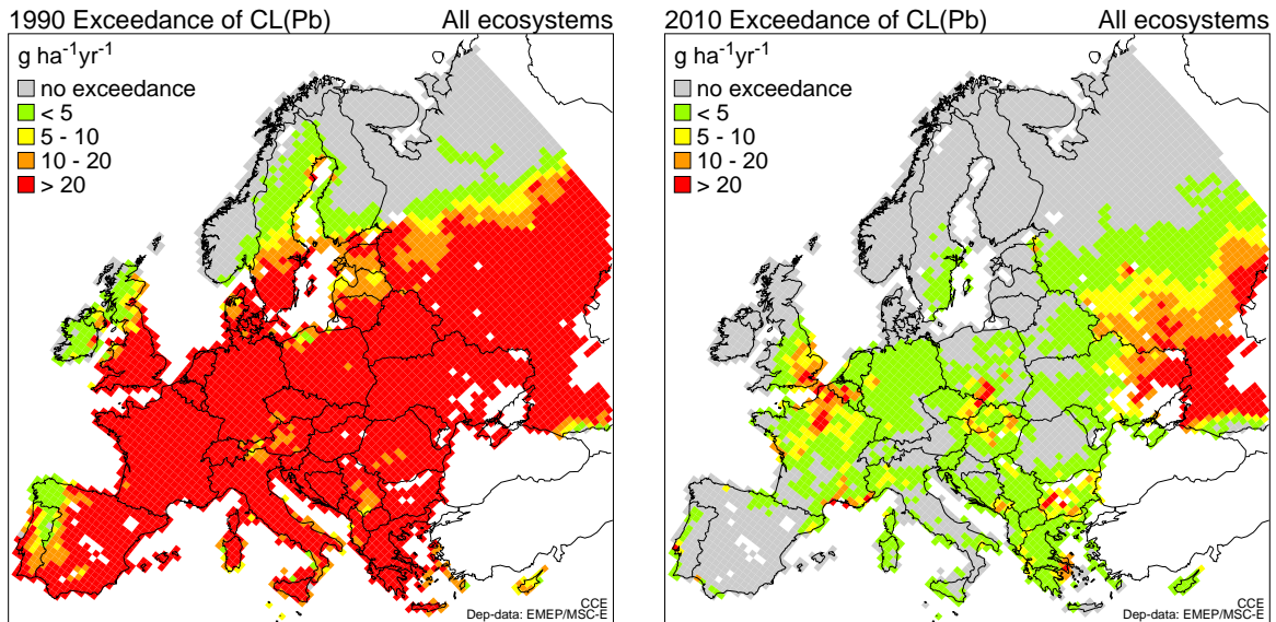
Figure 58: Exceedances (AAE) of the critical loads of lead in 1990 (left) and 2010 (right) in Europe . Note that the size of the colour shading in a grid cell indicates the % of the ecosystem area at risk. The ecosystem area can vary widely among grid cells. (Deposition data from EMEP-MSCE; critical loads data from the CCE).
