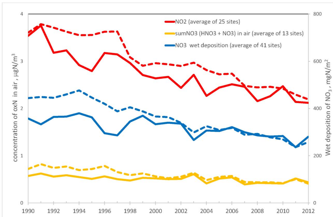
Figure 11: The observed and modelled annual average concentration in oxidized nitrogen components in air and wet deposition at EMEP sites with measurements for at least 75% of the time period, 1990-2012. Solid lines are observations while the dotted lines are EMEP model results for the same sites.
