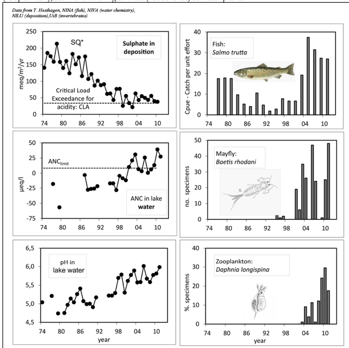
Figure 19: Biological recovery – an example from Norway. Recovery from acidification at Lake Saudlandsvatn, Norway. As sulphur deposition has decreased, the acid neutralising capacity (ANC) and pH have increased in the lake, and the populations of three sensitive species, i.e. brown trout, the mayfly Baetis rhodani and the planktonic crustacean Daphnia longispina have begun to recover (modified from Hesthagen et al. 2011 Sci Tot Env).
