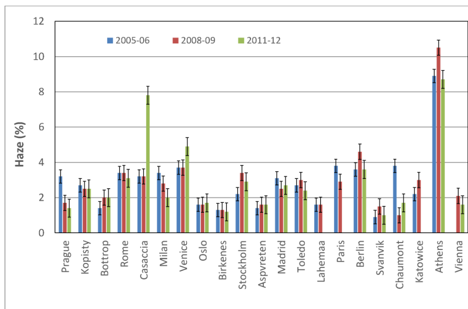
Figure 47: Comparison of haze (in %) during the three extensive campaigns (2005-2006; 2008-2009; 2011-2012).
