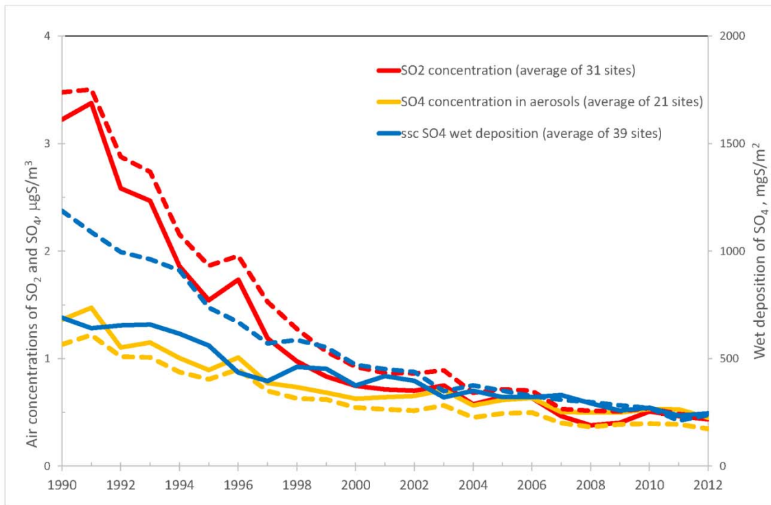
Figure 10: The observed and modelled annual average concentration in sulphur components in air and wet deposition at EMEP sites with measurements for at least 75% of the time period, 1990-2012. Solid lines are observations while the dotted lines are EMEP model results for the same sites.
