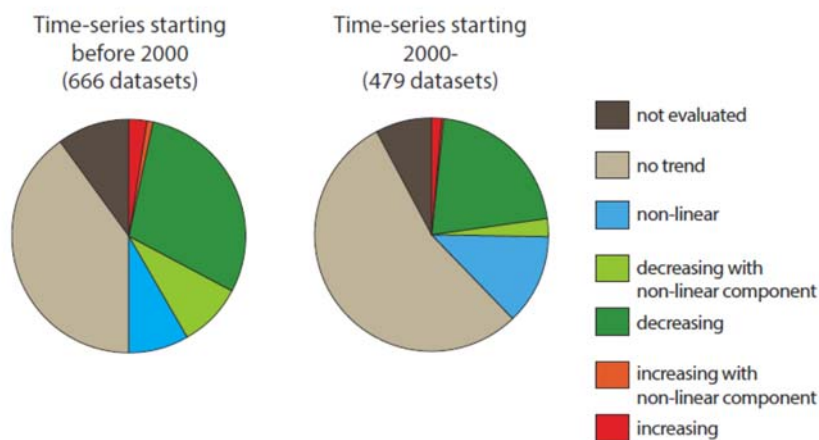
Figure 66 Aggregated results of statistical analyses of time-series of POPs in Arctic biota for entire time-series (left) and time-series since 2000 (right) (Source: AMAP, 2014).
