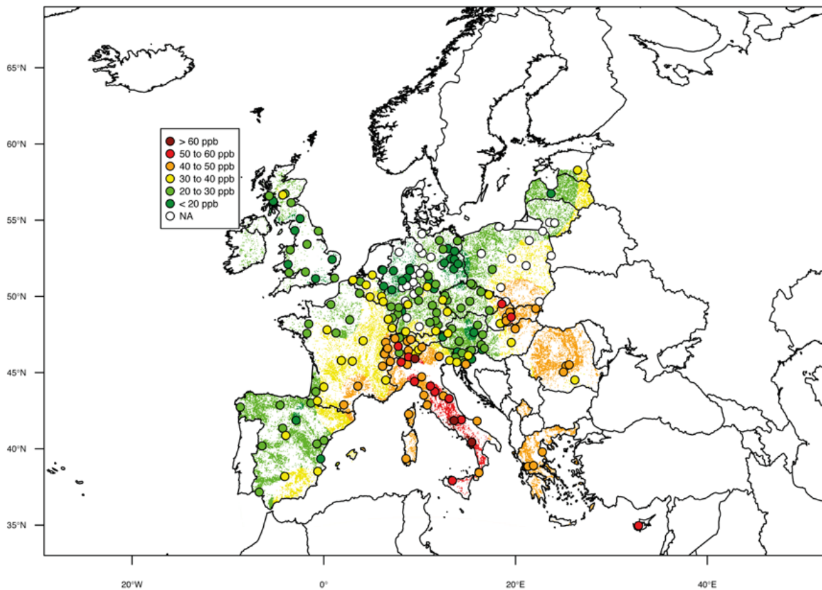
Figure 35: Mean O 3 concentration classes (April – September) from passive samplers on 203 rural forest level II plots during 2000-2013.
