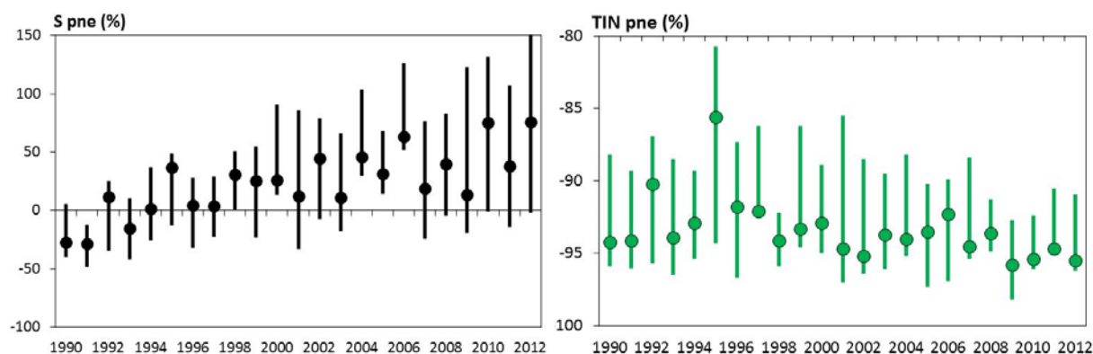
Figure 17: Percentiles (25%, median 50%, 75%) of percent net export (pne, %) of sulphate (SO 4 )(left) and total inorganic nitrogen (TIN) (right) for 8 IM sites in 1990-2012.
