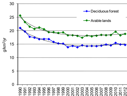
Figure 2: Trends of B[a]P deposition to deciduous forest and arable lands within the EMEP region (Source: Gusev et al., 2015).
