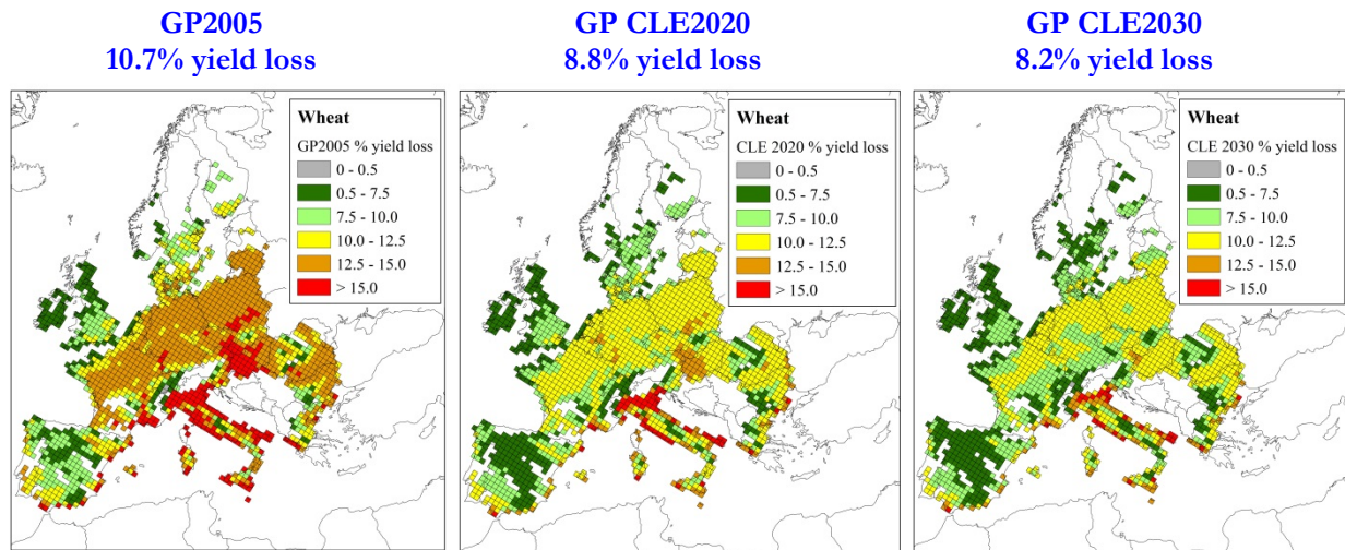
Figure 39: Calculated percentage yield losses due to ozone effects on wheat per 50 km x 50 km EMEP grid square in 2005, 2020 and 2030 for the wheat growing areas of the EU27+CH+NO for the base year (2005) of the revised Gothenburg Protocol (GP) and with implementation of its current legislation (CLE) for 2020 and 2030. The percentage yield loss was calculated using the generic ozone flux model for application in integrated assessment modelling (POD 3 IAM; LRTAP Convention, 2015).
