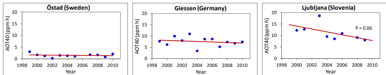
Figure 37: Trend in AOT40 at three selected sites in Europe. A significant trend ( P = 0.06 ), a decline of 0.6 ppm h per year, was found only in Ljubljana (Slovenia).
