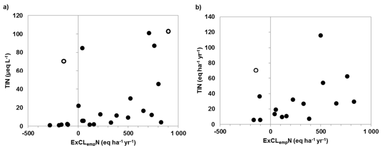
Figure 30: Eutrophication empirical impact indicators in relation to exceedance of critical loads of N at ICP IM sites. The x-axes show exceedances of empirical critical loads of nutrient N ( ExCL_{emp}N , NAT2000 deposition). The y-axes show annual mean concentrations (a) and fluxes (b) of TIN (NO 3 + NH 4 ) in runoff. Negative exceedance values indicate that the critical loads are not exceeded. Open circles indicate catchments with inputs of N from sources other than deposition. TIN flux for site DE01 (1373 eq ha -1 yr -1 ) is outside axis range and not shown in graphs (based on Holmberg et al. 2013).
