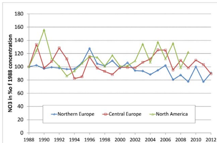
Figure 29: Trends in surface water chemistry at ICP Waters sites 1988-2012. Shown are the mean concentrations of \text{NO}_3 at 22 sites in northern Europe, 21 sites in central Europe and 37 sites in eastern North America (for 2010-2012, no data available for North America). (Source: Garmo et al. 2015).
