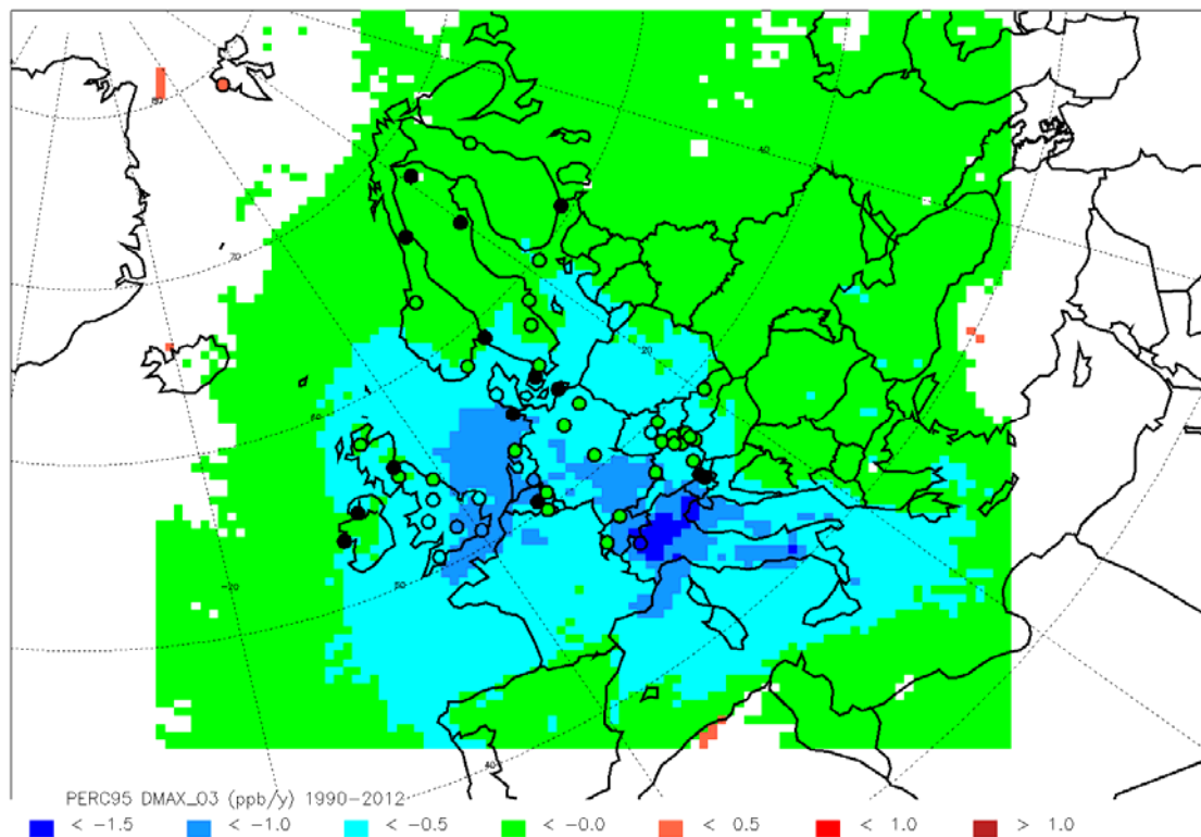
Figure 34: Sen's slopes (ppb year -1 ) of the modelled annual 95 percentiles of the daily maximum ozone concentration for the period 1990–2012 with the results from EMEP monitoring data on top (circles). The colors indicate the magnitude of the trend. Filled, black circles indicate non-significant slopes. Note that the significance criteria for the stations were changed from p=0.05 to p=0.2 in this plot.
