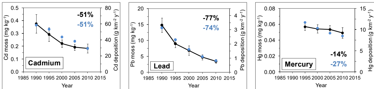
Figure 52: Average median metal concentration ( \pm one standard error) in mosses for countries that reported metal data for at least four survey years since 1990; some countries reported three survey years since 1995 for mercury (Harmens et al. 2015). The blue dots in the graphs show the decline in deposition across Europe as modelled by EMEP (Travnikov et al. 2012). The black and blue values in the graphs represent the percentage change (i.e. a decline) between 1990 (1995 for mercury) and 2010 for the moss concentrations and EMEP modelled depositions respectively.
