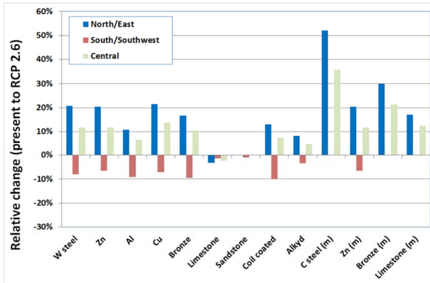
Figure 24: Calculated relative changes in corrosion due to SO 2 for the IPCC RCP2.6 scenario. Calculations are based on dose-response functions for the SO 2 dominating situation for most materials and dose-response functions for the multi-pollutant situation, indicated by (m).
