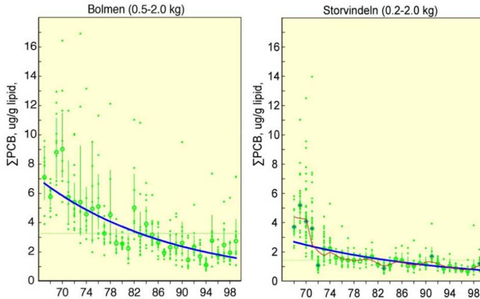
Figure 69: Example of two time series of PCBs in pike muscle ( \mu\text{g/g lipid} ) from Lake Bolmen (southern Sweden) and Lake Storvindelen (northern Sweden) for the years 1967/1968 - 1999. Source: Fjeld et al. 2005; Nyberg et al. 2014.
