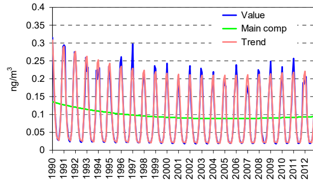
Figure 3: Trend of monthly mean B[a]P air concentrations in the EMEP region for the period from 1990 to 2012.
