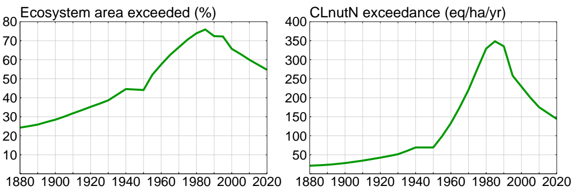
Figure 32: Temporal development of the area in Europe where nutrient N critical loads are exceeded (left; % of ecosystem area) and average accumulated exceedance (AAE) (right; eq ha -1 yr -1 ) of nutrient N critical loads (all ecosystems). Future exceedances are based on the implementation of agreed legislation. (Emission and deposition data from EMEP-CIAM and EMEP- MSC-W; critical loads data from the CCE).
