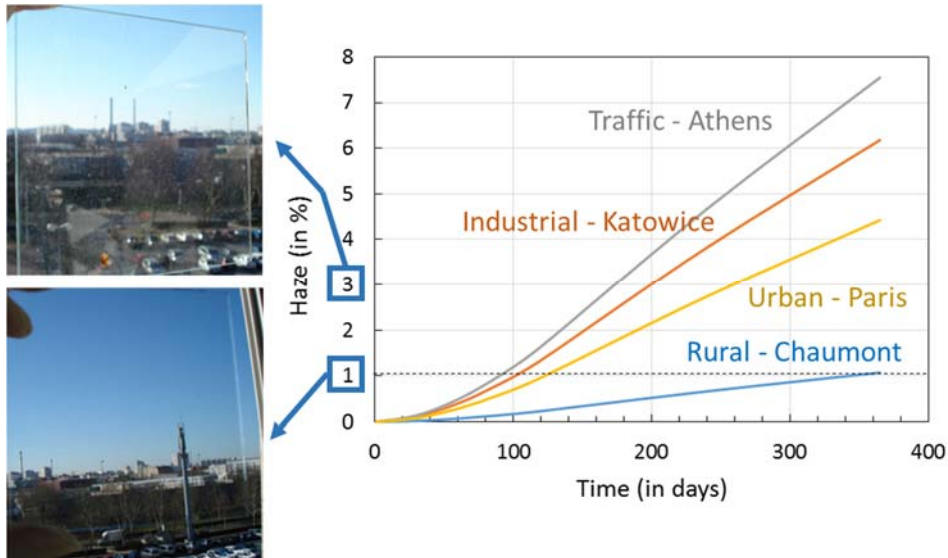
Figure 48: Predicted haze (in %) as a function of time for 4 types of sites: rural, urban, industrial and traffic. Input environmental data for the 2008-2009 campaigns were selected (Lombardo et al. 2014). Visual aspects are shown on 2 pictures: Katowice after 1 year (haze = 3%), upper image and Chaumont (haze = 1%), lower image.
