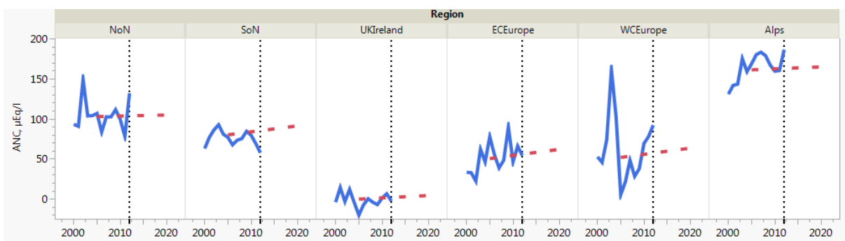
Figure 20: Observed mean (blue) and modelled (red) acid neutralizing capacity (ANC) in European regions between 2000 and 2020. Regions are northern Nordic (NoN), southern Nordic (SoN), the UK and Ireland, East-Central Europe (EC Europe), West-Central Europe (WC Europe) and the Alps (see also 2.7).
