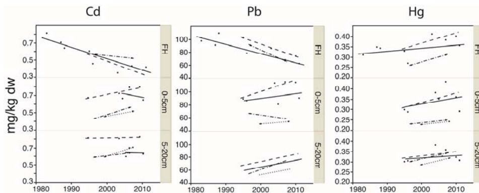
Figure 54: Soil metal concentrations at the four ICP IM sites in Sweden (Aneboda (solid line) , Gammtratten (dotted line), Gårdsjön (dashed line), Kindla (dotdashed line)).
