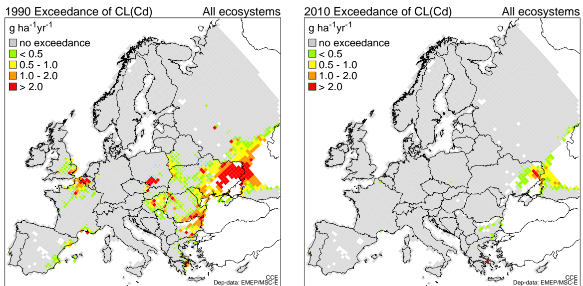
Figure 57: Exceedances (AAE) of the critical loads of cadmium in 1990 (left) and 2010 (right) in Europe. Note that the size of the colour shading in a grid cell indicates the % of the ecosystem area at risk. The ecosystem area can vary widely among grid cells. (Deposition data from EMEP-MSCE; critical loads data from the CCE).
