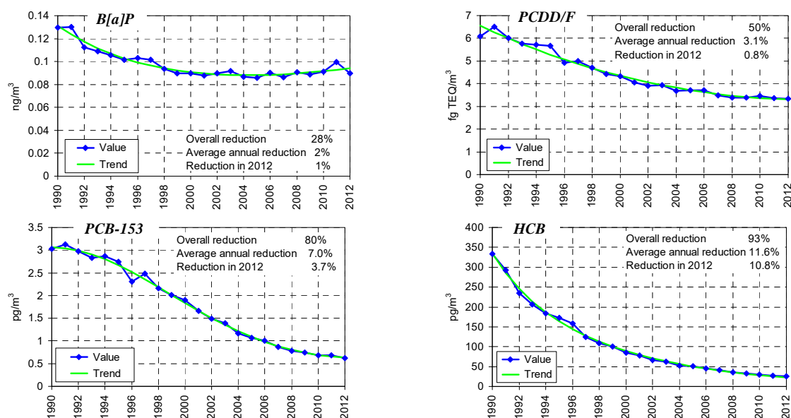
Figure 61: Trends in annual mean air concentrations of (a) B[a]P, (b) PCDD/Fs, (c) PCB-153 and (d) HCB in the EMEP region for the period from 1990 to 2012. Negative reduction denotes increase of air concentrations. Green line indicates estimated trend and blue line – annual mean air concentrations. Reduction rates refer to main trend component. (Source: Gusev et al. 2015).
