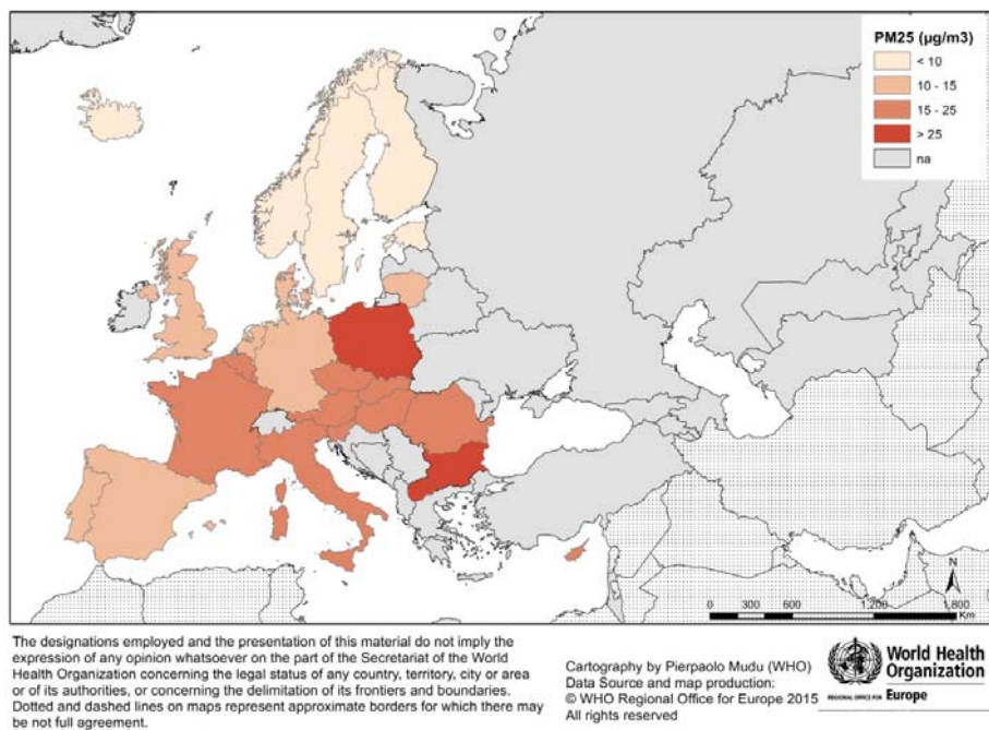
Figure 44: Population weighted annual mean PM2.5, for 2012 or the last year available.
