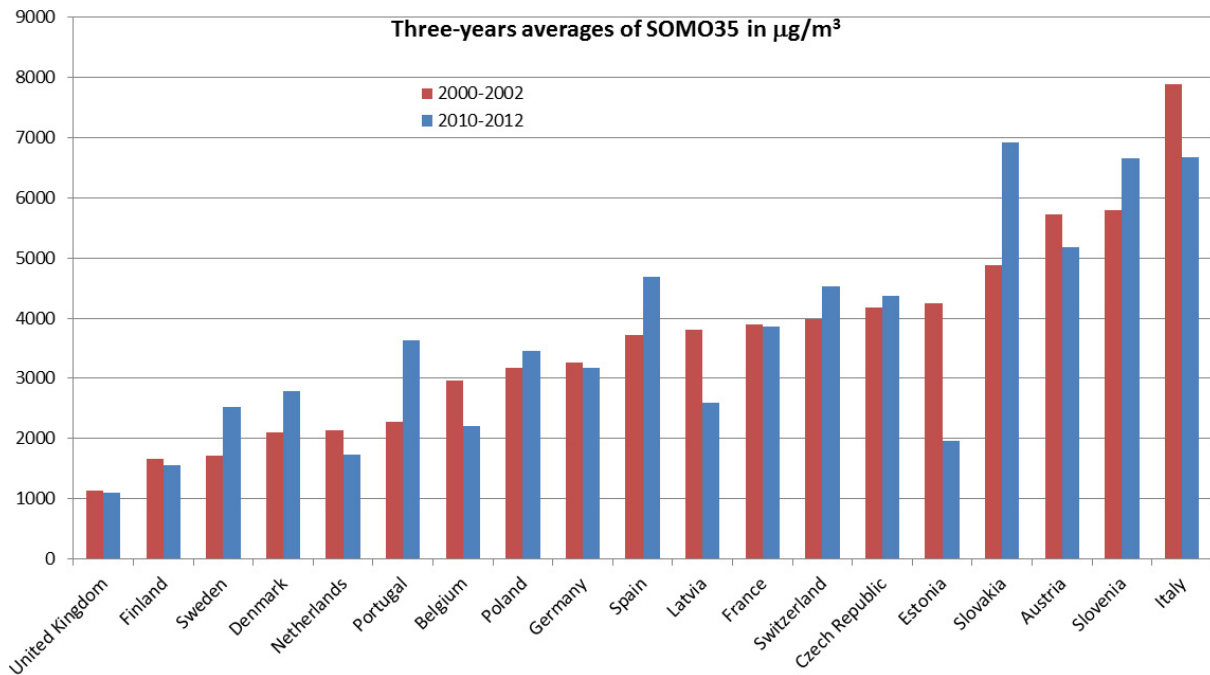
Figure 41: Population weighted annual mean SOMO35, three-year averages, for 2000-2002 and 2010-2012.
