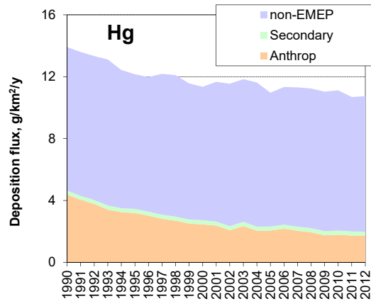
Figure 50: Mercury deposition fluxes caused by anthropogenic and secondary sources within EMEP region and by non-EMEP sources.
