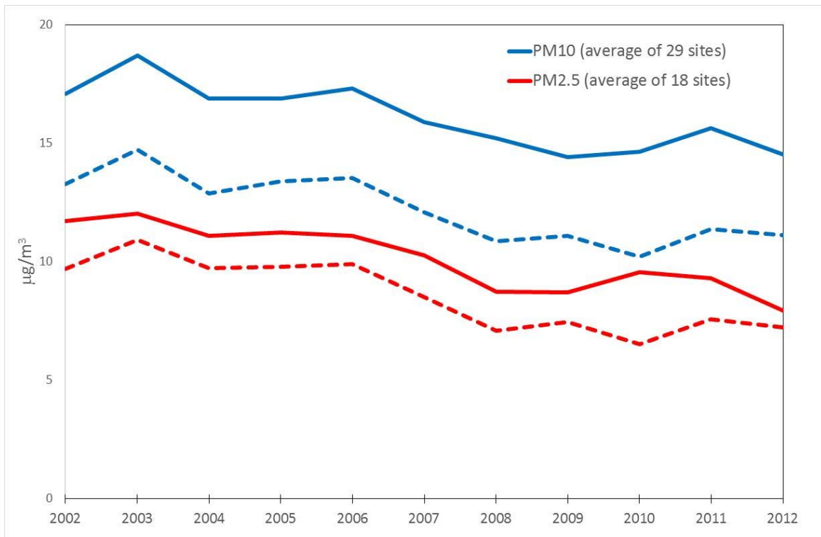
Figure 42: The observed and modelled annual average concentrations in PM 10 and PM 2.5 at EMEP sites with measurements for at least 75% of the time period, 2002-2012. Solid lines are observations while the dotted lines are EMEP model results for the same sites.
