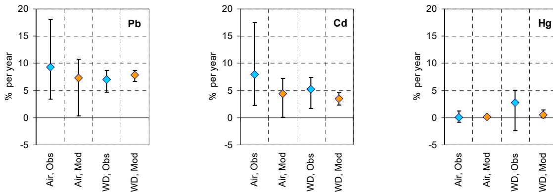
Figure 51: Mean annual reduction rates for modelled and observed air concentrations and wet deposition fluxes of lead (left), cadmium (middle) and mercury (right) over selected EMEP monitoring stations. Whiskers span the mean range of average reduction rates among stations.
