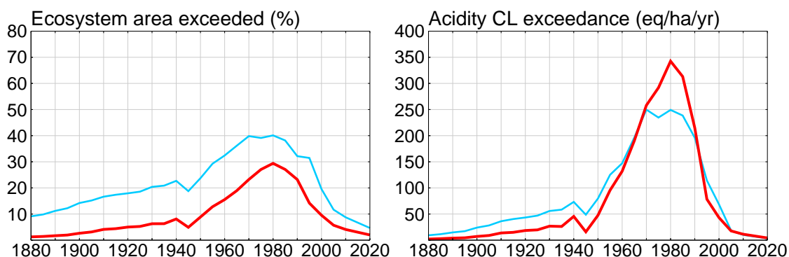
Figure 26: Temporal development of the area in Europe where acidity critical loads are exceeded (left; % of ecosystem area) and average accumulated exceedance (AAE) (right; eq ha -1 yr -1 ) of critical loads of acidity (red: all ecosystems, blue: surface waters). Future exceedances are based on the implementation of agreed legislation (emission and deposition data from EMEP-CIAM and EMEP- MSC-W; critical loads data from the CCE).
