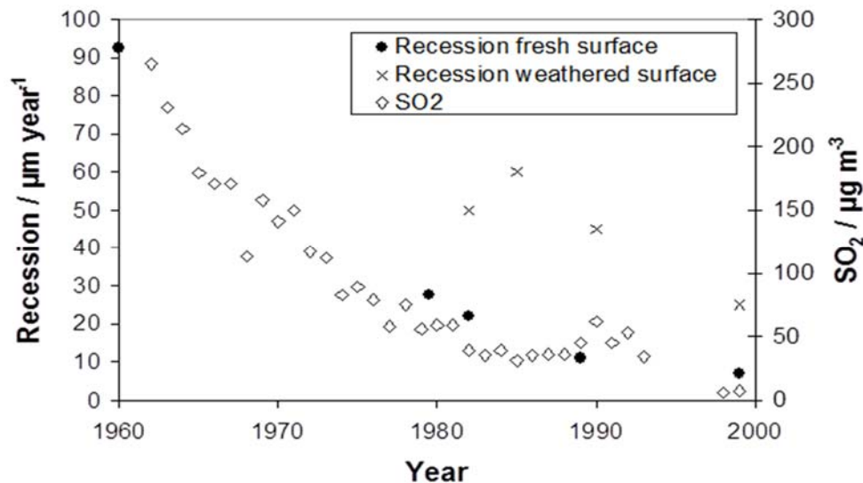
Figure 23: Surface recession rates of limestone and \text{SO}_2 concentration at St Paul's Cathedral. The surface recession of fresh surfaces is measured on standard samples while recession on weathered surfaces is measured on the actual building using micro-erosion meters.
