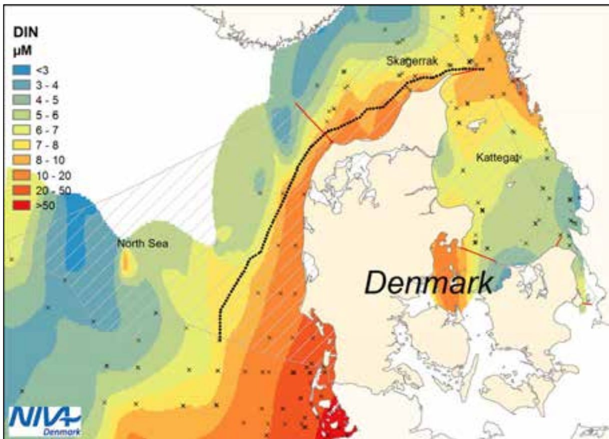
Figure D.4: Interpolated average surface (0-5m) DIN concentrations [ \mu\text{mol l}^{-1} ] for winter (Dec, Jan, Feb) 2006-2013, showing locations of sampling stations (x). The heavy dotted black line indicates the boundary for Non-Problem and Problem Areas, as determined by analysis of EO chlorophyll a measurements.
