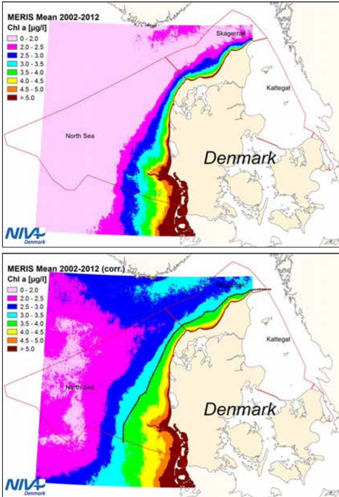
Figure C.3: MERIS Chlorophyll a Concentrations, averaged for the period 2002-2012, Top: uncorrected, Bottom: corrected using the function Cbl_{corr} = 2.14 * Cbl_{MERIS}^{0.515} . The black dotted line in the bottom figure indicates the boundary of the region where Chlorophylla concentration does not exceed 3.5 \mu\text{g l}^{-1} .
