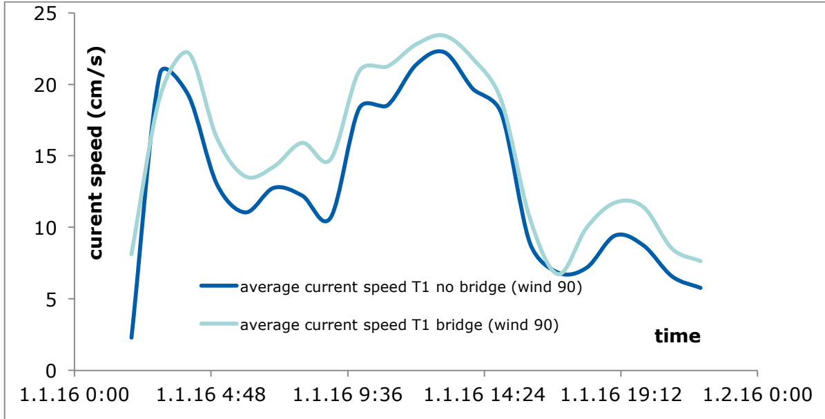
Figure 5.11 Averaged current speed for T1 (outside the bridge) for east wind before and after constructing the bridge.
