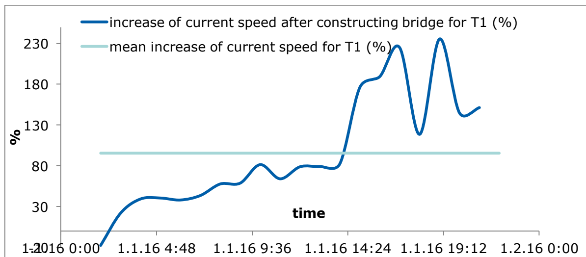
Figure 5.21 Percentage increase of averaged current speed for T1 for the north wind after constructing the bridge.
