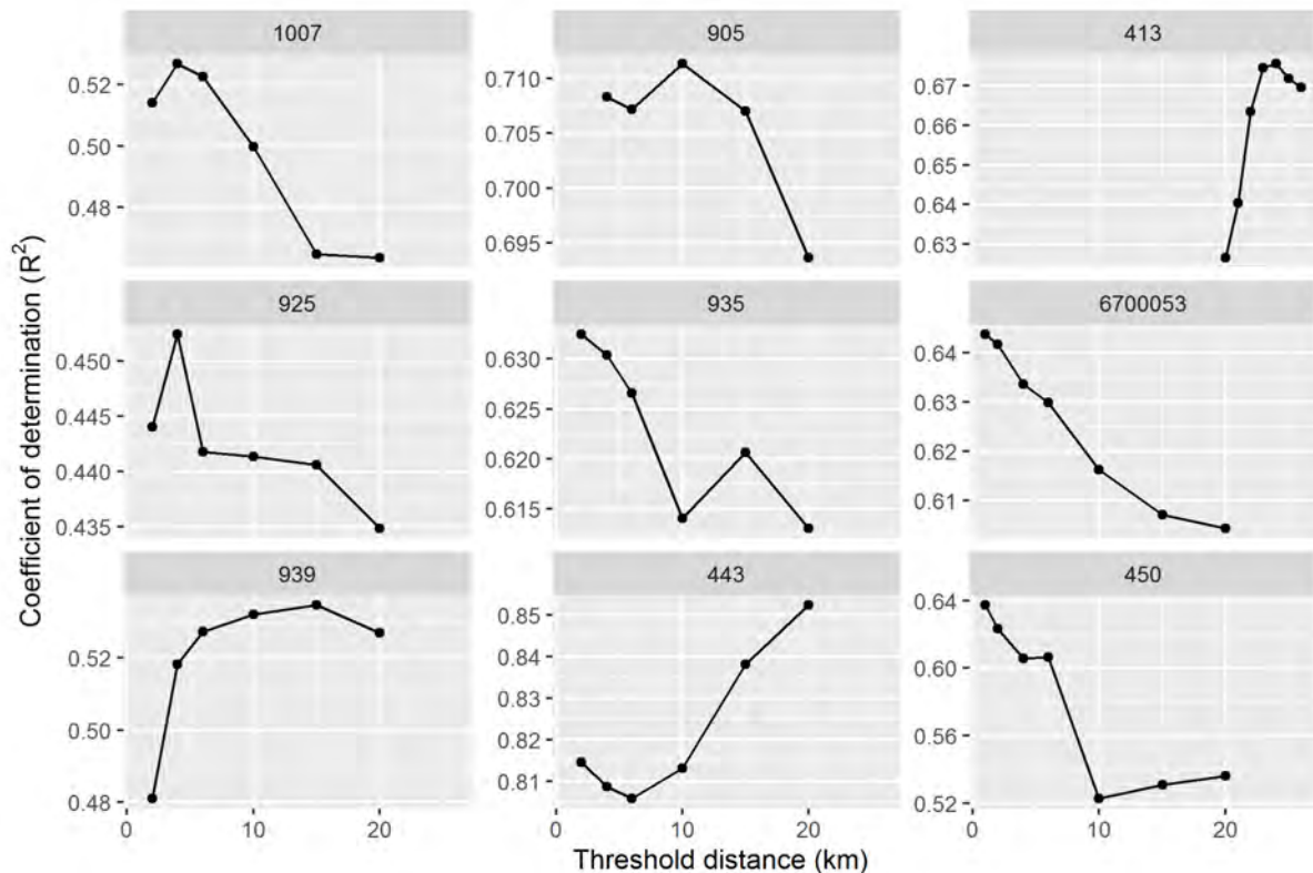
Figure 3.1 Selecting optimal threshold distance ( r ) for selecting Ferrybox data close to oceanographic stations (sorted from north to south). The graph shows the fit of a regression between station-based chlorophyll- a measurements and median Ferrybox chlorophyll- a estimates, as measured by the coefficient of determination ( R^2 ).
