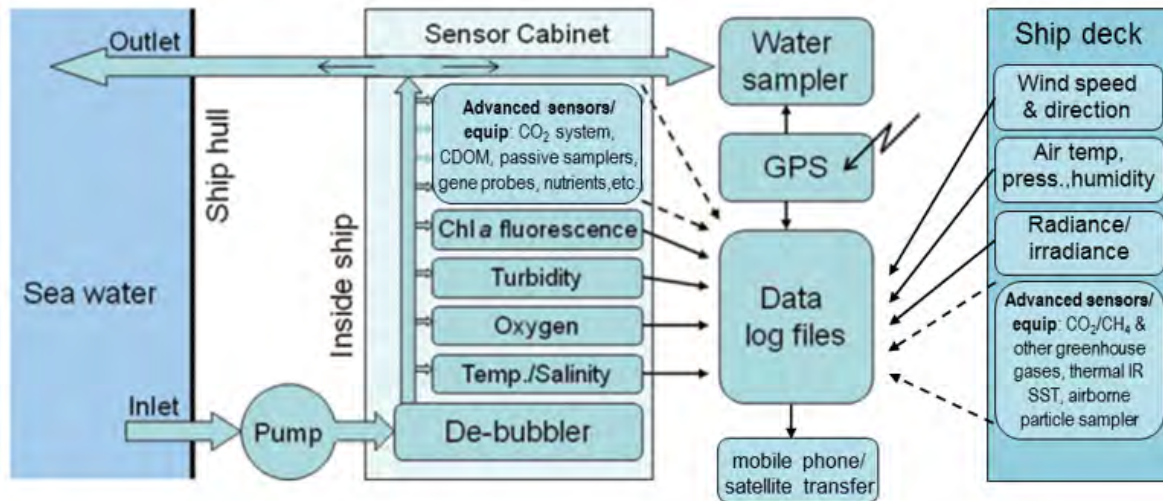
Figure 2.1 An example of an autonomous Ferrybox system that includes a seawater pump, pipes, sensors, water sampler, and data logging hardware/software. Figure is adapted from Volent et al. (2011).
