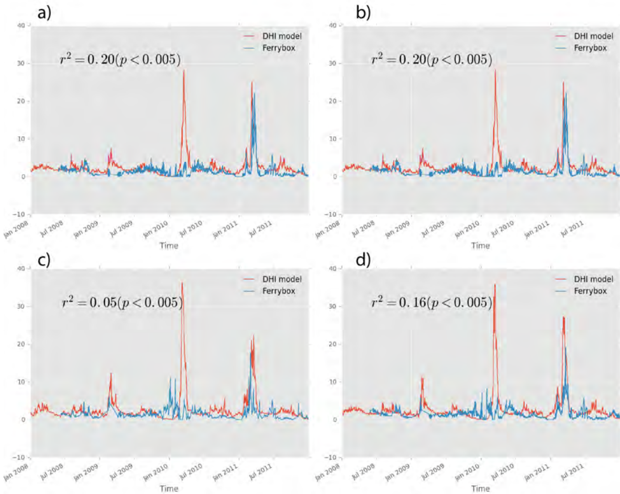
Figure A1.1 Comparison between chlorophyll-a from Ferrybox observations and ocean model (DHI) from selected stations a) 935, b) 939 c) 1007, and d) 925. Ferrybox data measured within a 5-km radius of the geographical position for each station were extracted and plotted. Correlations between model and Ferrybox were calculated using Pearson's linear correlation algorithm. Data from station N3 and 6700053 for 5 km radius was not available.
