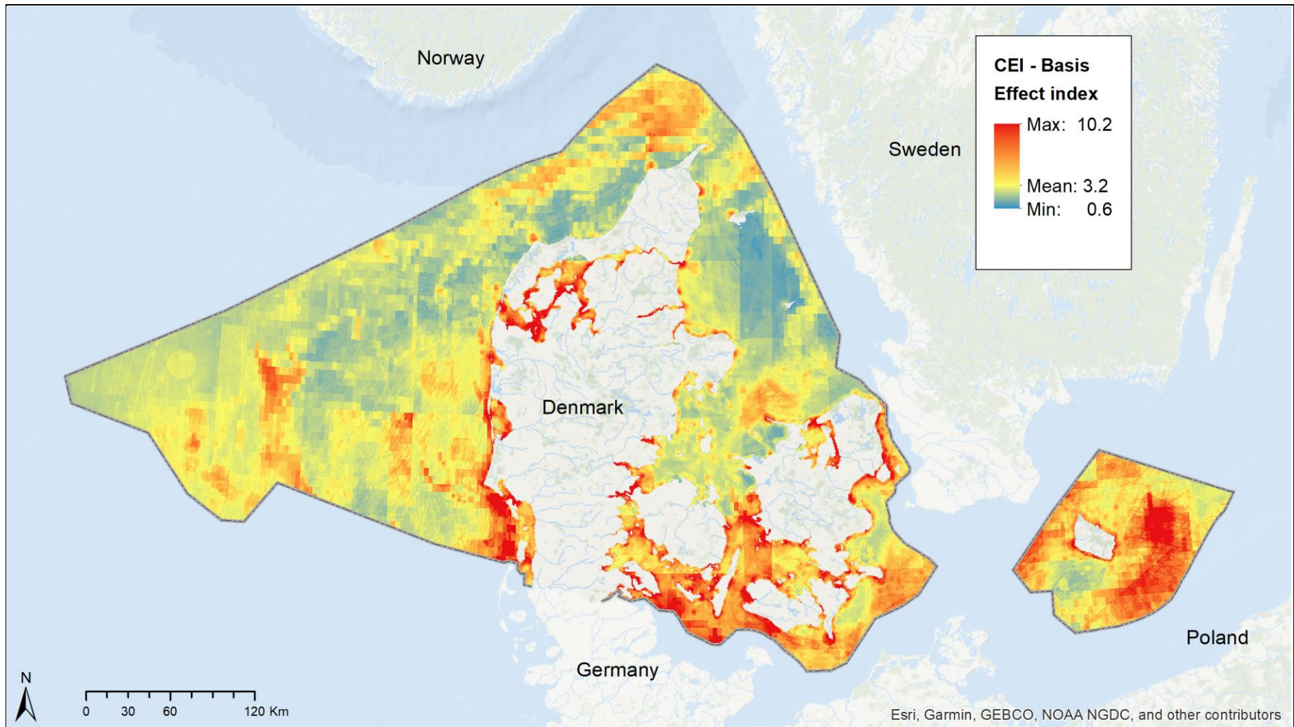
Figure 6: Map of intensities and spatial variations in the estimated combined effects of human pressures and activities including climate change. The colour scale shows the stretch for 2.5 standard deviations from the mean, where red indicates a higher effect impact and blue lower. Please note that the values are unit less and that the magnitude is defined by the models data inputs, which here are normalised between 0-1. The index is calculated using EcolImpactMapper developed by Stock (2016).
