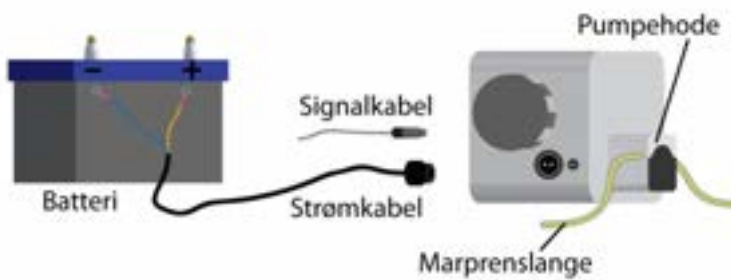
Figur 9. Pumpeoppsett.
