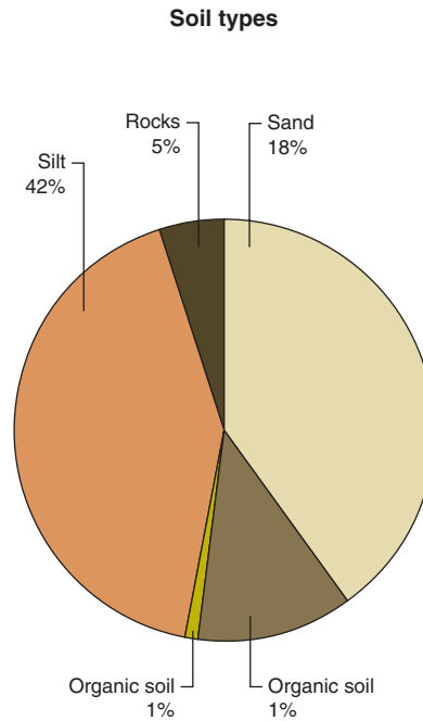
Figure 3: Main soil types in the Enza catchment.
