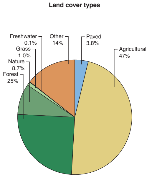
Figure 2: Main land use classes in the Enza catchment.
