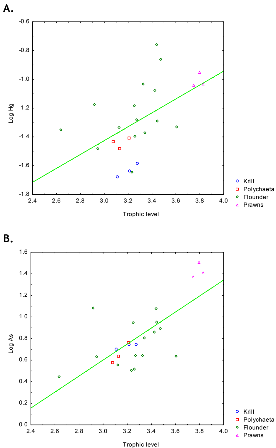
Figure 43. Trophic level against concentrations ( \mu\text{g/g} wet wt.; log-transformed) of mercury (A.) and arsenic (B.) in organisms of the Inner Oslofjord food web (herring gull excluded; R^2 = 0.28 and 0.50 , respectively, p = 0.007 and 0.0001 , respectively).
