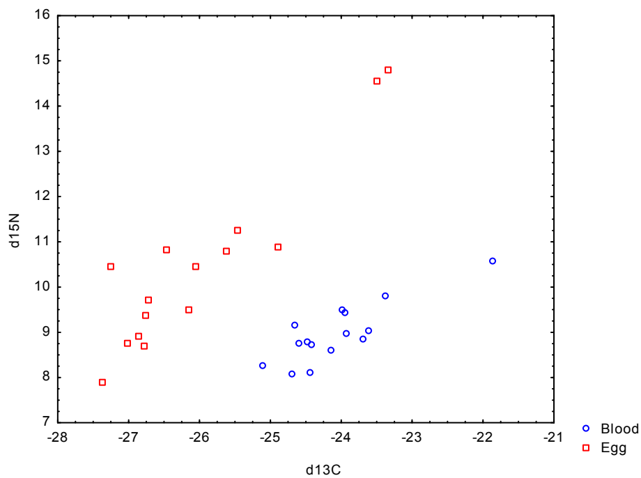
Figure 3. \delta^{13}C plotted against \delta^{15}N in organisms from the inner Oslofjord. (Herring gull = eggs; A.), and \delta^{13}C plotted against \delta^{15}N in herring gull blood and eggs (B.).
