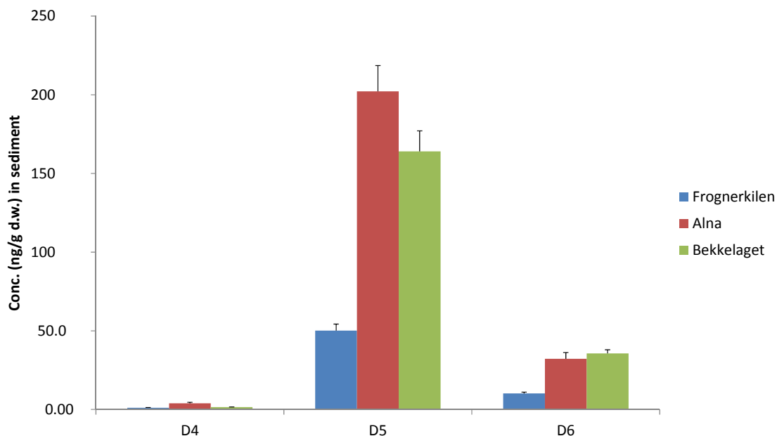
Figure 31. Concentrations of cyclic volatile methylsiloxanes (ng/g dry wt.) in sediments from Frognerkilen, the mouth of Alna River and at Bekkelaget (mean and standard deviation; n=3).
