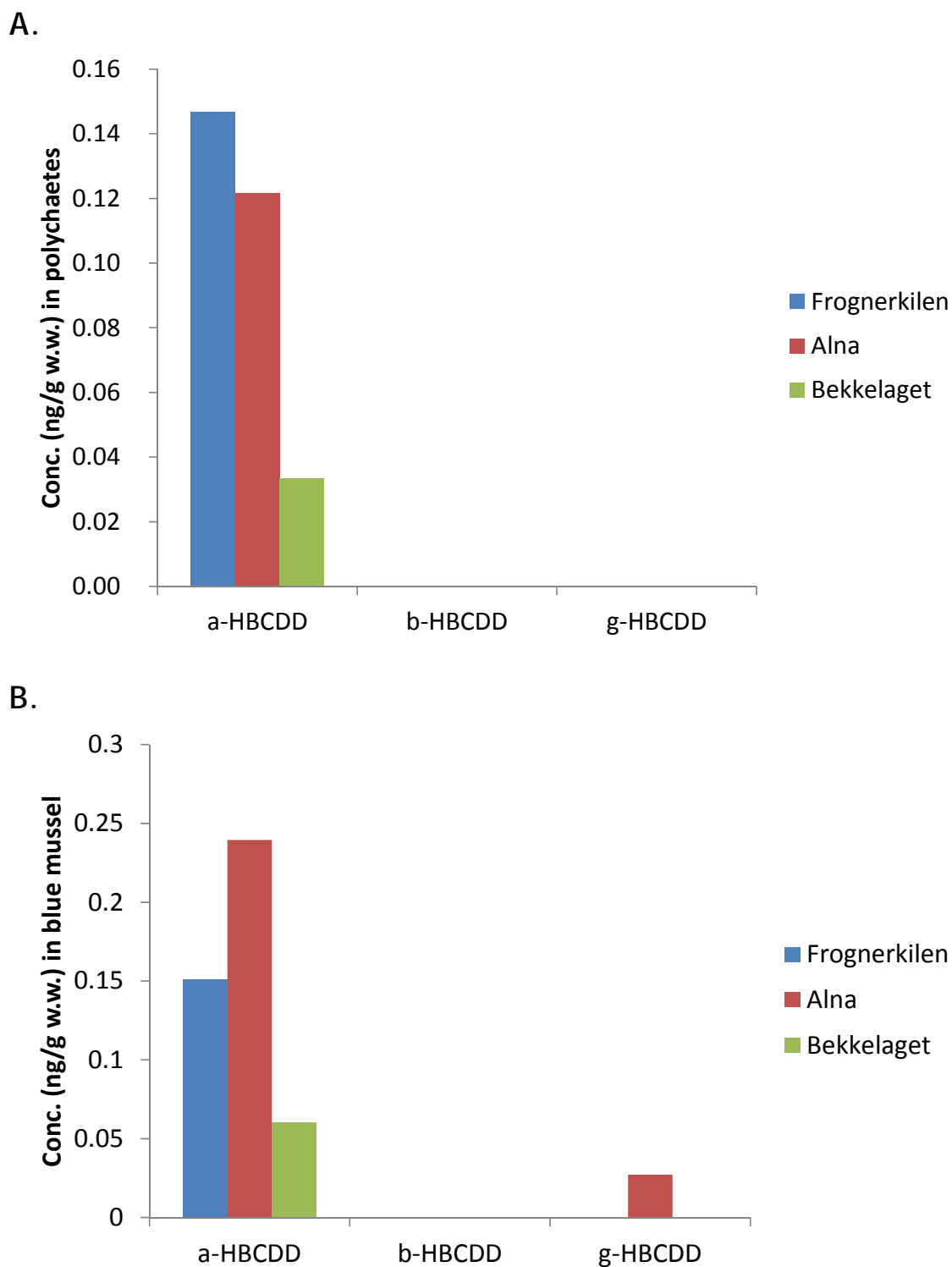
Figure 15. Concentrations of HBCDD stereoisomers (ng/g wet wt.) in polychaetes (A.) and blue mussel (B.) from Frognerkilen, the mouth of Alna River and at Bekkelaget. One composite sample per station.
