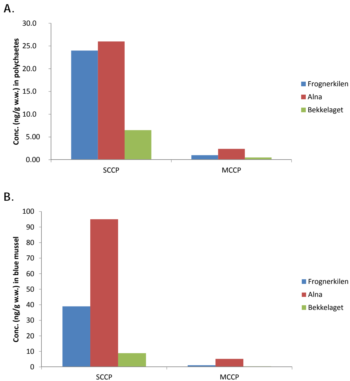
Figure 23. Concentrations of short and medium chained chloroparaffines (S/MCCPs; ng/g wet wt.) in polychaetes (A.) and blue mussel (B.) from Frognerkilen, the mouth of Alna River and at Bekkelaget. One composite sample per station.
