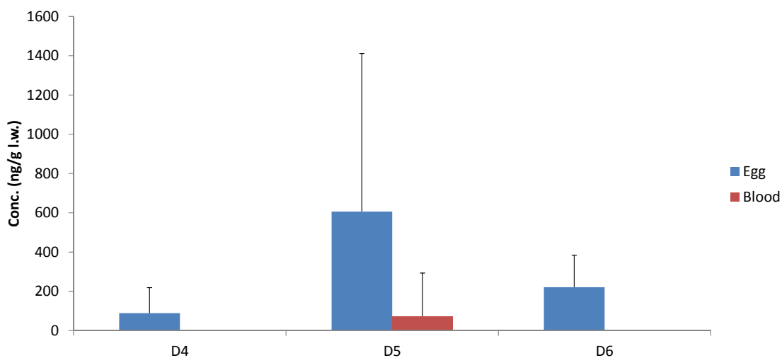
Figure 32. Concentrations of cyclic volatile methylsiloxanes (ng/g lipid wt.) in Herring gull (eggs and blood) from the Inner Oslofjord (mean and standard deviation; n=15; non-detects are assigned values of zero (relevant only for blood, where only D5 was detected in 2 of 15 samples)).
