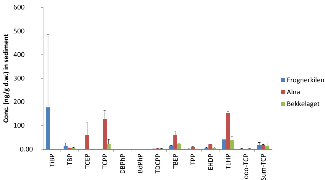
Figure 28. Concentrations of PFRs (ng/g dry wt.) in sediments from Frognerkilen, the mouth of Alna River and at Bekkelaget (mean and standard deviation; n=3; non-detects are assigned values of zero; TiBP was only detected in one sample from Frognerkilen; 531.9 ng/g dry wt.).
