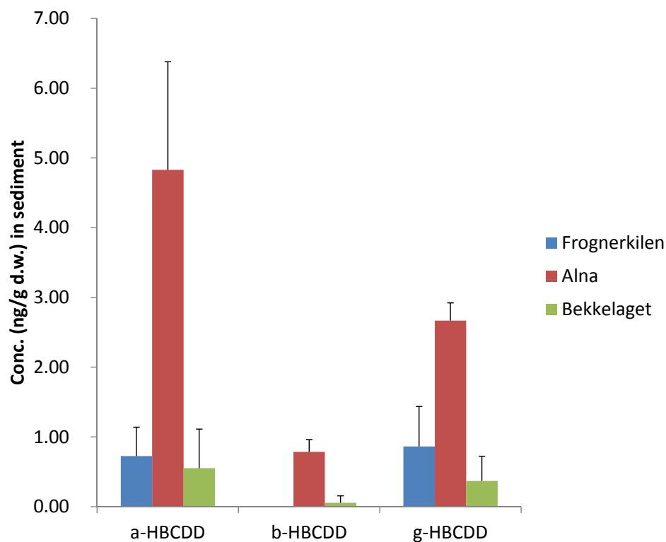
Figure 16. Concentrations of HBCDD stereoisomers (ng/g dry wt.) in sediments from Frognerkilen, the mouth of Alna River and at Bekkelaget (mean and standard deviation; n=3; non-detects are assigned values of zero).
