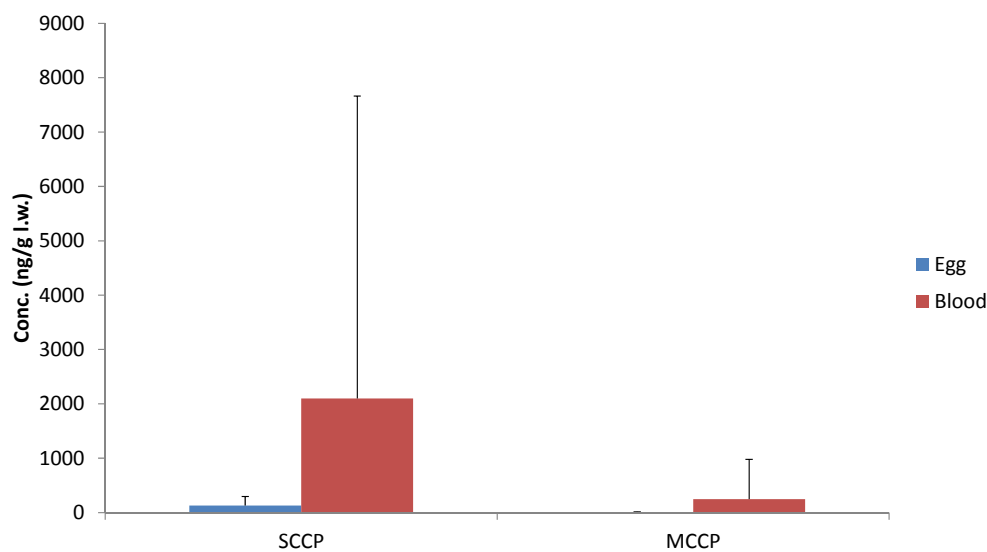
Figure 25. Concentrations of short and medium chained chloroparaffines (S/MCCPs; ng/g lipid wt.) in Herring gull (eggs and blood) from the Inner Oslofjord (mean and standard deviation; n=15; non-detects are assigned values of zero).
