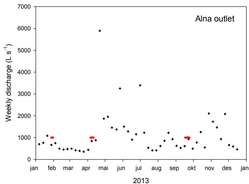
Figure 36. Weekly riverine discharge ( \text{L/s} ) of the Alna River with three continuous flow centrifugation sampling events superimposed (red horizontal lines).
