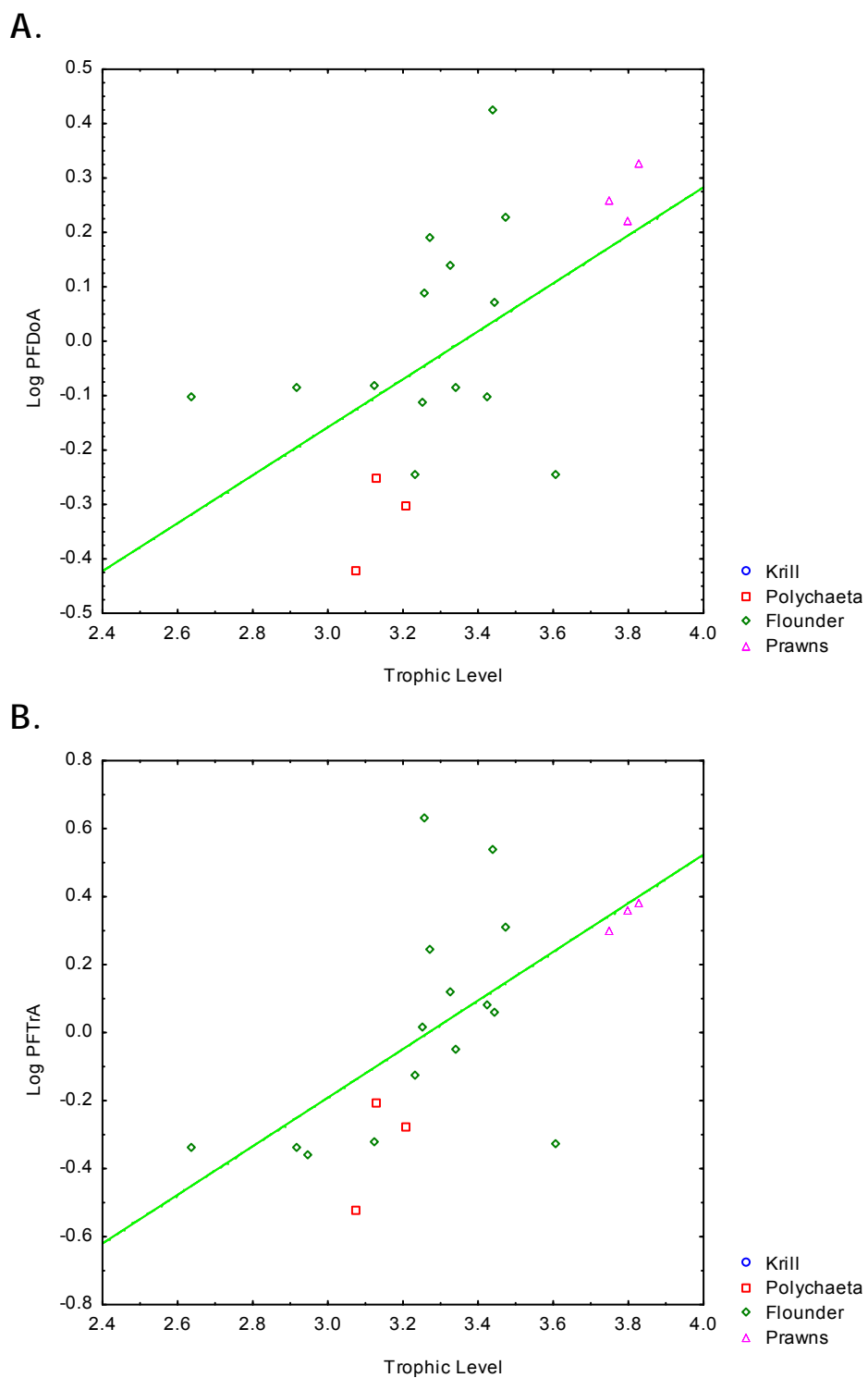
Figure 39. Trophic level against concentrations (ng/g wet wt.; log-transformed) of PFDoA (A.) and PFTrA (B.) in organisms of the Inner Oslofjord food web. Only concentrations above the LoD are included ( R^2=0.30 and 0.40 , respectively. p=0.01 and 0.002 , respectively).
