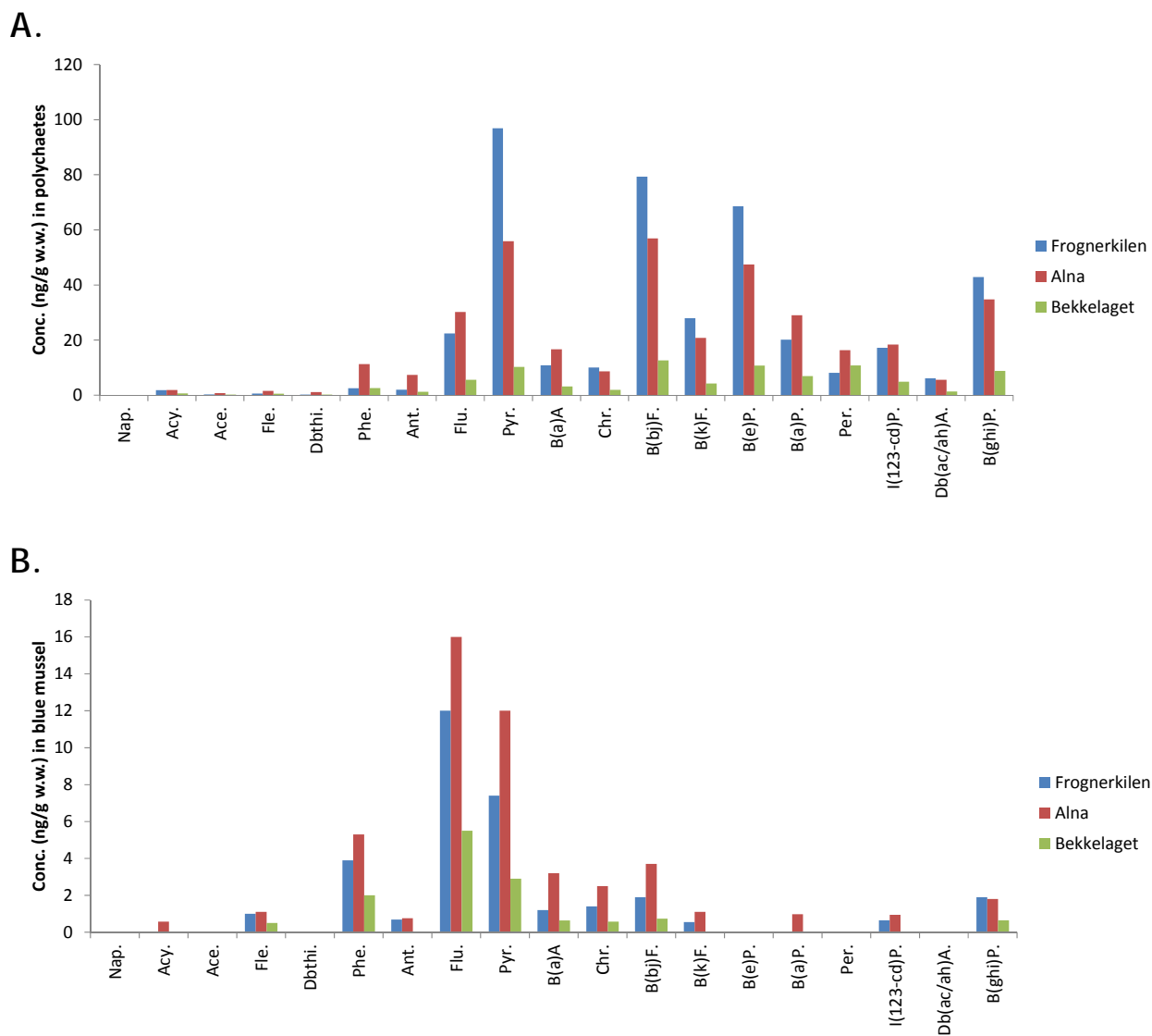
Figure 41. Concentrations of PAHs (ng/g wet wt.) in polychaetes (A.) and blue mussel (B.) from Frognerkilen, the mouth of Alna River and at Bekkelaget. One composite sample per station.
