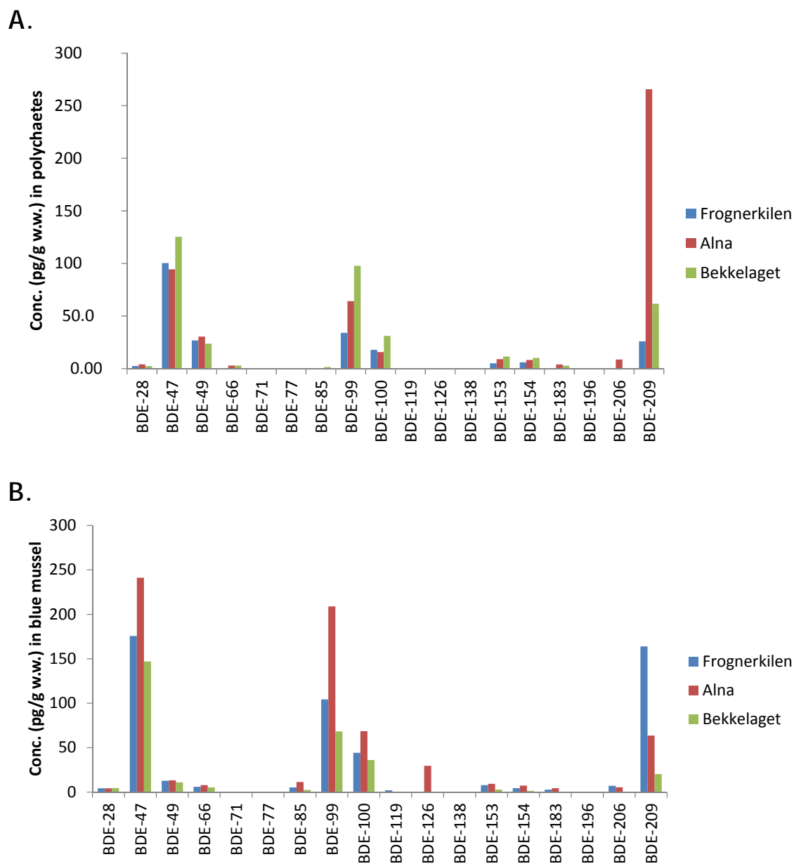
Figure 11. Concentrations of PBDEs (pg/g wet. wt.) in polychaetes (A.) and blue mussel (B.) from Frognerkilen, the mouth of Alna River and at Bekkelaget. One composite sample per station.
