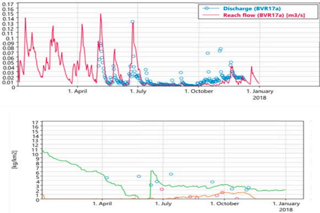
Figure 13. Model application to the Canadian case study. Upper panel shows the fit between modelled (red line) and observed (blue dots) river water discharges (driven in the model by an underlying hydrological module). The lower panel shows predicted (green and red lines) vs observed (blue and red dots, respectively) masses of MPs in the catchment soils over time. (green shows results for soils with applied sludge while red represents control soils).
