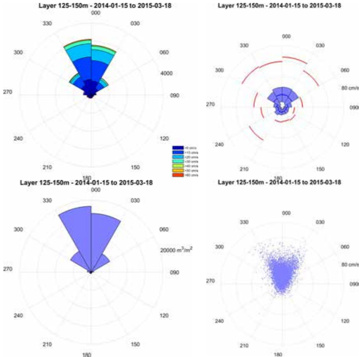
Figure 7 Polar plots of the bottom current during the whole deployment period. Upper left : current histogram by directions sectors. Upper right : blue arcs correspond to the mean current value within the direction sector. Blue areas are standard deviation extending on each side of the mean value. Red arcs are the maximum current value observed. Lower left : estimated transport integrated over the deployment period. Lower right : scatter plot of all observations.
