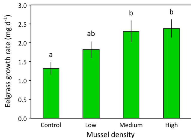
Figure 2. Eelgrass growth rate (mean ± SE) in aquarium experiment with four different mussel densities. Letters indicate significant differences ( p < 0.05 ).
