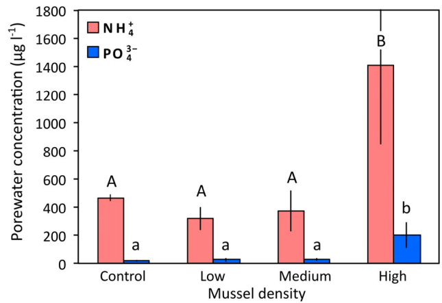
Figure 3. Porewater ammonium (red) and phosphate (blue) concentrations (mean ± SE) in aquaria with four different mussel densities in aquarium experiment. Letters (uppercase: ammonium, lowercase: phosphate) indicate significant differences ( p < 0.05 ).
