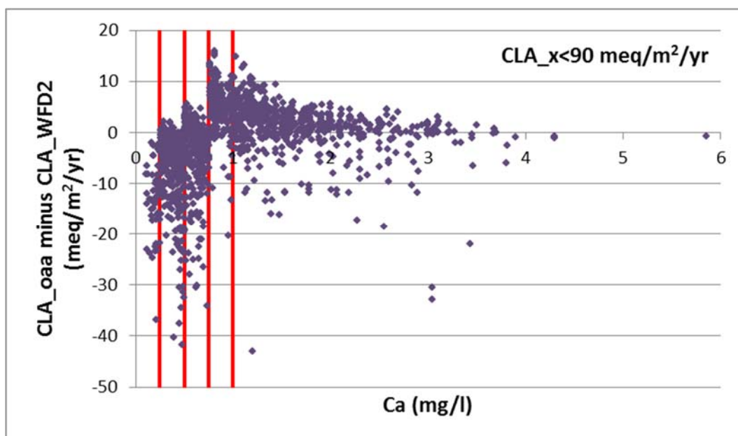
Figure 7. The relationship between the difference between CLA_ooa and CLA_WFD2 and calcium concentration. Only grid values where both CLAs are <90 \text{ meq/m}^2/\text{yr} are included. Calcium category boundaries (WFD) are marked by red vertical lines.
