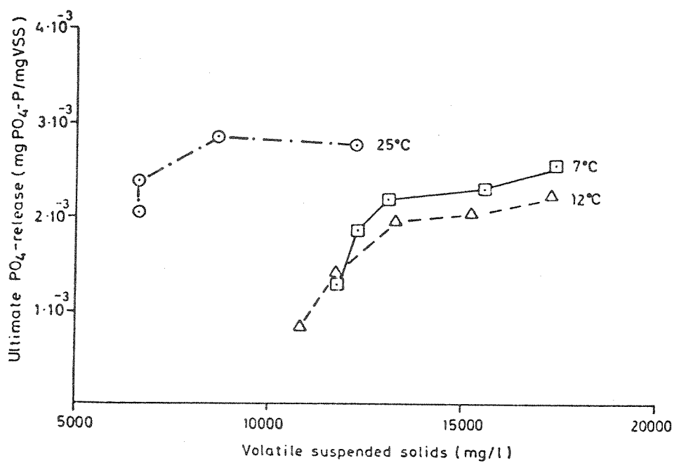
Figure 51. Ultimate Orthophosphate Release vs. Volatile Suspended Solids Concentration - Primary Sludge.
