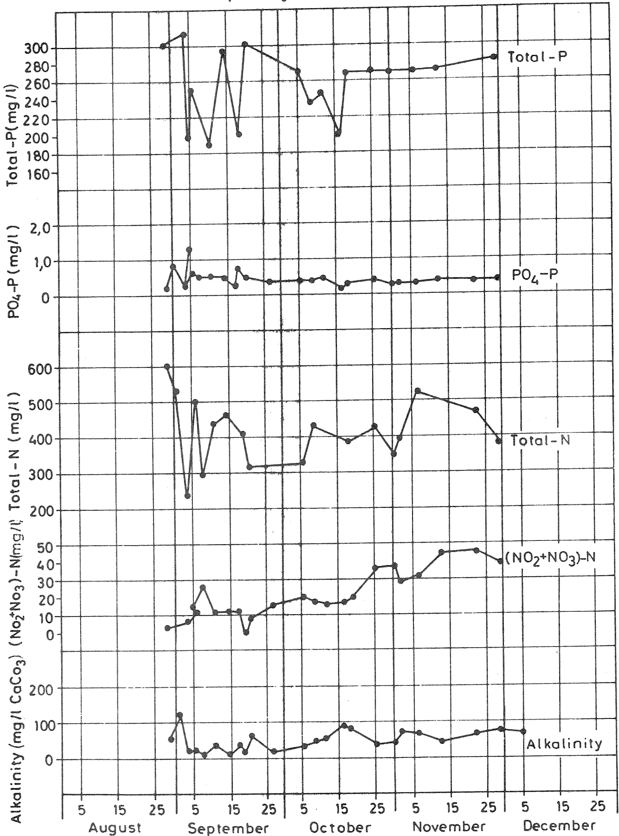
Figure 65. Digested Mixed Primary-Chemical Sludge vs. Time.
