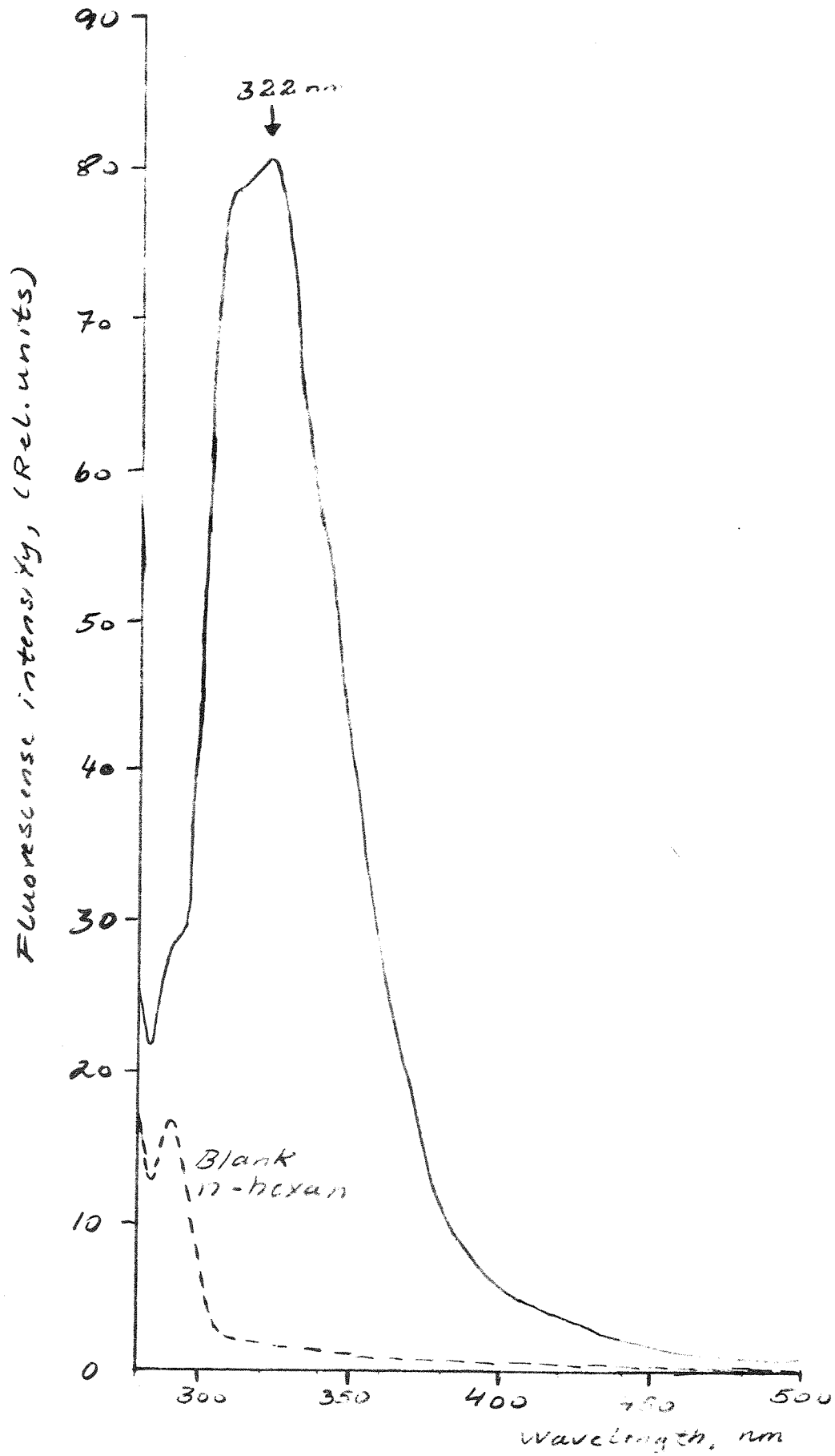
Figure 1 Fluorescence emission spectra of a diesel oil standard (1.74 µg/ml) in n-hexane.
