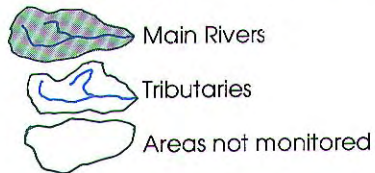
Fig. I.IV Main Rivers and Tributaries draining to The Barents Sea.
