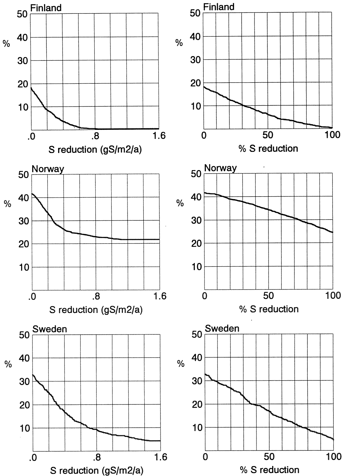
Figure 4. Inverse cumulative distribution functions for each country showing the reductions required for S deposition in absolute deposition units (left) and in percentages from present deposition (right), for the N deposition fixed at present level.
