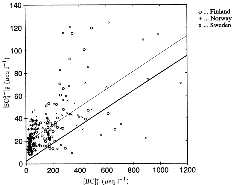
Figure 2. Background sulfate concentration as a function of base cation concentration. The thin line shows the regression equation (Eq.32) and the thick line the regression minus one standard deviation used for computing the background sulfate concentration.
