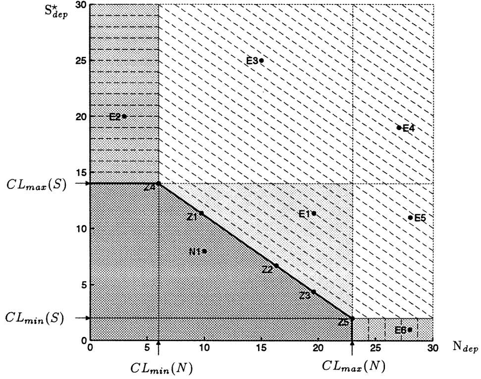
Figure 1. The relationships between the N and S depositions and critical loads. The case for the non-exceedance ( N1 ) and the six cases for exceedance ( E1 - E6 ) as well as the five cases for critical load ( Z1 - Z5 ) are described in the text.
