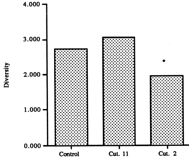
Fig. 68. Mean diversity (Shannon-Wiener) in boxes with different treatments. Please note that diversity shown for Cut. 11 and 2 are mean values based on diversity for 3 individual boxes whereas diversity in control are based on one box (box no. 3). * above column indicate significant difference from Cut. 11.
