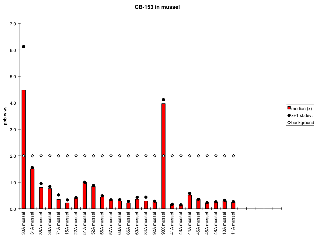
Figure 28. Median, standard deviation and provisional "high background" concentration for CB-153 in mussels ( Mytilus edulis ) 1994 ( A ) and 1995 ( B ), ppb wet weight (see maps in Figure 12-Figure 15).
