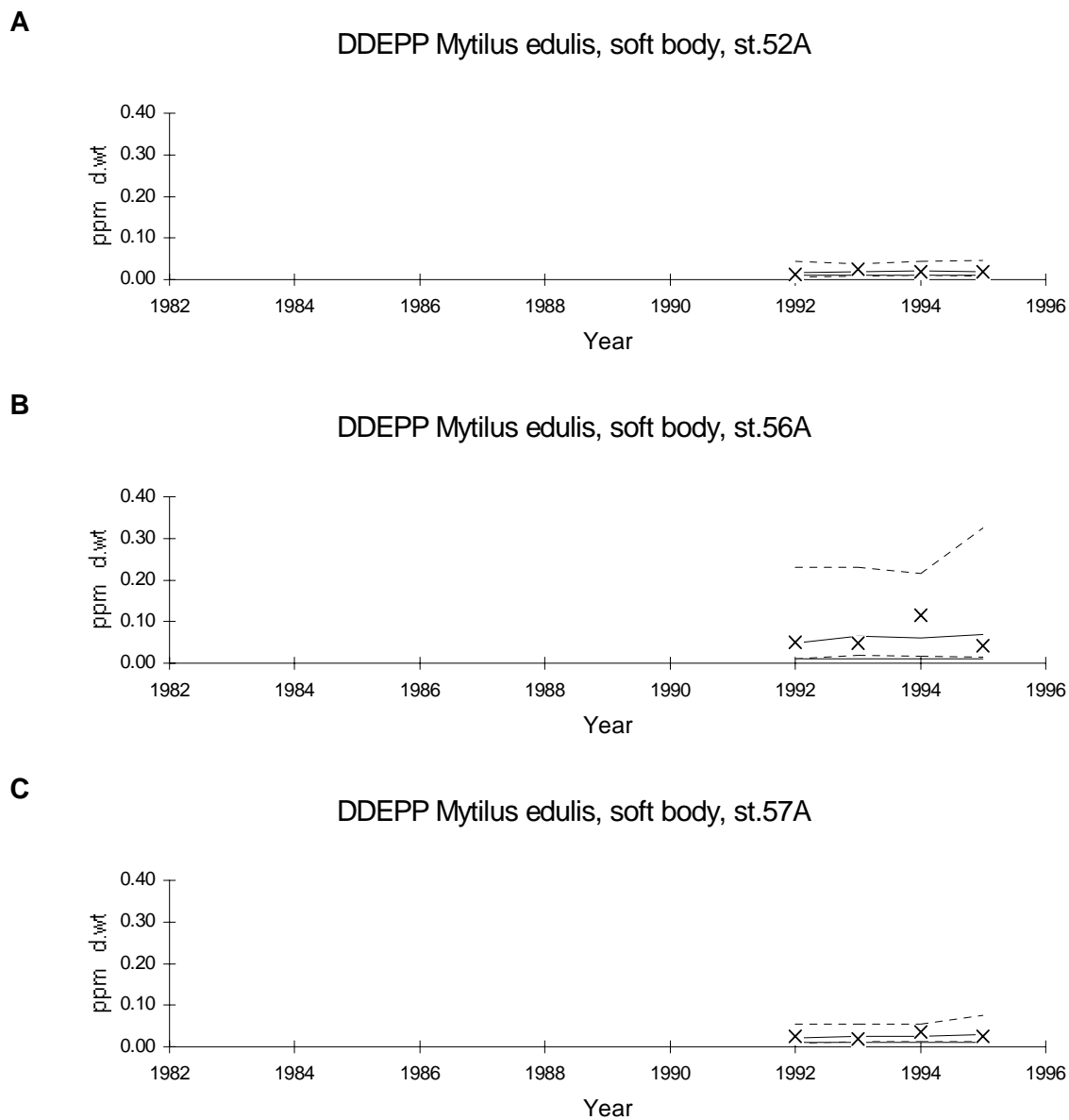
Figure 9. Median ppDDE (DDEPP) concentration in blue mussel ( Mytilus edulis ) from inner (st.52) to outer (st.57) Sørffjord. (cf., Figure 1 and Figure 12).
