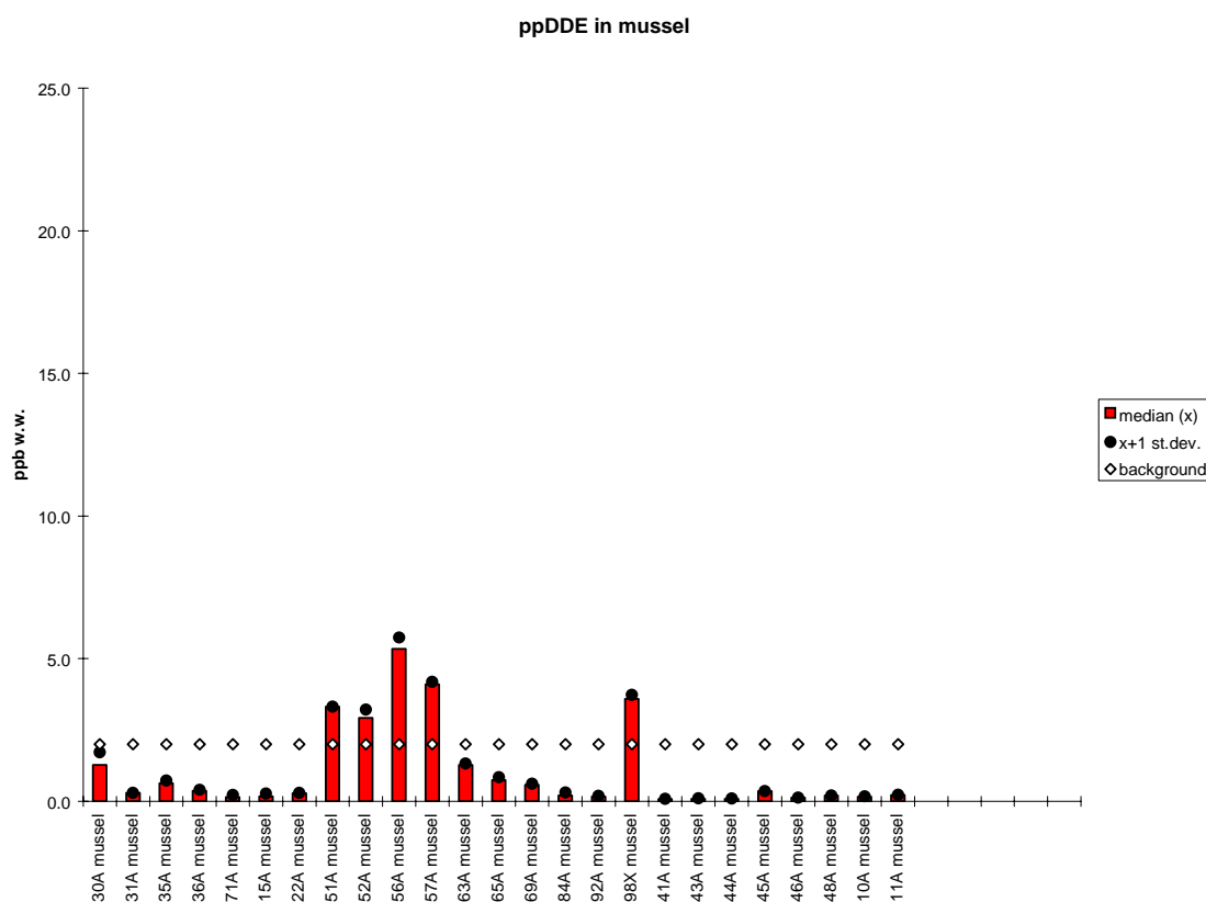
Figure 30. Median, standard deviation and provisional "high background" concentration for ppDDE (DDEPP) in mussels ( Mytilus edulis ) 1994 (A) and 1995 (B), ppb wet weight (see maps in Figure 12- Figure 15). (See also footnote in Table 1.)
