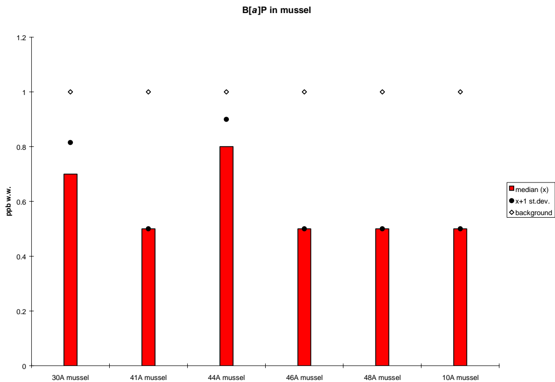
Figure 36. Median, standard deviation and provisional "high background" concentration for B[a]P (BAP) in mussels 1995 ( A ) and 1996 ( B ) ppb wet weight (see maps in Figure 1 and Figure 4).
