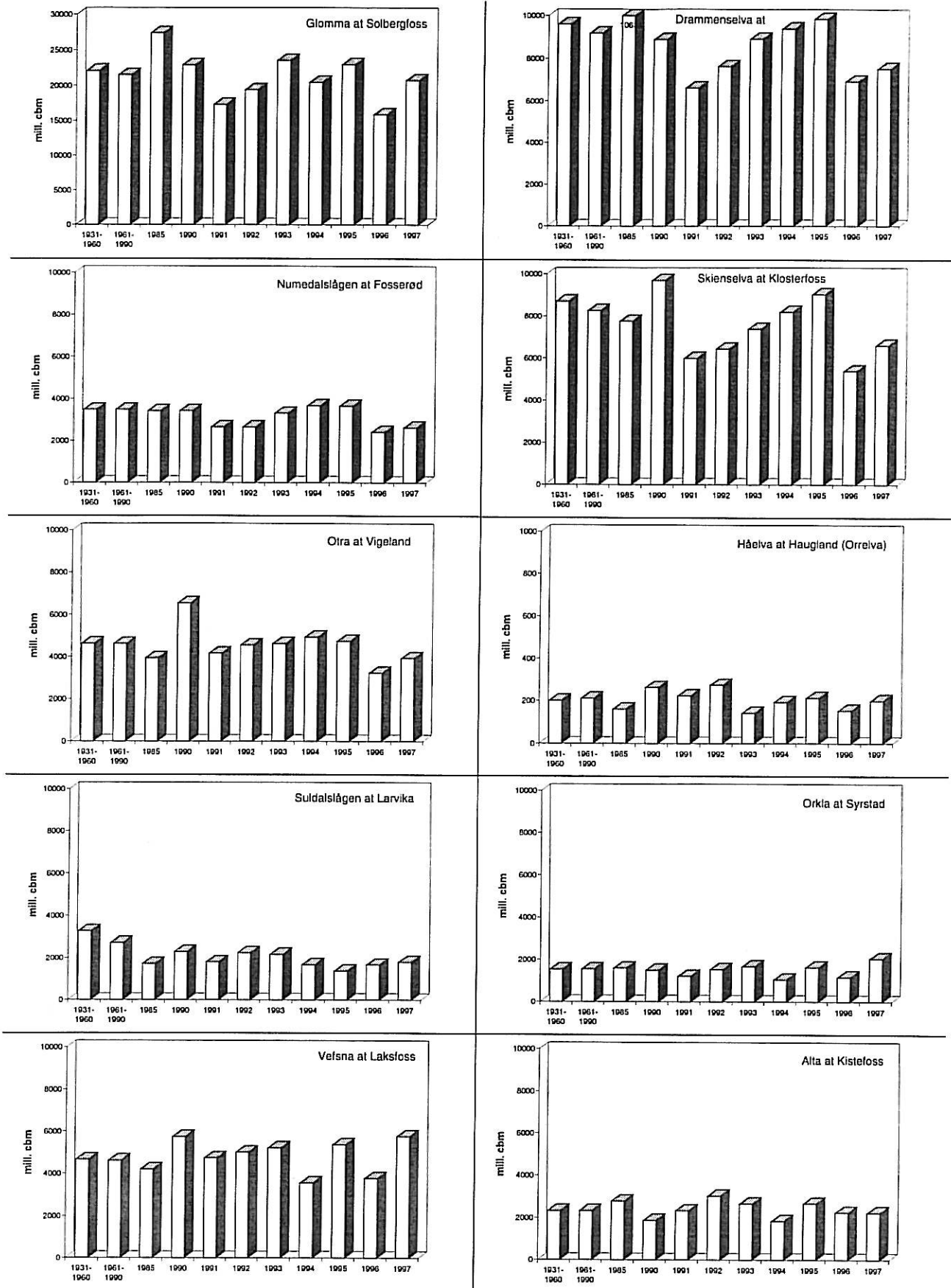
Fig. 2 Main Rivers. Mean Annual Runoff (1931-60 and 1961-90) and Annual Runoff for the Years 1985, 1990-1997 (mill. cbm.). Source: Norwegian Water Resources and Energy Administration
