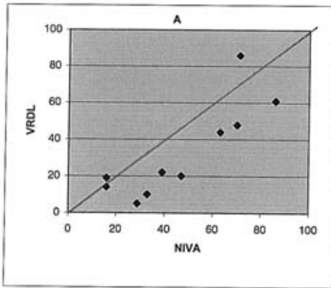
Figure A3.9. Phosphate-phosphorous, \mu\text{g/l}
