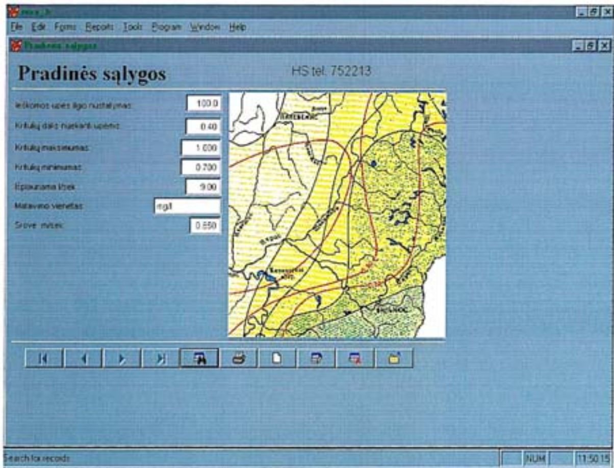
Figure 5.8. Window for input of preliminary factors in the TEOTIL model.
