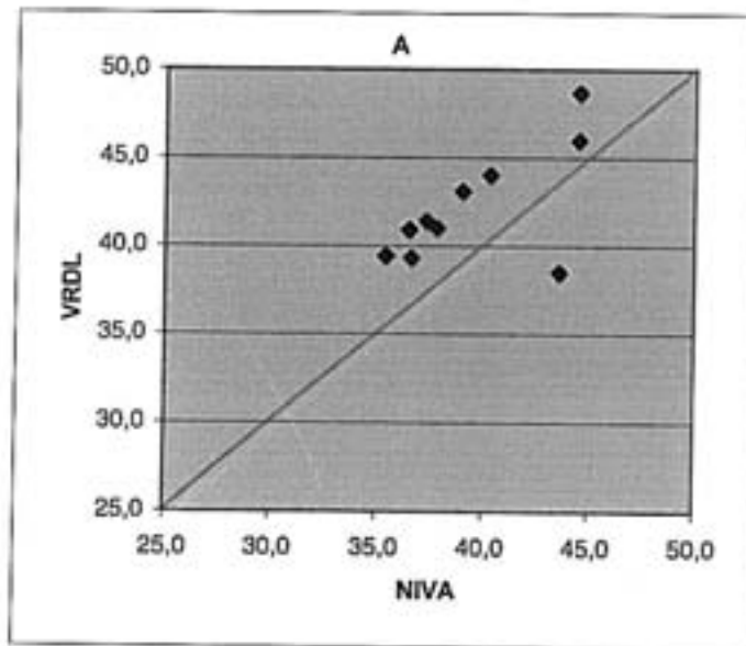
Figure A3.2. Conductivity, mS/m at 25 °C
