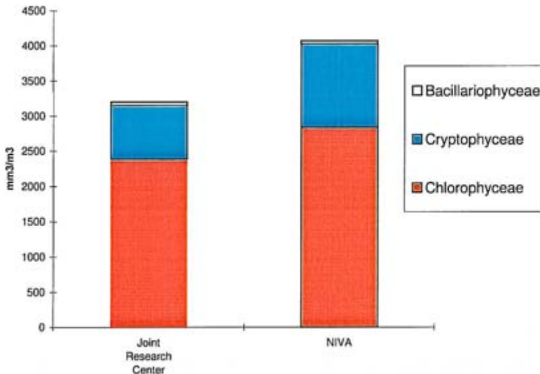
Figure 4.3 Calculated volumes of the main groups of phytoplankton in the sample from Bebruko Lake 3 rd September 1996. The Joint Research Centre and NIVA made the calculations separately.
