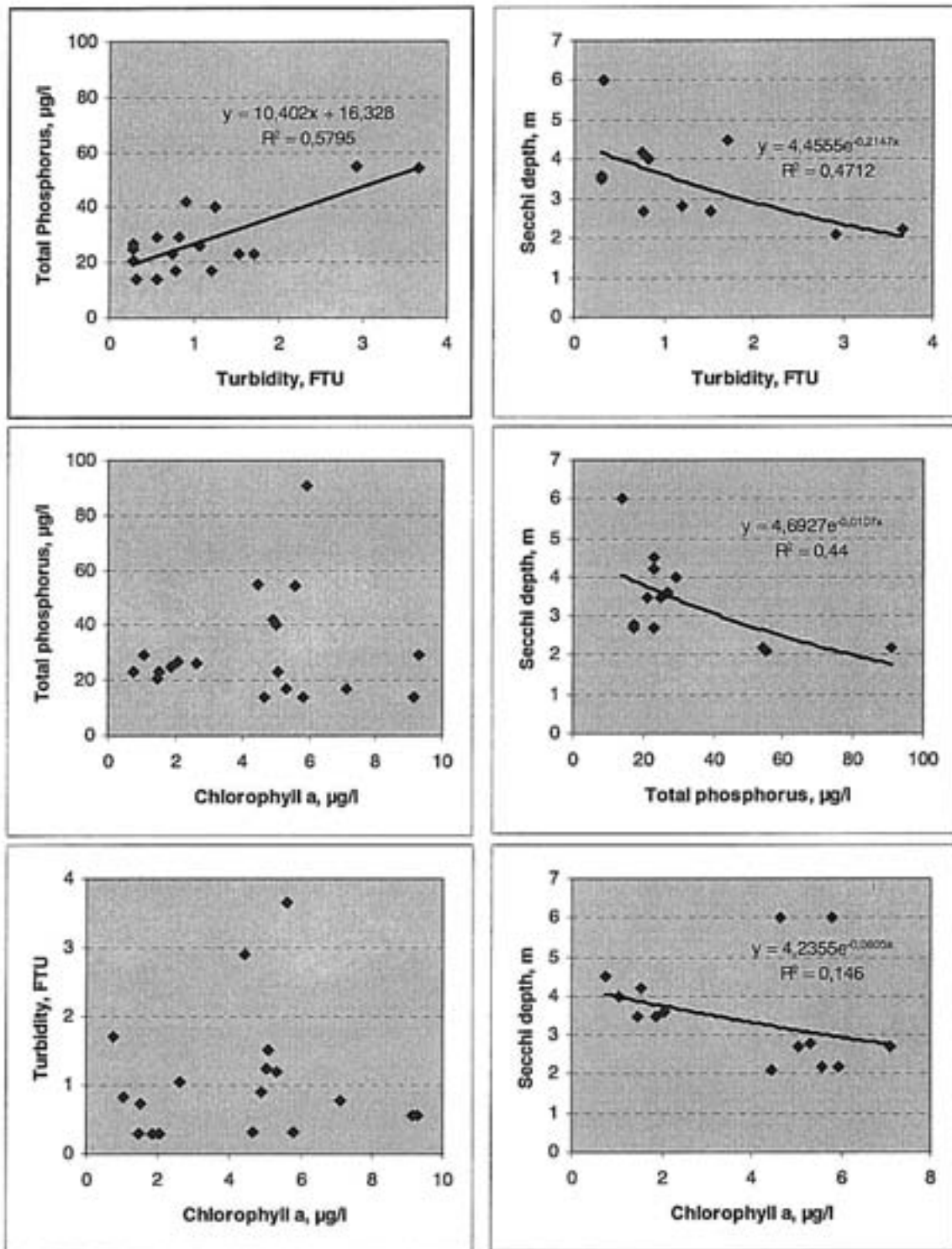
Figure 3.2. Correlation between lake monitoring parameters from 6 lakes in May/June 1998.
