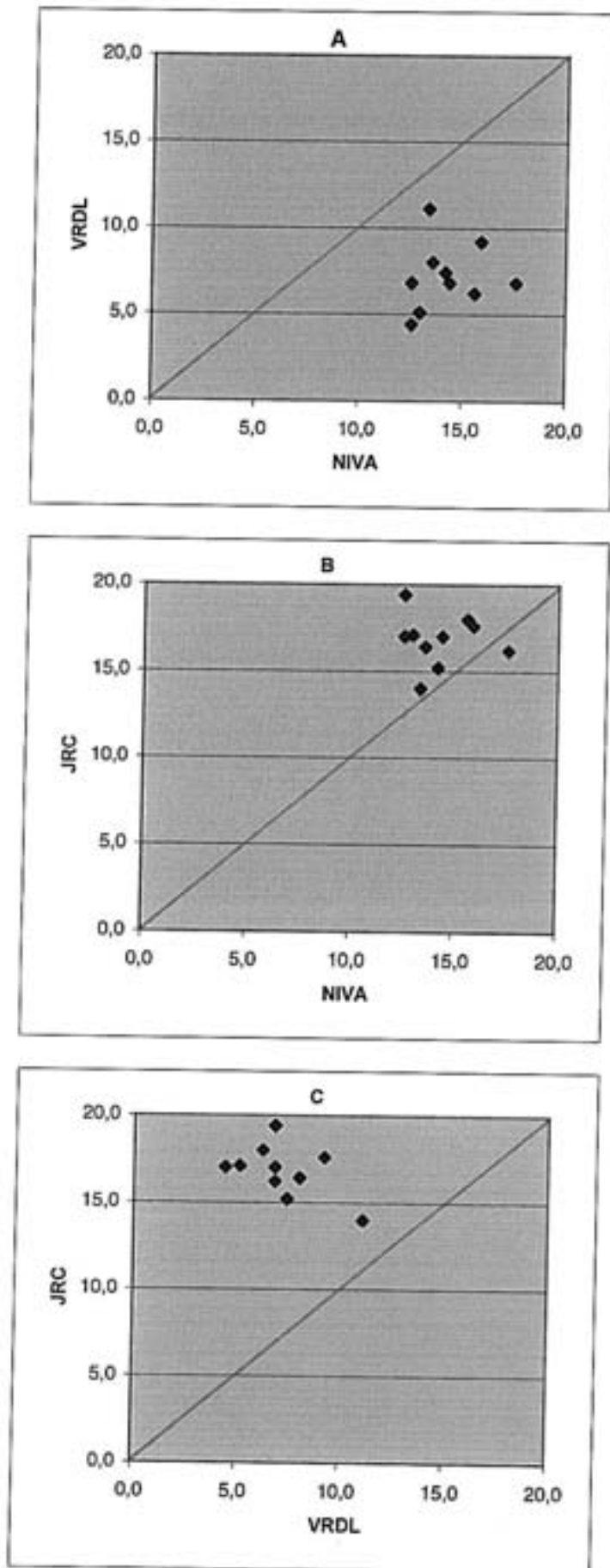
Figure A3.14. Magnesium, mg/l
