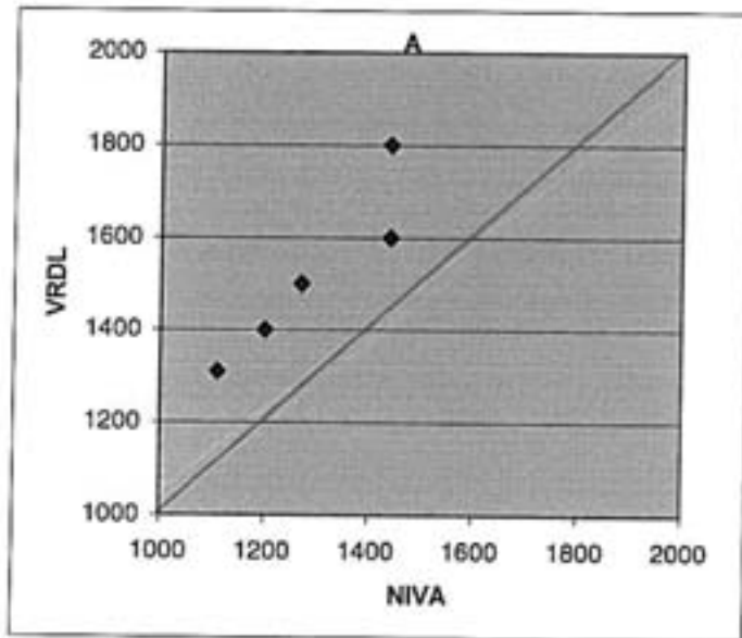
FigureA3. 7. Total nitrogen, \mu\text{g/l}
