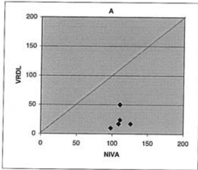
Figure A3.5. Ammonium-nitrogen, \mu\text{g/l}
