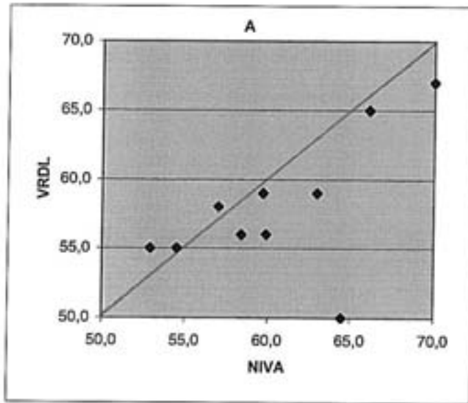
Figure A3.13. Calcium, mg/l
