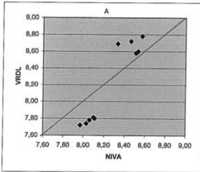
Figure A3.1. pH
