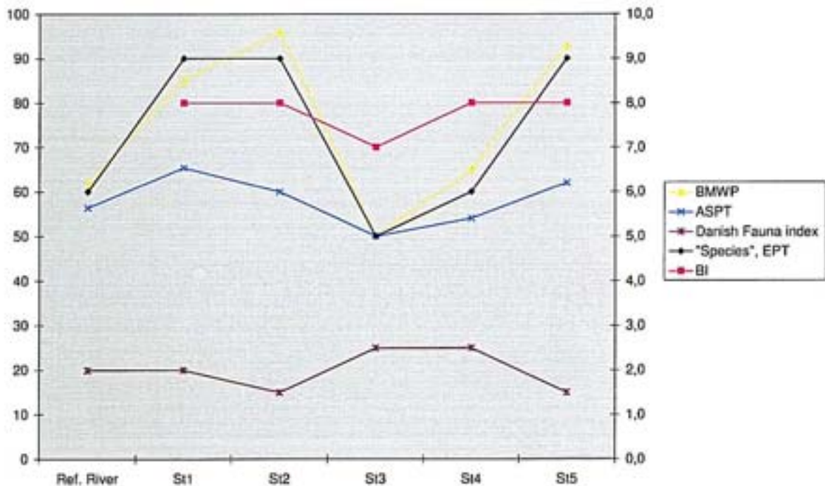
Figure 4.2 . Different macroinvertebrate indexes based on the material from the Neris river. The numbers are index values. BMWP on the left axis. Other indexes on the right axis.
