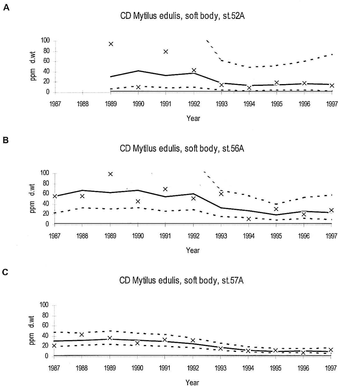
Figure 9. Median cadmium (Cd) concentration in blue mussel ( Mytilus edulis ) from inner (st.52A) to outer (st.57A) Sør fjord. NB: (cf., Figure 1 and Figure 26). Note: for some years the upper confidence interval line is off-scale in figures A and B.
