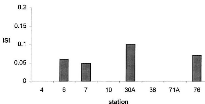
Figure 21. Intersex (ISI) in Littorina littorea at eight locations in southern Norway in 1997.
