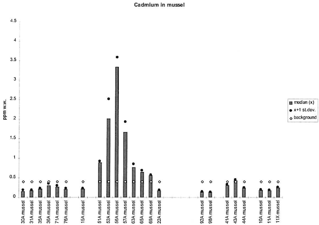
Figure 27. Median, standard deviation and provisional "high background" concentration for cadmium in mussels ( Mytilus edulis ) 1996 (A) and 1997 (B), ppm wet weight (see maps in Figure 1- Figure 4).
