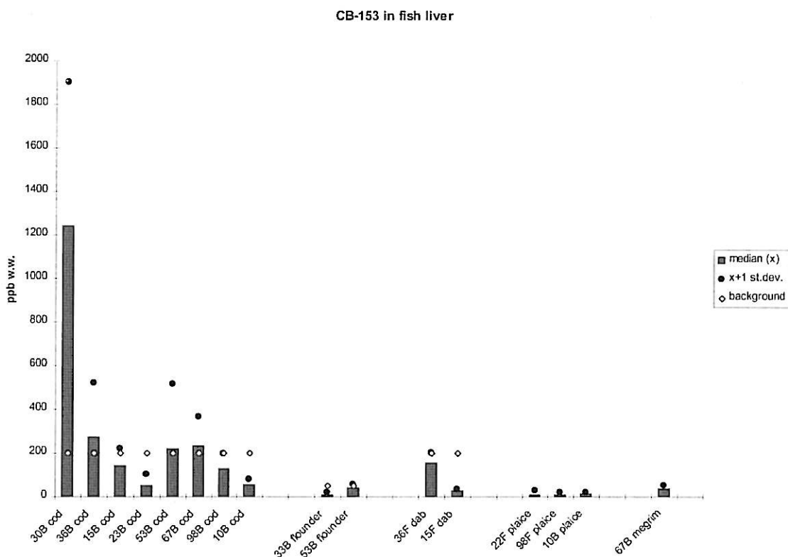
Figure 40. Median, standard deviation and provisional "high background" concentration for CB-153 in fish liver 1996 (A) and 1997 (B), ppb wet weight (see maps in Figure 1-Figure 4).
