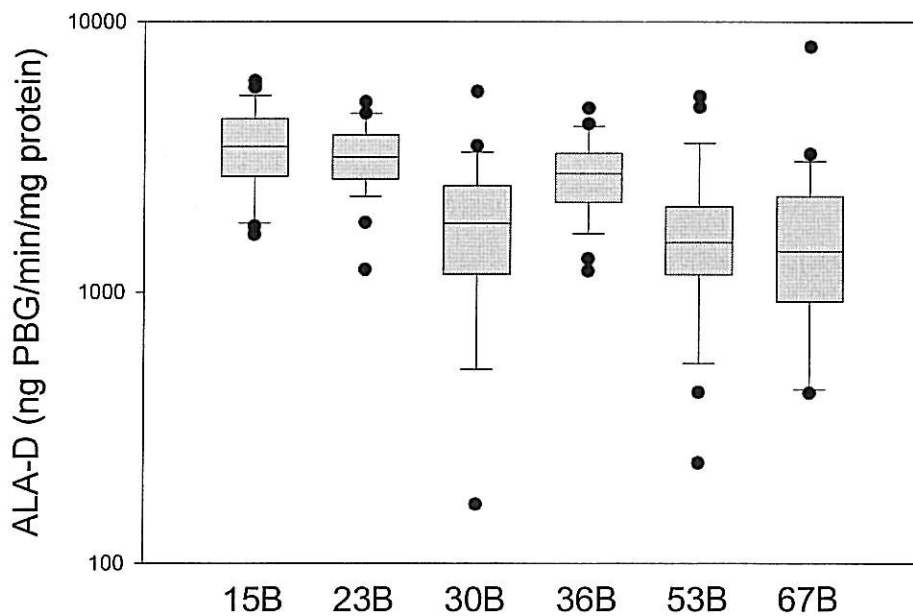
Figure 16. Activity of ALA-D in blood cells of cod sampled at the indicated sites. Median, quartiles, 10/90-percentiles and outliers are indicated. (One low outlier not shown for st.30B, see also Figure 1, Appendix J Table 11.)
