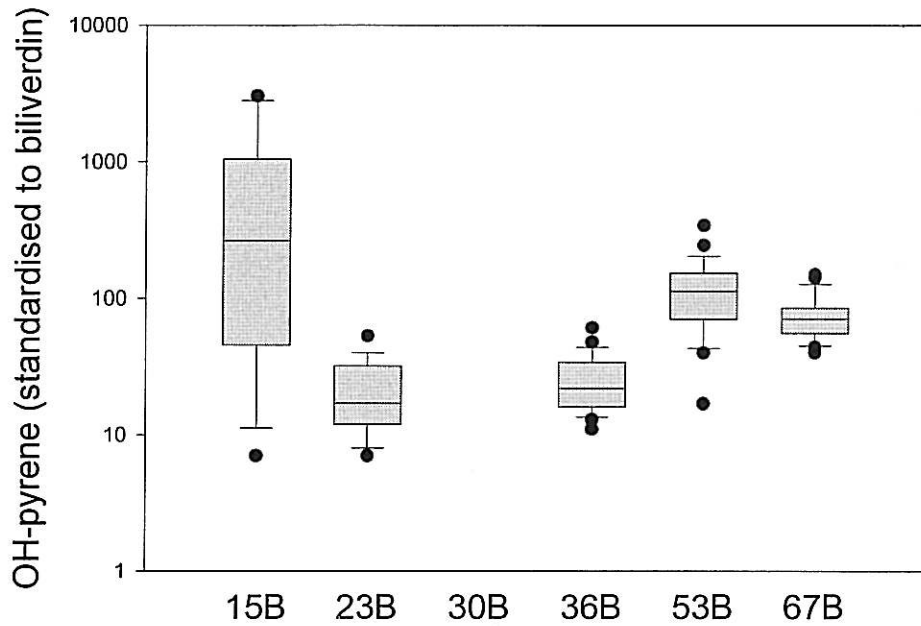
Figure 15. Concentrations of OH-pyrene in bile of cod sampled at the indicated sites. Median, quartiles, 10/90-percentiles and outliers are indicated. (See also Figure 1, Appendix J Table 10.)
