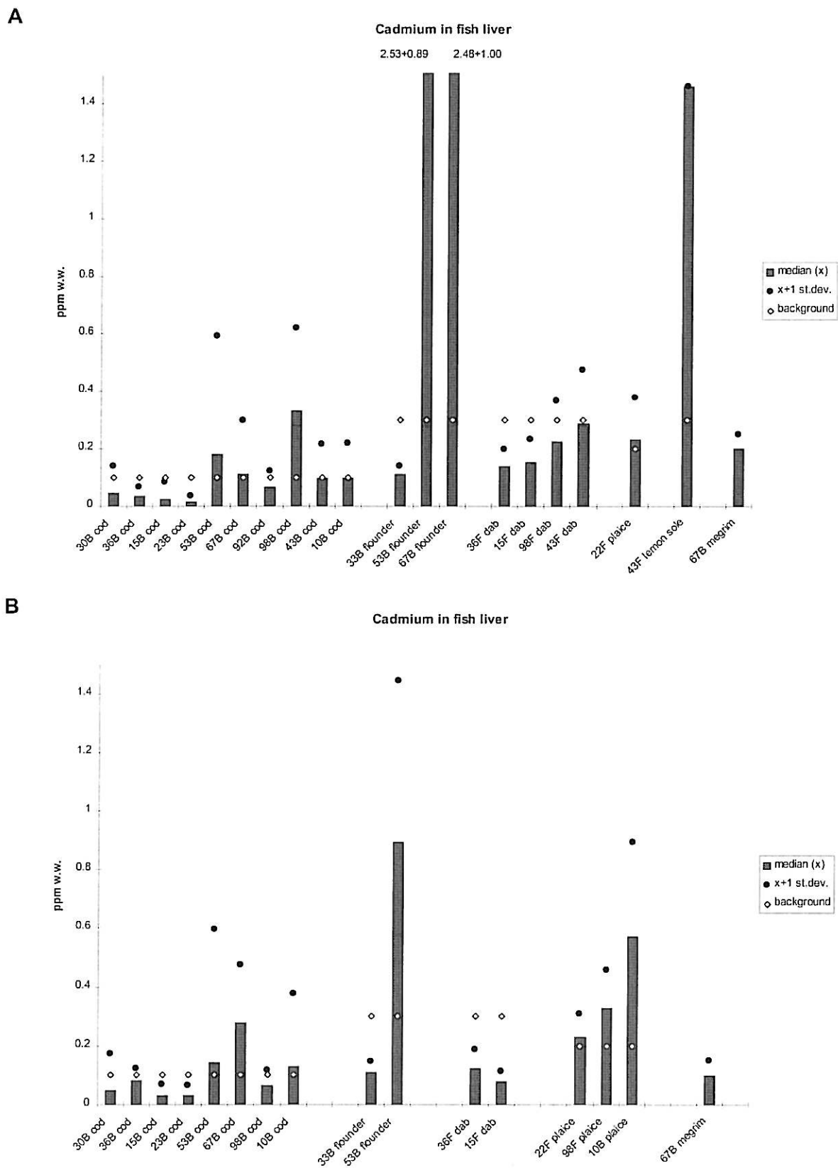
Figure 28. Median, standard deviation and provisional "high background" concentration for cadmium in fish liver 1996 (A) and 1997 (B), ppm wet weight (see maps in Figure 1-Figure 4).
