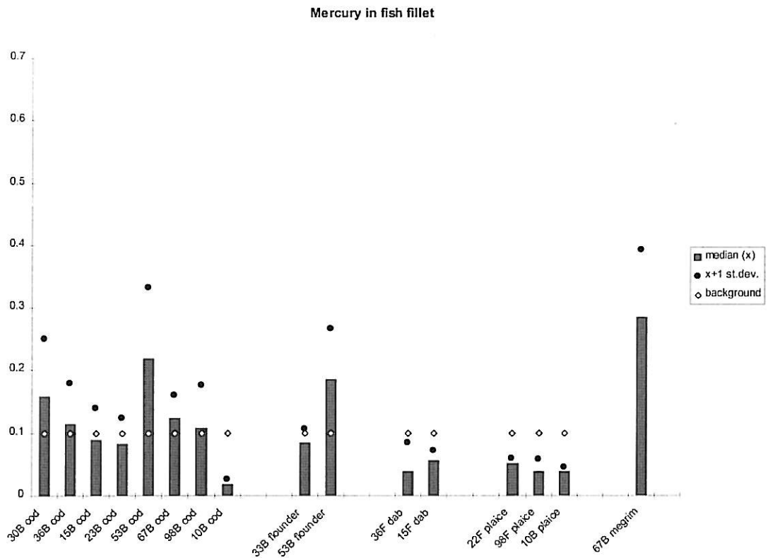
Figure 32. Median, standard deviation and provisional "high background" concentration for mercury in fish fillet 1996 (A) and 1997 (B), ppm wet weight (see maps in Figure 1-Figure 4).
