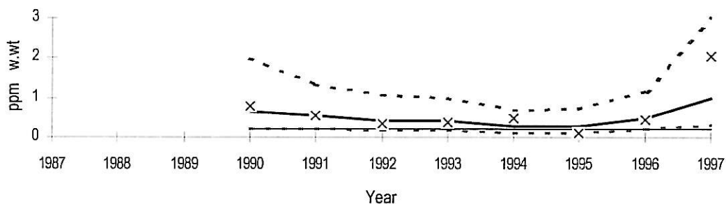
Figure 13. Median ppDDE (DDEPP) concentrations in cod ( Gadus morhua ) from Sørfjord (st.53B) and Hardangerfjord (st.67B) (cf., Figure 1 and Figure 26). Note that for some years the upper confidence interval line is off-scale in Figures A and B.
