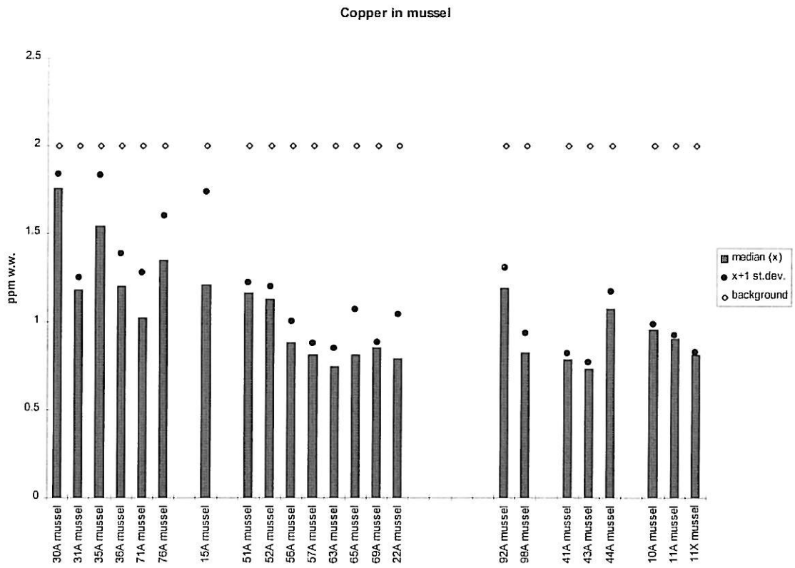
Figure 29. Median standard deviation and provisional "high background" concentration for copper in mussels ( Mytilus edulis ) 1996 (A) and 1997 (B), ppm wet weight (see maps in Figure 1-Figure 4).
