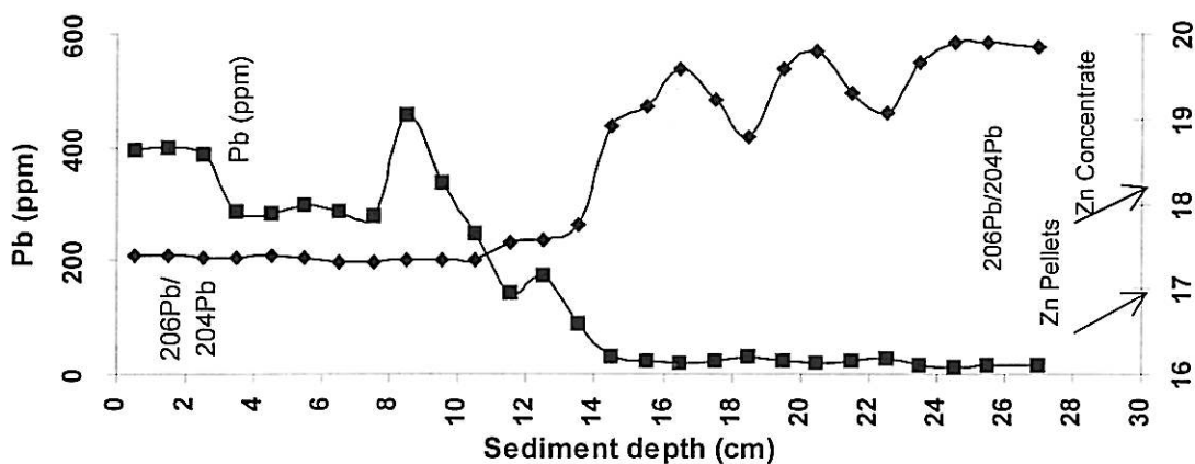
Figure 22. Lead (Pb ppm) and 206 Pb/ 204 Pb ratio in a sediment core (st. 52S, about 10 km from Odda, Figure 1) from the Sør fjord. The isotope ratio in zinc concentrate and pellets are marked with arrows.
