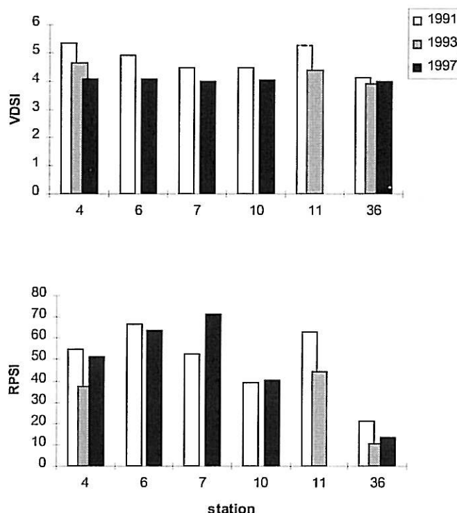
Figure 20. Imposex (VDSI and RPSI) in Nucella lapillus at 6 stations in southern Norway in 1991 (Harding et al. 1992), 1993 (Walday et al. 1997) and 1997. (See maps Figure 1 and Figure 19.)
