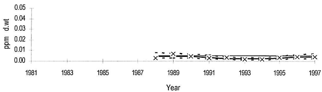
Figure 5. Median CB153 concentration in blue mussel ( Mytilus edulis ) from inner (st.30A) to outer (st.36A) Oslofjord. (cf., Figure 1 and Figure 26).
