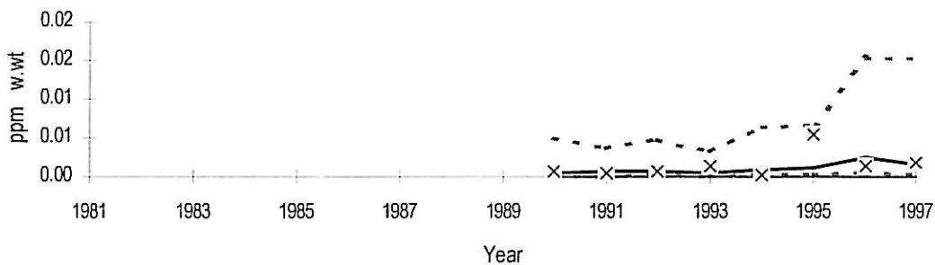
Figure 6. Median CB-153 concentration in liver and fillet of cod ( Gadus morhua ) from the inner (st.30B) to outer (st.36B) Oslofjord. (cf., Figure 1 and Figure 26). Note: for some years the upper confidence interval line is off-scale in Figure D.
