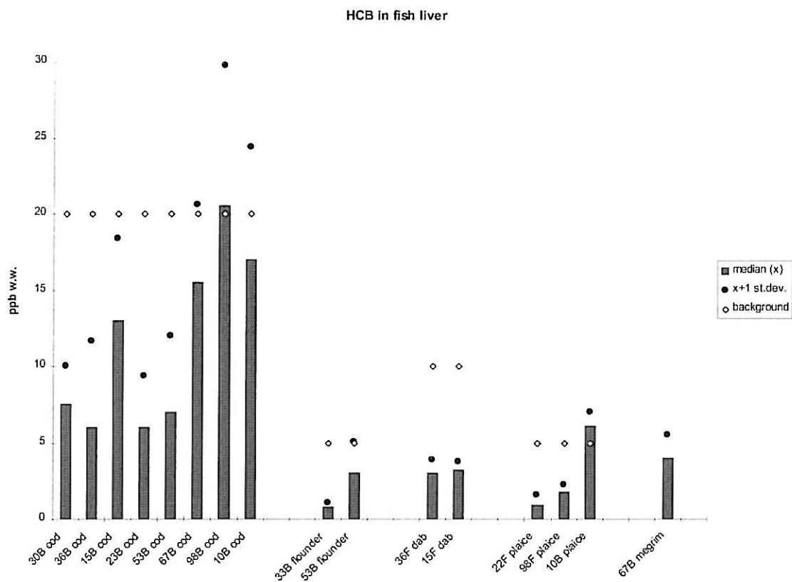
Figure 46. Median, standard deviation and provisional "high background" concentration for HCB in fish liver 1996 (A) and 1997 (B), ppb wet weight (see maps in Figure 1-Figure 4).
