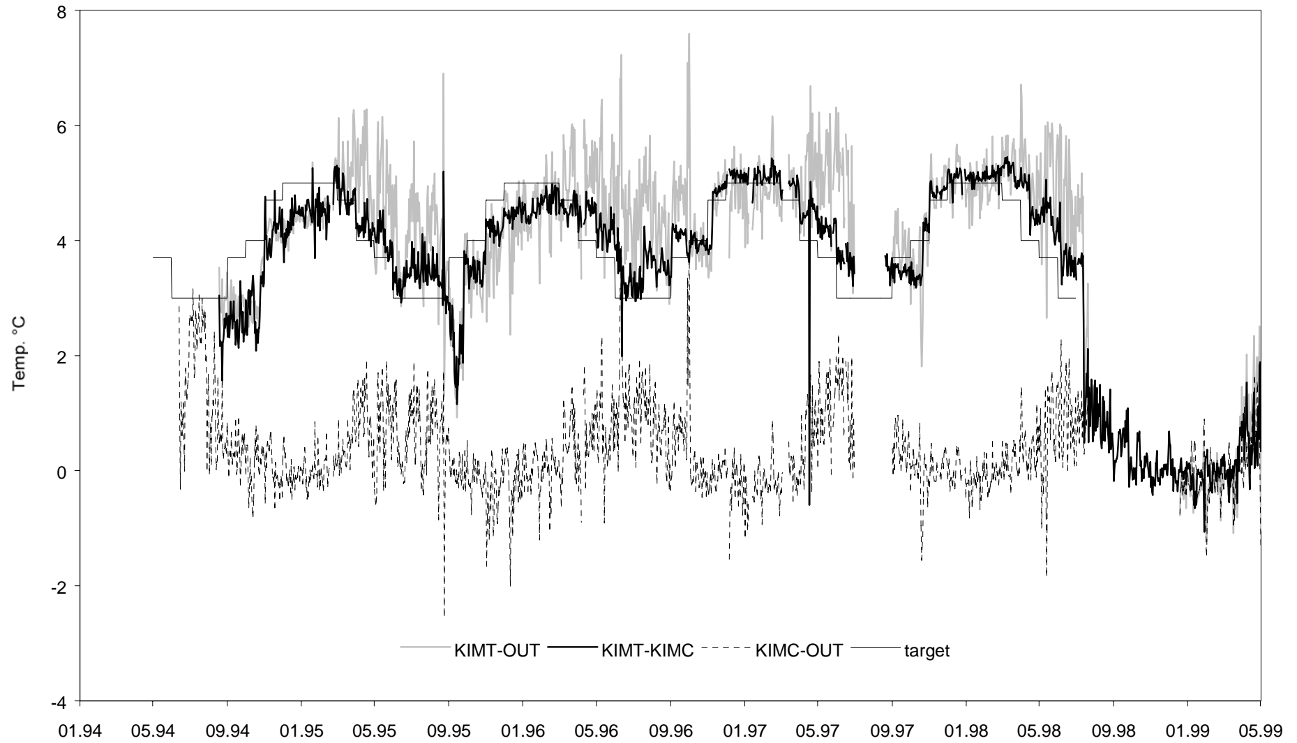
Delta Air Temperature °C, 1994-1999 (DGT)
