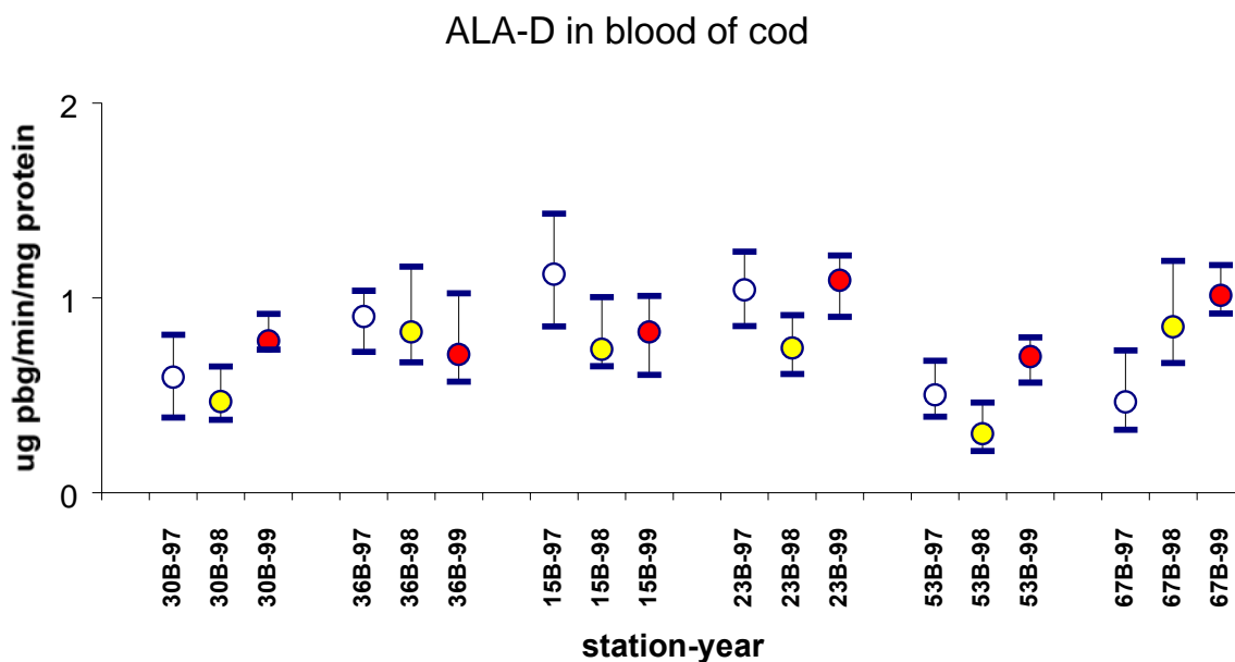
Figure 13. Activity of \delta -aminolevulinic acid dehydratase (ALA-D, \mu\text{g pbg/min/mg protein} ) in red blood cells from Atlantic cod collected at the indicated stations from 1997 to 1999. Median and quartiles (25%, 75%).
