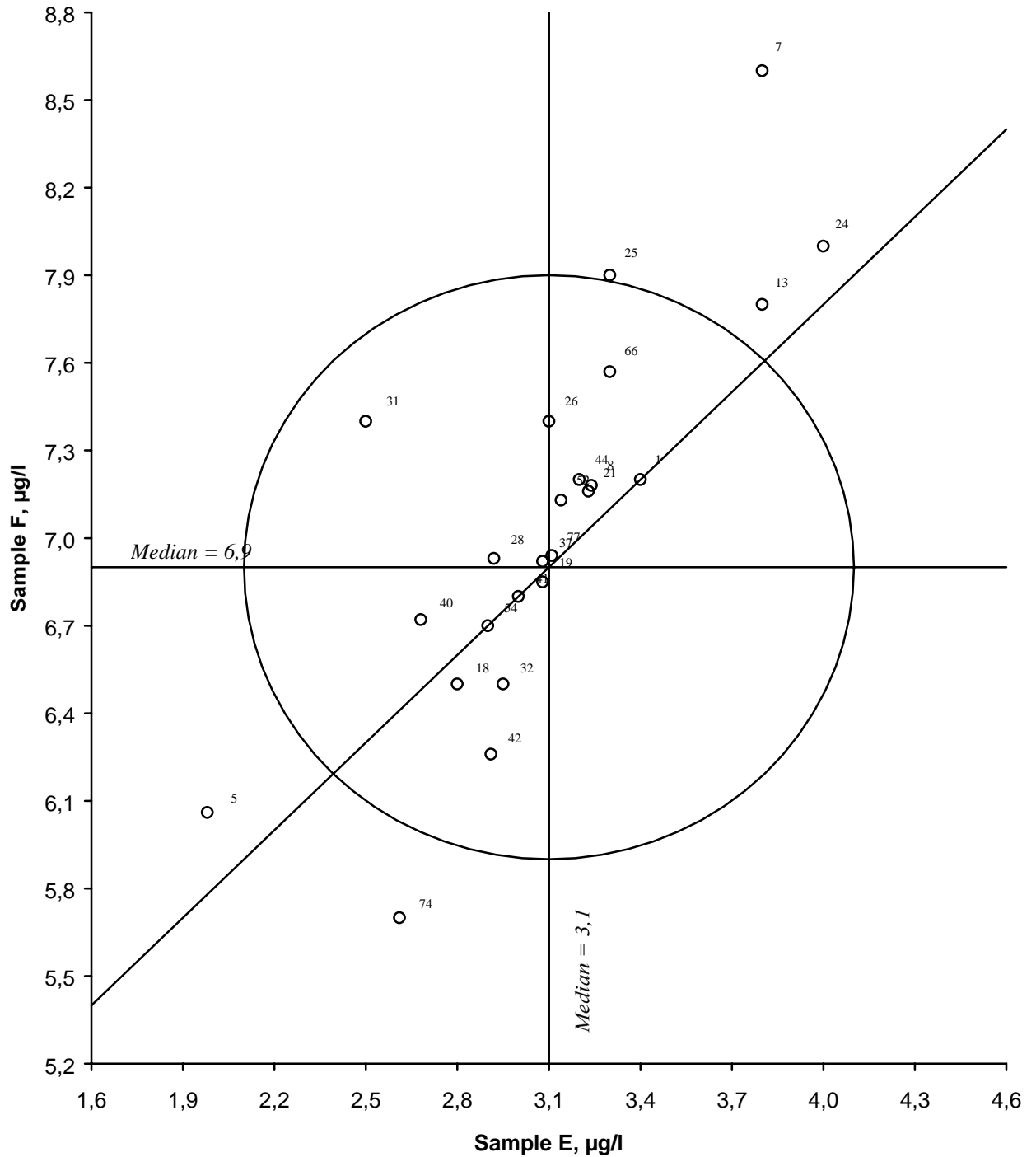
Figure 20. Youdendiagramme for lead, sample pair EF. Acceptance limit given by the circle is 20 %.
