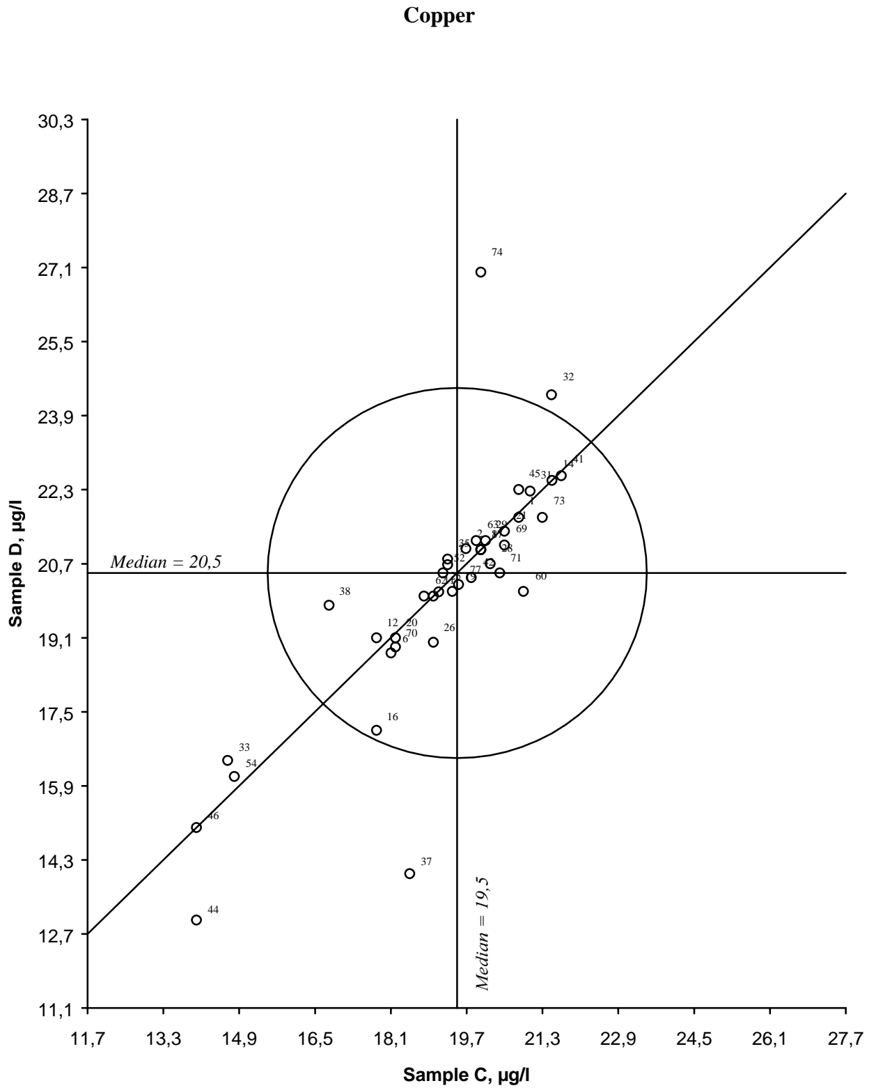
Figure 15. Youden diagramme for copper, sample pair CD Acceptance limit, given by the circle, is 20 %
