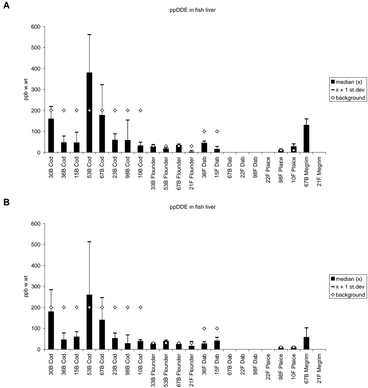
Figure 32. Median, standard deviation and provisional "high background" concentration for ppDDE (DDEPP) in fish liver 2000 (A) and 2001 (B), ppb wet weight (see maps in Appendix F). (See also footnote in Table 7).
