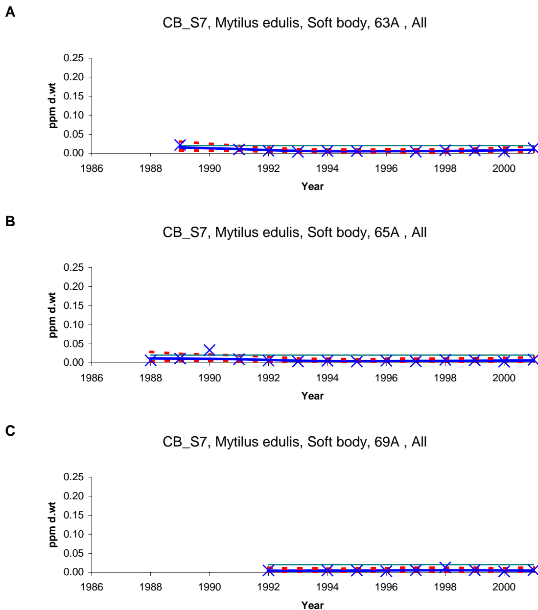
Figure 13. Median CB_S7 (=ΣPCB-7) concentrations in blue mussel ( Mytilus edulis ) from Hardangerfjord (st. 63A, 65A and 69A). (cf. Appendix F and key in Figure 22). Note: horizontal line for "high background" near x-axis.
