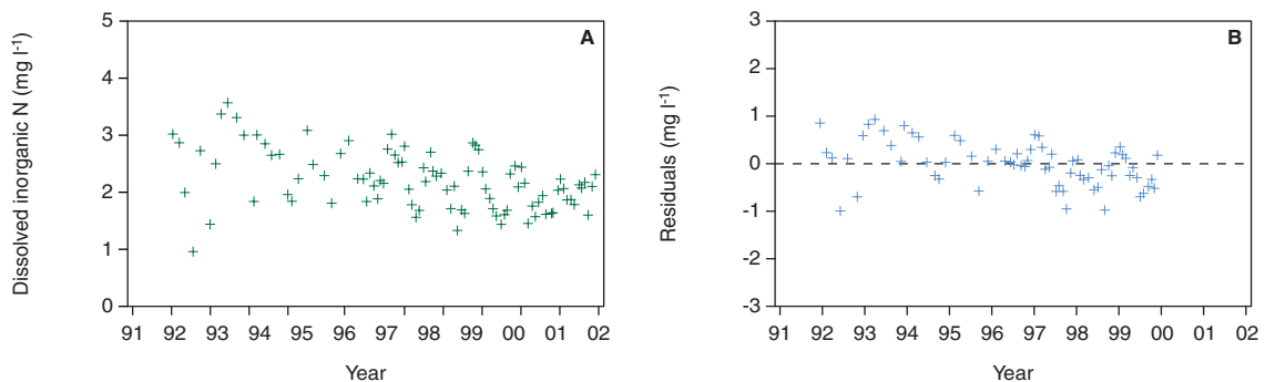
Figure 9: Time series of concentrations of dissolved inorganic N and the flow-adjusted concentrations (residuals) during the period 1992-2001. Average concentration of total nitrogen is 2.25 \text{ mg l}^{-1} ( CV=14\% ).
