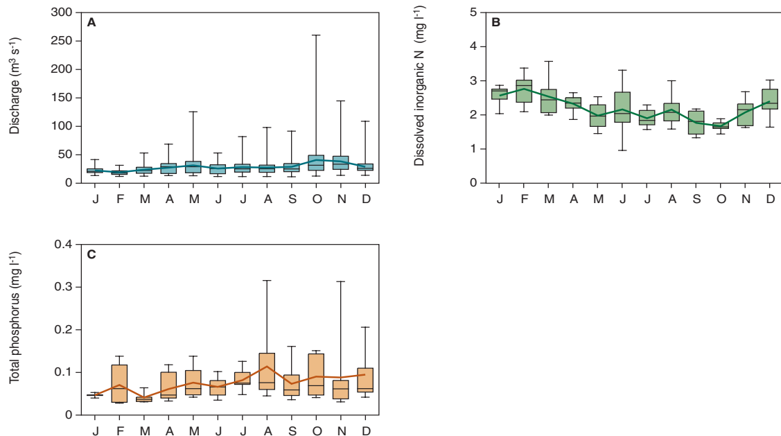
Figure 8: Box-Whisker plots showing the variation in runoff, and dissolved inorganic nitrogen and total phosphorus concentrations in the catchment.
