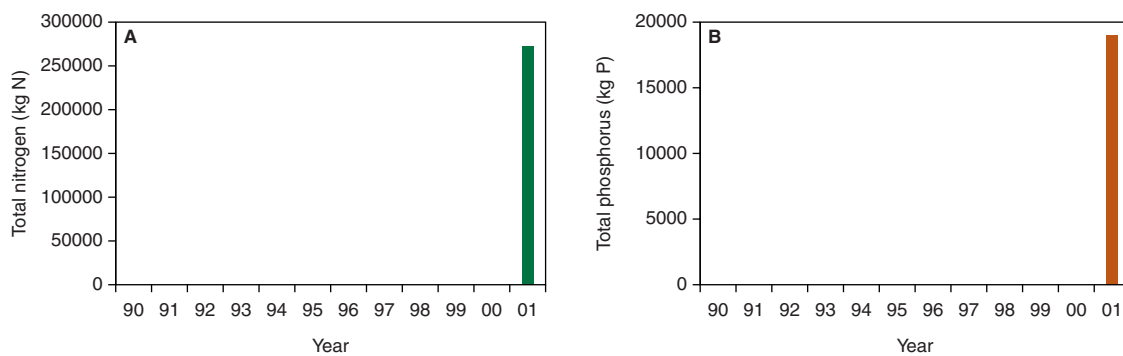
Figure 4: Annual discharge of total nitrogen and total phosphorus from WWTPs in the Gurk catchment.
