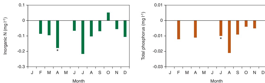
Figure 12: Monthly trend calculated on an annual basis in the concentration of dissolved inorganic nitrogen and total phosphorus during the period 1992-1999. (*Significant at P=5\% ). Months are missing due to absence of monitoring data during the time period tested.
