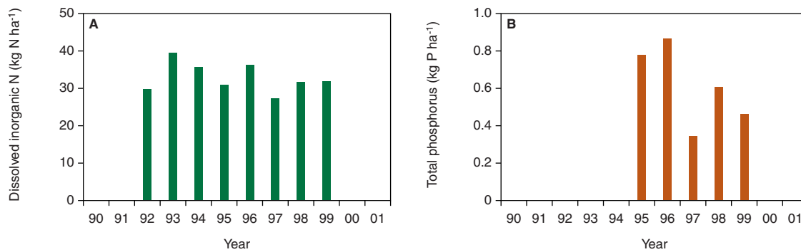
Figure 7: Annual diffuse losses of dissolved inorganic nitrogen and total phosphorus from agricultural land within the catchment.
