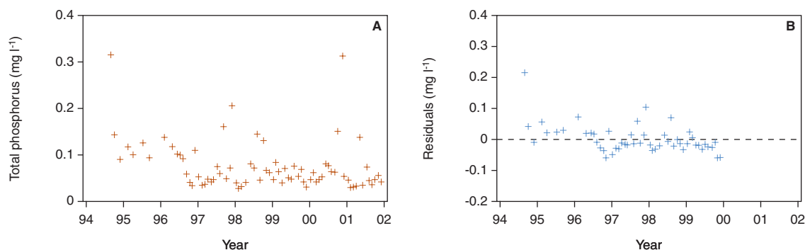
Figure 10: Time-series of flow-adjusted concentrations of total phosphorus and the flow-adjusted concentrations (residuals) during the period 1994-2001. The average concentration of total phosphorus is 0.071 mg l -1 (CV=22%).
