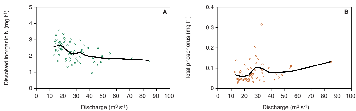
Figure 13: Relationships between discharge and concentrations of dissolved inorganic nitrogen and total phosphorus, established applying the LOWESS fitting procedure (see Annex 3).
